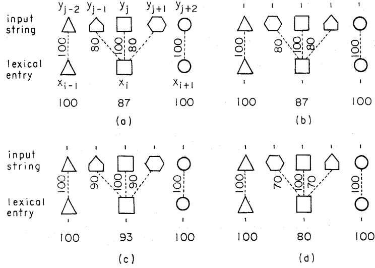
Fig. 5. Graphic model of normalization of coarticulation. (a) and (b): before normalization, (c) and (d): after normalization. Where, we assume that S(\triangle, \wedge) = S(\bigcirc, \vee) = 80 , S(\triangle, \square) = S(\bigcirc, \square) = 60 , S(\triangle, \bigcirc) = 40 , k = 0.5 .
