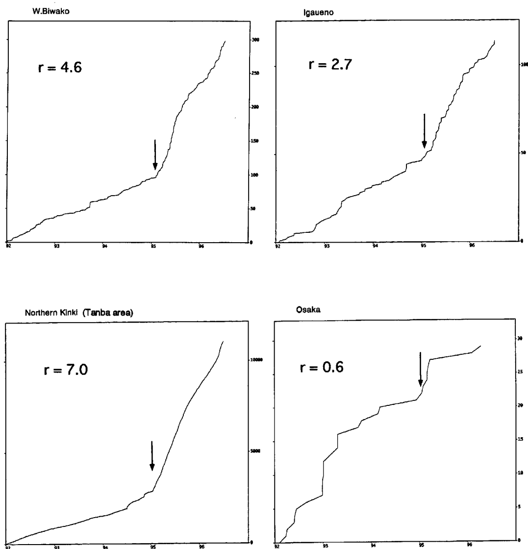
Fig. 13 Changes of seismicity rates. r = seismicity rate (post-mainshock)/seismicity rate (pre-mainshock)
