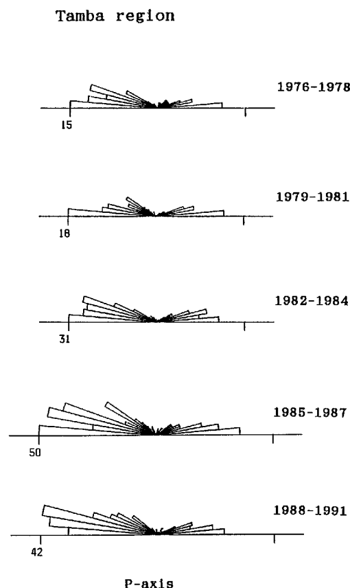
Fig. 9 Temporal variation of rose diagrams of P axes for the activity in the Tanba mountain area. In 1988-1991, the diagram rotated clockwise about 10^\circ .
