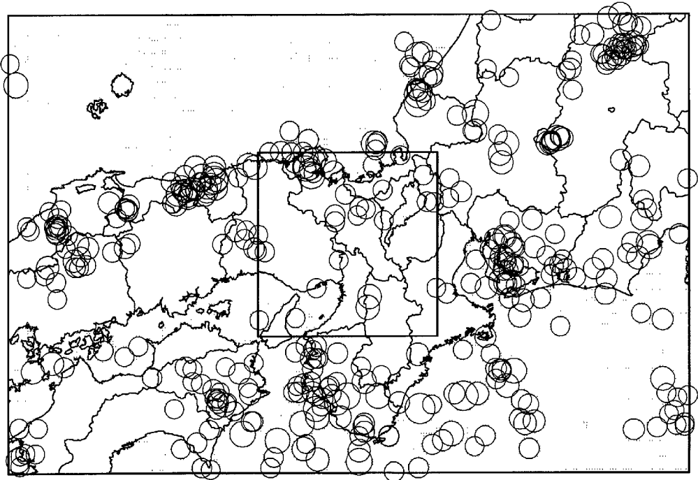
Fig. 3 Epicentral distribution of major earthquakes of M > 5 , determined by JMA during 1926~1994.
