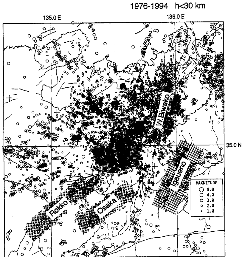
Fig. 10 Lineations of seismic activities (longer than 30km). These were proposed sites for the future major events.
