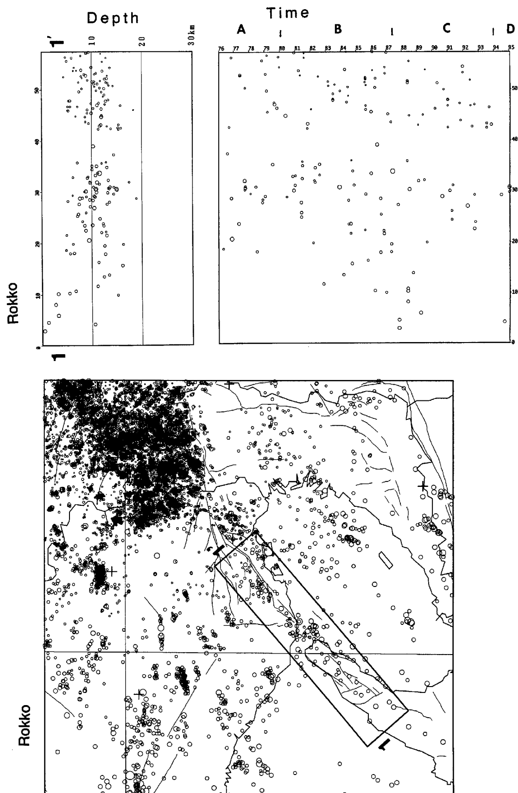
Fig. 12 (a) Distributions of epicenters, depths and time-spaces, for Rokko lineation.
