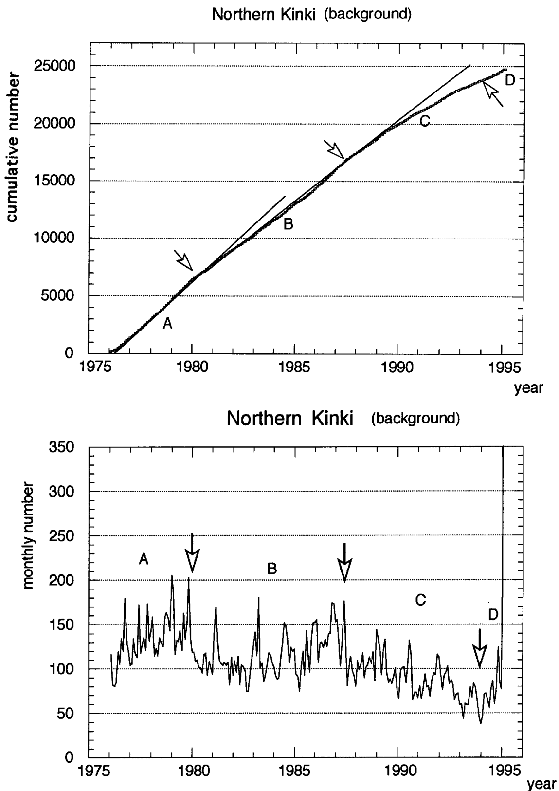
Fig. 6 Temporal variation of monthly numbers (lower) and their cumulative curve (upper). The arrows divide the pre-mainshock activity into 4 characteristic intervals A~D.
