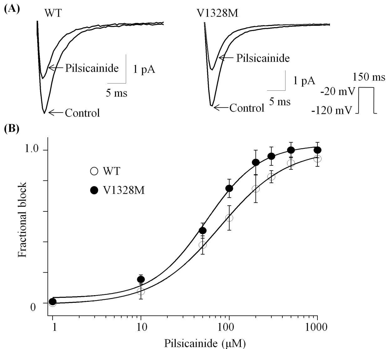
Fig 5. Tonic block of WT and V1328M by pilsicainide. (A) Representative traces in WT and V1328M in the absence or presence of 50 μM pilsicainide. Currents were elicited every 15 seconds by 150 ms pulses to -20 mV from a holding potential of -120 mV. (B) Dose-response relationship of the tonic block. The data were fitted with the Hill equation: y = 1/[1 + (x/K_i)^n] , where y represents the fractional block; x is the concentration of quinidine; K_i is the half-maximal concentration of inhibition; and n is the Hill coefficient. Numbers in parentheses are the number of patches.
