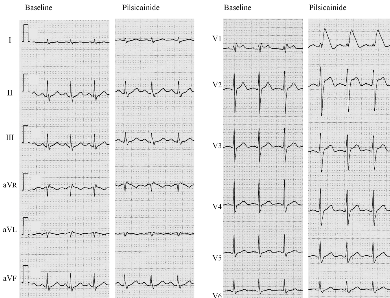
Fig 2. ECG phenotypes on pilsicainide. Left panels show baseline ECGs and the right panels show the ECGs after intravenous injection of pilsicainide (0.8 mg/kg).
