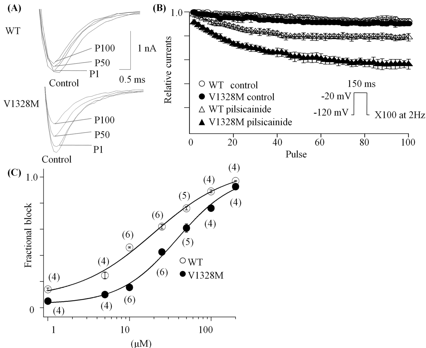
Fig 6. Use-dependent block of WT and V1328M by pilsicainide. (A) Superimposed current traces in the absence or presence of 10 \mu M pilsicainide at pulse number 1, 50 and 100 (P1, P50 and P100). Currents were elicited every 0.5 second by 150 ms pulses to -20 mV from a holding potential of -120 mV. (B) Normalized currents were plotted against the pulse number. (C) Dose-response relationships of the use-dependent block. Fractional block was estimated at pulse #100 in the absence or presence of the drug. The data were fitted with the Hill equation.
