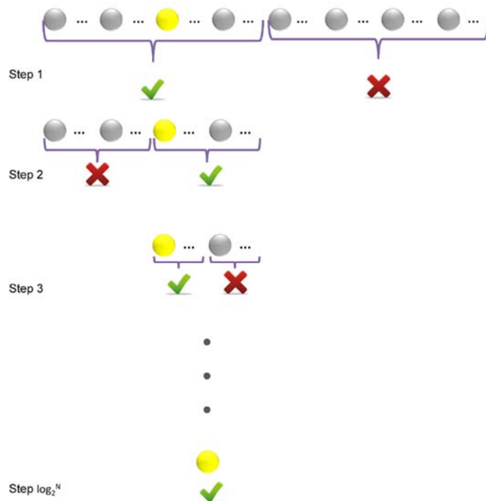
Figure 2-6. Bisection-based method.
