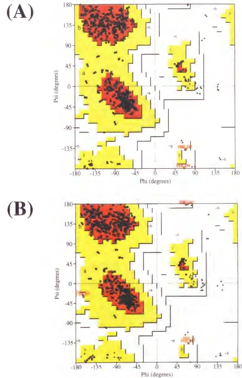
Fig. 4-2. Ramachandran plot of the backbone torsion angles of BSAR bound with PLP-L-Ala (A) and that with PLP-D-Ala (B). Triangles and squares indicate glycine and non-glycine residues, respectively.
