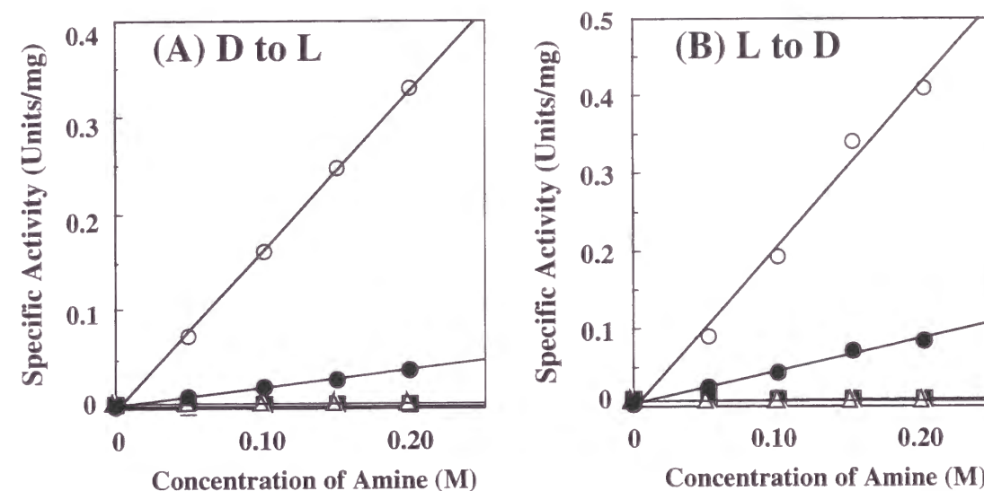
Fig. 2-2. Amine-assisted racemization catalyzed by the K39A mutant enzyme. The specific activities of the K39A mutant enzyme for the reactions from D- to L-alanine (A), and L- to D-alanine (B) were measured in the presence of various concentrations of methylamine at pH 9.0 (●) and 10.5 (○), dimethylamine at pH 10.5 (■), and diethylamine at pH 10.5 (Δ).
