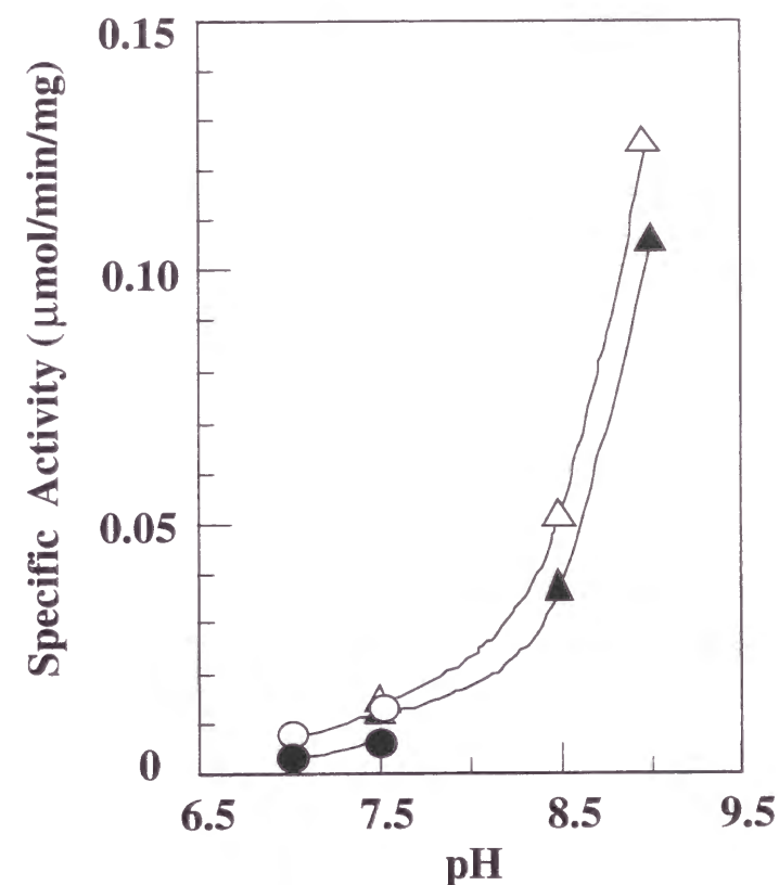
Fig. 5-2. Effect of pH on the rate of \alpha,\beta -elimination of \beta -Cl-D- and L-Ala catalyzed by K39A mutant enzyme in the presence of methylamine. The reaction was carried out with 10 mM \beta -Cl-D-Ala (open symbol) or \beta -Cl-L-Ala (closed symbol), 100 mM HEPES buffer (circle, pH 7.0 and 7.5) or Bis-Tris-Propane buffer (triangle, pH 7.5, 8.5, and 9.0), and 75 \mu g of a homogeneous preparation of K39A mutant enzyme in the presence of 100 mM methylamine. Other conditions were the same as those described in the EXPERIMENTAL PROCEDURES in this chapter.
