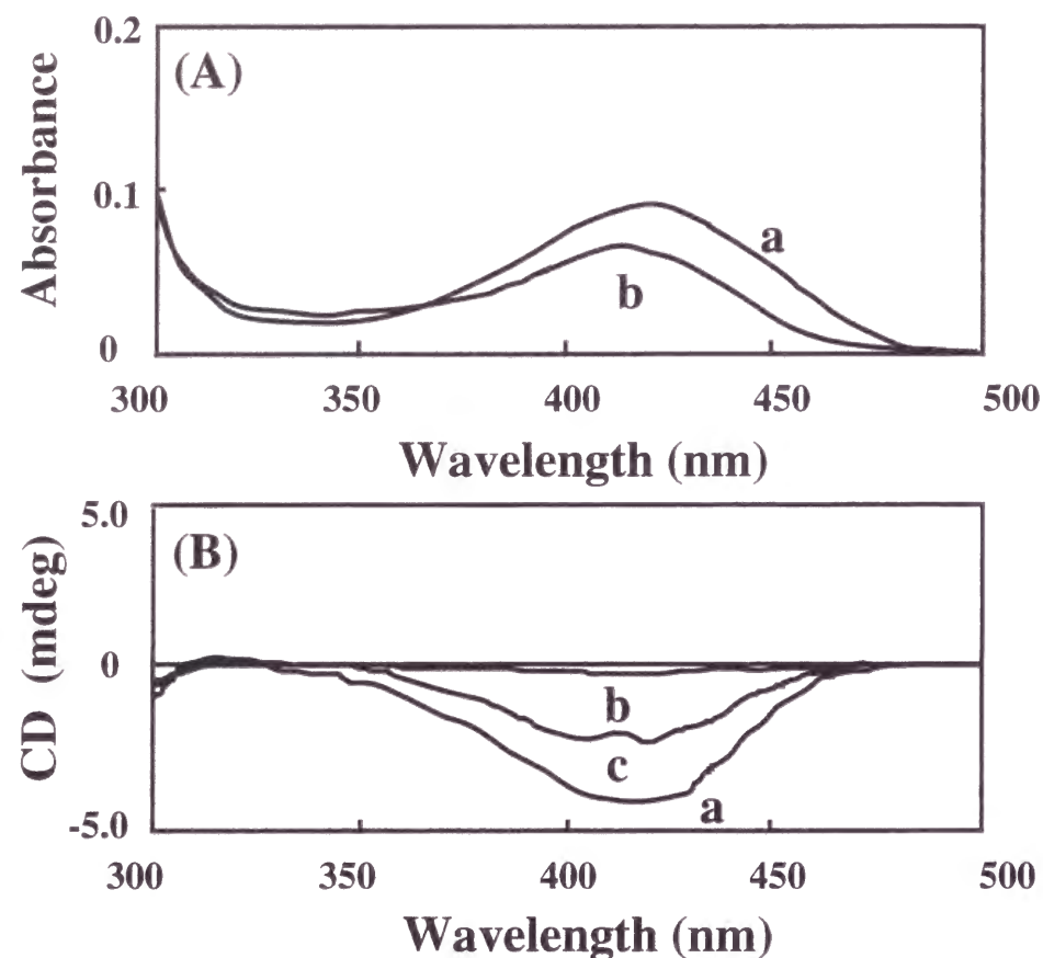
Fig. 2-1. Absorption (A) and circular dichroism (B) spectra of the wild-type and the K39A mutant alanine racemases. Absorption spectra of the wild-type (a) and K39A mutant (b) alanine racemases were taken in 20 mM potassium phosphate buffer (pH 7.2) containing 0.01% 2-mercaptoethanol at a protein concentration of 1.0 mg/ml. CD spectra of the wild-type enzyme (a), and the K39A mutant enzyme in the absence (b) or presence (c) of 500 mM methylamine were taken in 20 mM CAPS buffer (pH 10.5) containing 0.01% 2-mercaptoethanol at a protein concentration of 2.0 mg/ml with a JASCO J-600 recording spectropolarimeter at 25 °C with a 0.1 or 1.0-cm light path length cell under nitrogen atmosphere.
