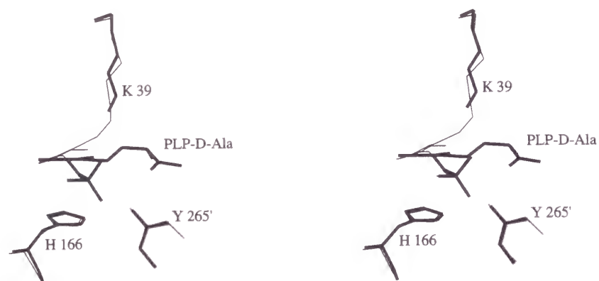
Fig. 4-6. Stereodiagram of the active-site of PLP-form BSAR (thin line) overlaid with BSAR bound with PLP-D-Ala (thick line).
