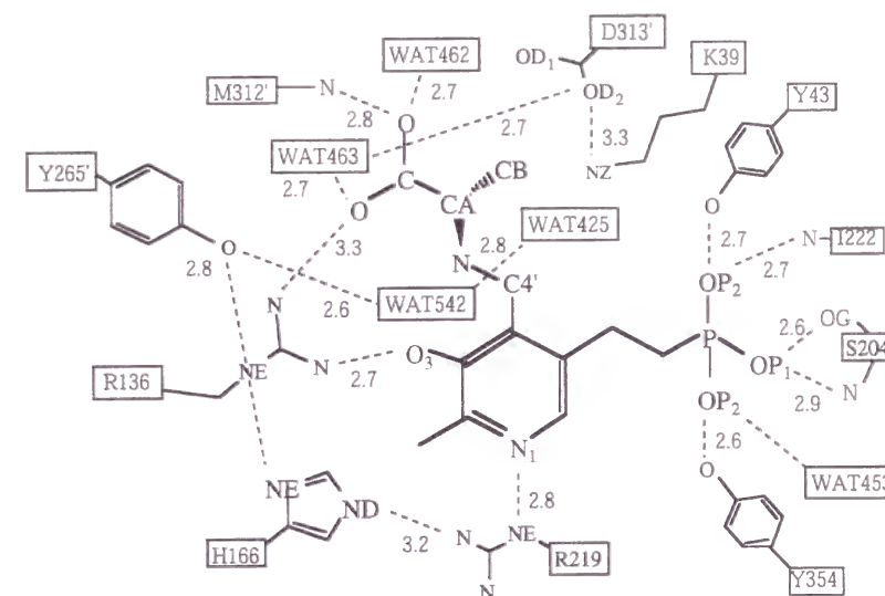
Fig. 4-8. Schematic diagram of the active-site of BSAR bound with PLP-L-Ala. Presumed hydrogen bonds are indicated by dashed lines between atoms that are separated by less than 3.3 Å.
