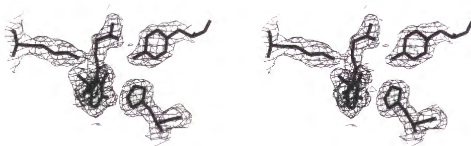
Fig. 4-7. Stereoview of BSAR bound with PLP-D-Ala. The electron density shown was calculated using a simulated annealing omit map with coefficients 2Fo-Fc map contoured at 1.0 sigma.
