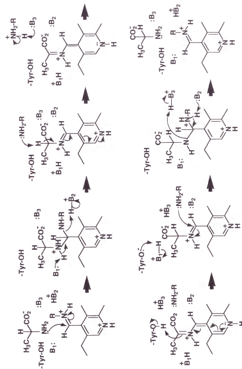
Scheme 2-1. Proposed mechanism of amine-assisted alanine racemization reactions catalyzed by K39A mutant enzyme. B 1 , B 2 and B 3 are the side chains of amino acid residues presumably participating in proton donation and abstraction. The phenolic hydroxyl group of Tyr265' is assumed to be the second base abstracting \alpha -hydrogen from alanyl-PLP aldimine and donating a proton to the \alpha -position of the carbanion intermediate.
