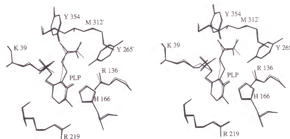
Fig. 4-3. Stereodiagram of the active site of BSAR bound with PLP-L-Ala (thick line) overlaid with that bound with PLP-D-Ala (thin line).
