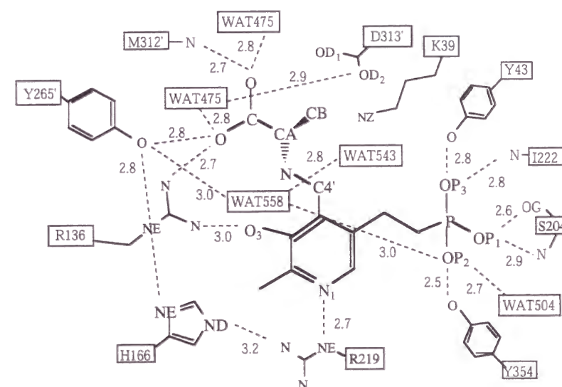
Fig. 4-9. Schematic diagram of the active-site of BSAR bound with PLP-D-Ala. Presumed hydrogen bonds are indicated by dashed lines between atoms that are separated by less than 3.3 Å.
