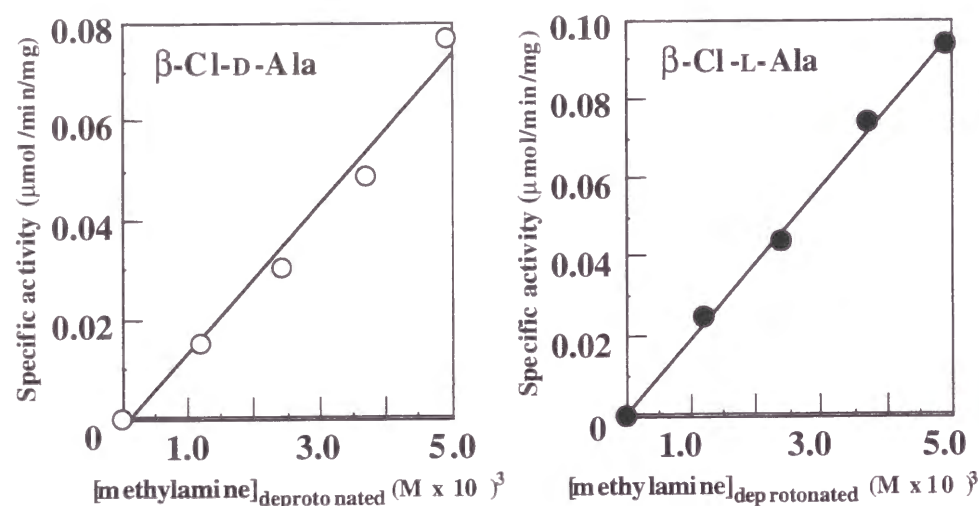
Fig. 5-3. Effect of concentration of methylamine on the rate of \alpha,\beta -elimination of \beta -Cl-D- and L-Ala catalyzed by K39A mutant enzyme.
