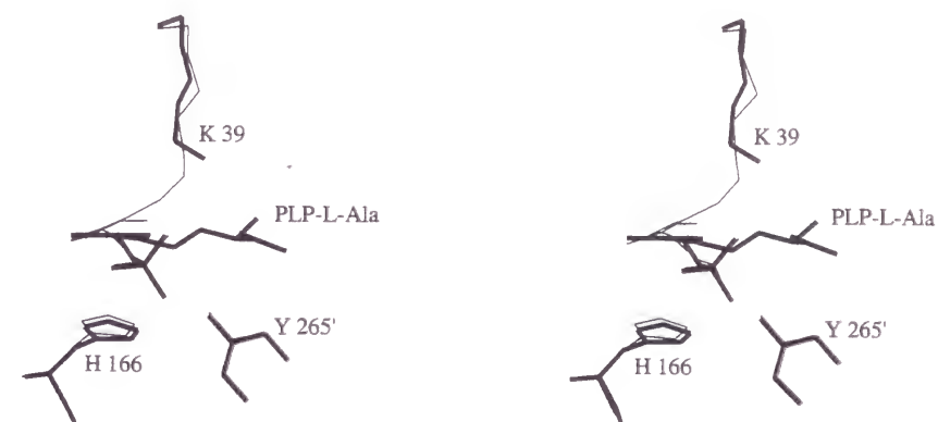
Fig. 4-4. Stereodigram of the active-site of PLP-form BSAR (thin line) overlaid with BSAR bound with PLP-L-Ala (thick line).
