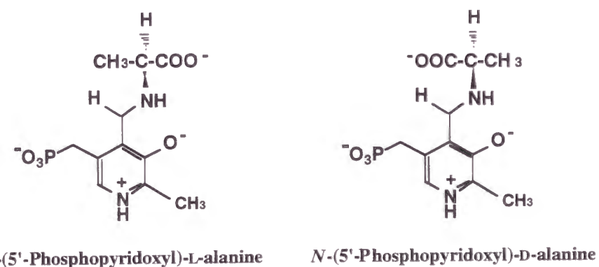
Fig. 4-1. Structures of the external aldimine intermediate analogues.
