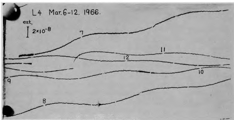
Photo. 1(b). The abrupt change in the crustal strain in the direction of the S38°W at Osakayama during the earthquake in the suburb (Mar. 1966), observed with H-59-D type extensometer.
