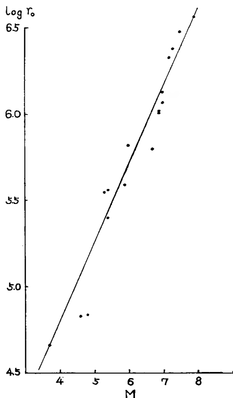
Fig. 3. The relation between the radius of the fault area r_0 and seismic magnitude M . The full line is \log r_0 = 0.45M + 3.00 .
