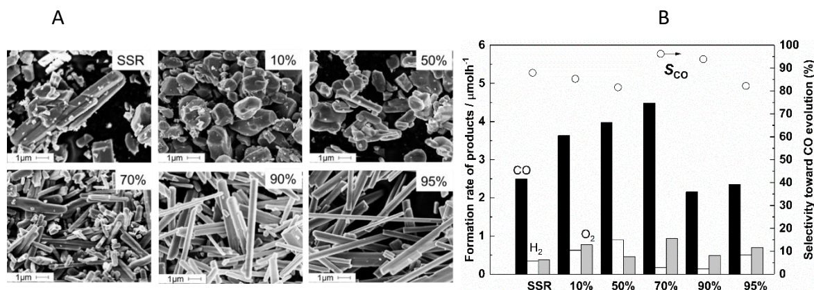
Fig. 9 SEM images(A) and photocatalytic activity(B) of prepared KTO samples by a flux method with different molar ratio x of potassium chloride, where x [mol%] = 100 \times (\text{amount of KTO a flux [mol]}) / (\text{amount of KTO[mol]} + \text{amount of a flux [mol]}) , Formation rates of CO (black bar), H 2 (white bar), and O 2 (grey bar) and the S_{CO} evolution (open circles).
