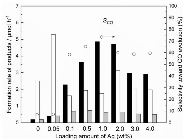
Fig. 13 Formation rates of CO (black bar), H 2 (white bar), and O 2 (grey bar) and the S_{CO} (open circles) in the photocatalytic conversion of CO 2 over the Ag/NTO( NaCl ,PD) samples with different loading amount of Ag cocatalyst. The formation rates were recorded after 1 hour's irradiation. Photocatalyst powder: 0.2 g, reaction solution volume: 350 mL, additive: 0.5 M NaHCO 3 , Ag loading method: photodeposition method, CO 2 flow rate: 15 mL min -1 , light source: 100-W high-pressure Hg lamp.
