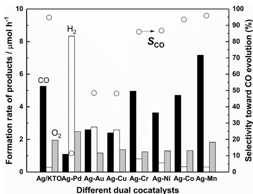
Fig. 4 Formation rates of CO (black bar), H 2 (white bar), and O 2 (grey bar) and the S_{\text{CO}} (open circles) in the photocatalytic CO 2 reduction with H 2 O over the prepared KTO samples, (a) Ag(1.0)/KTO, (b) Ag(1.0)-Pd(1.0)/KTO, (c) Ag(1.0)-Au(0.85)/KTO, (d) Ag(1.0)-Cu(1.0)/KTO, (e) Ag(1.0)-Cr(0.006)/KTO, (f) Ag(1.0)-Ni(0.02)/KTO, (g) Ag(1.0)-Co(0.02)/KTO, and (h) Ag(1.0)-Mn(0.09)/KTO.
