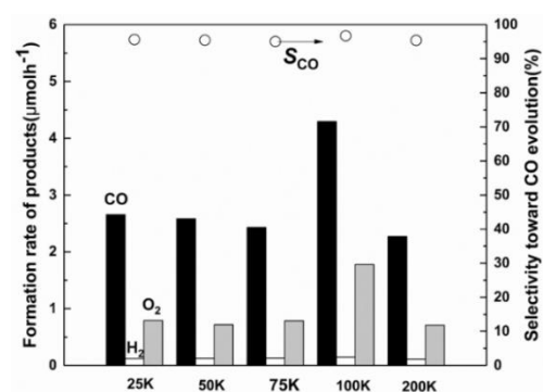
Fig. 18 photocatalytic activity of CO (black bar), H 2 (white bar), O 2 (grey bar) and the S CO evolution (open circles) over the prepared KTO samples by a flux method at different cooling rate.
