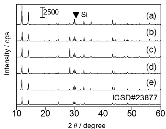
Fig. 7 XRD patterns of the prepared NTO samples with various flux; (a) NaCl, (b) NaCl:KCl=3:1, (c) NaCl:KCl=1:1, (d) NaCl:KCl=1:3, (e) KCl, and ICSD#23877 for Na 2 Ti 6 O 13 .
