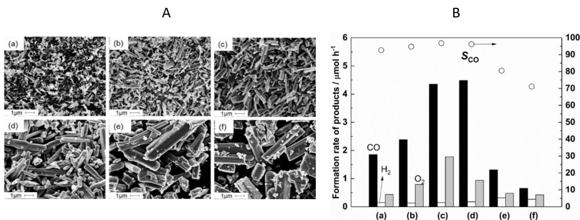
Fig. 12 SEM images (A) and photocatalytic activity (B) of CO (black bar), H 2 (white bar), and O 2 (grey bar) and the S_{\text{CO}} evolution (open circles) over the prepared KTO samples by a flux method at different holding temperature, (a)1073 K, (b)1173 K, (c)1273 K, (d)1373 K, (e)1473 K and (f)1573 K.
