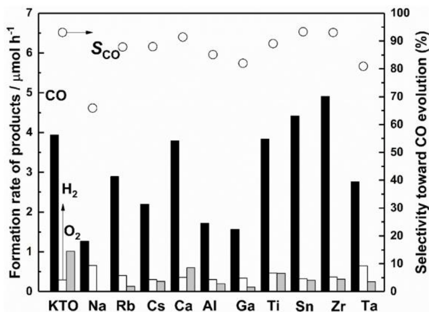
Fig. 4 Formation rates of CO (black bar), H 2 (white bar), and O 2 (gray bar) and the CO selectivity ( S_{CO}\% , open circles) in the photocatalytic reaction tests over the 1 wt% Ag/KTO:M(2 mol%) samples, where the metal ions were modified by a flux mediate method.
