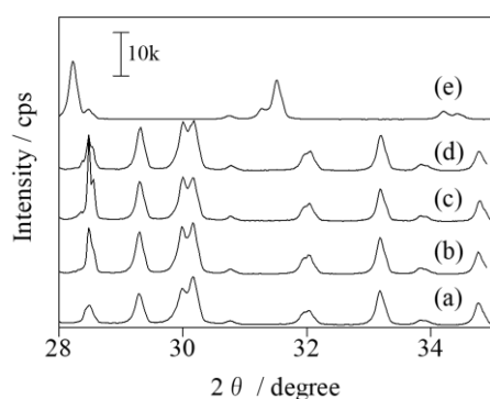
Fig. 12 XRD patterns of prepared KTO:Zr samples, (a) bare KTO, (b) 0.5 mol%, (c) 2 mol%, (d) 5 mol%, (e) KxZrOz.
