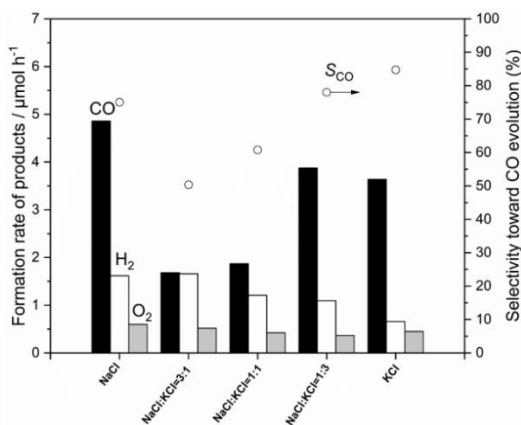
Fig. 10 Formation rates of CO (black bar), H 2 (white bar), and O 2 (grey bar) and the S_{\text{CO}} evolution (open circles) in the photocatalytic reaction tests with the Ag/NTO( NaCl:KCl ) samples prepared by using the mixed flux consisting of different ratio of NaCl and KCl.
