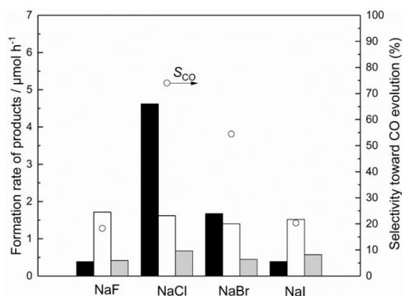
Fig. 9 Formation rates of CO (black bar), H 2 (white bar), and O 2 (grey bar) and the S_{\text{CO}} evolution (open circles) in the photocatalytic reaction tests with the Ag/NTO( NaX ) ( X : F, Cl, Br, and I) samples prepared by using various fluxes. The values were recorded after 1 hour's irradiation. Ag cocatalyst was loaded by the PD method.
