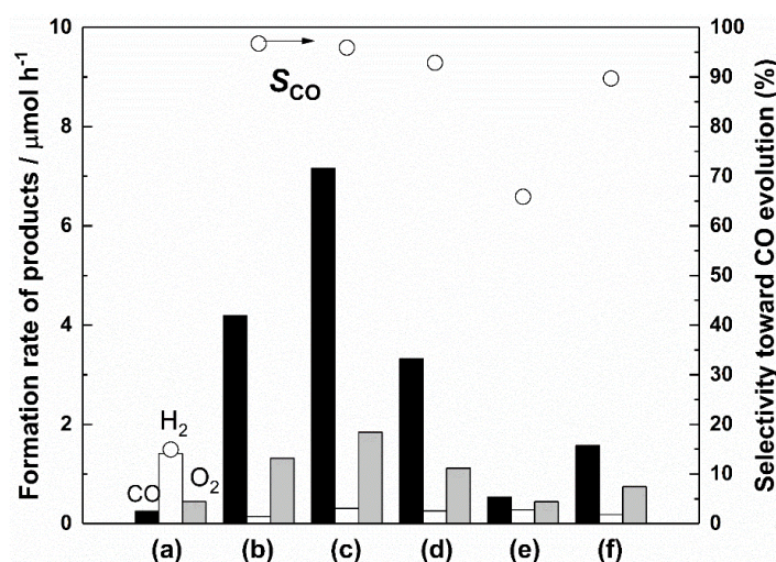
Fig. 4 Photocatalytic reduction of \text{CO}_2 over the prepared samples loaded with different methods, (a) bare KTO, (b) \text{Ag}/\text{KTO} , (c) \text{MnO}_x(\text{PD, 0.09})\text{-Ag(PD, 1.0)}/\text{KTO} , (d) \text{MnO}_x(\text{IMP, 1.0})/\text{Ag(PD, 1.0)}/\text{KTO} , (e) \text{Ag(PD, 1.0)}/\text{MnO}_x(\text{IMP, 1.0})/\text{KTO} , and (f) \text{MnO}_x(\text{IMP, 1.0})\text{-Ag(IMP,1.0)}/\text{KTO} .
