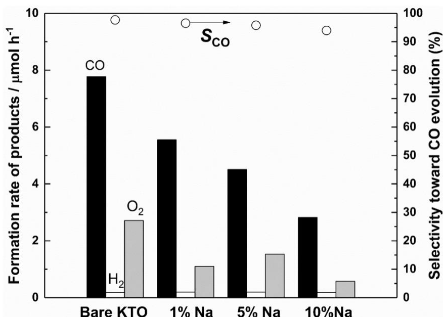
Fig. 3 Formation rates of CO (black bar), H 2 (white bar), and O 2 (gray bar) and the CO selectivity ( S_{\text{CO}}\% , open circles) in the photocatalytic reaction tests over the \text{MnO}_x\text{-Ag/KTO\_Na}(x \text{ mol}\%) samples, where loading amount of \text{MnO}_x and Ag cocatalyst was both 1 wt%.
