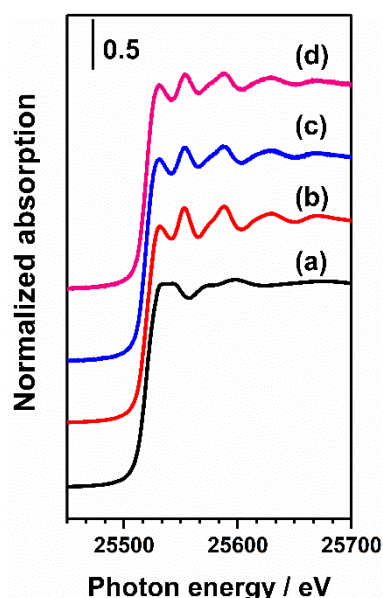
Fig. 19 Ag K-edge XANES of (a) \text{Ag}_2\text{O} , (b) Ag foil, (c) Ag/KTO_before reaction, and (d) Ag/KTO_after reaction.
