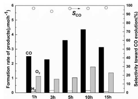
Fig. 16 photocatalytic activity of CO (black bar), H 2 (white bar), O 2 (grey bar) and the S_{CO} evolution (open circles) over the prepared KTO samples by a flux method at different cooling rate.
