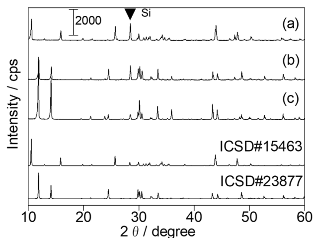
Fig. 1 XRD patterns of the samples; (a) the \text{Na}_2\text{Ti}_3\text{O}_7(\text{SSR}) sample, (b) the \text{NTO}(\text{SSR}) sample, and (c) the \text{NTO}(\text{NaCl}) sample. Silicon powder mixed to calibrate the angle showed a diffraction indicated by a closed triangle. The patterns from the ICSD database are also shown, ICSD#15463 for \text{Na}_2\text{Ti}_3\text{O}_7 and ICSD#23877 for \text{Na}_2\text{Ti}_6\text{O}_{13} .
