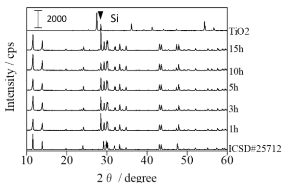
Fig. 13 XRD patterns of prepared KTO samples by a flux method at different holding temperature.
