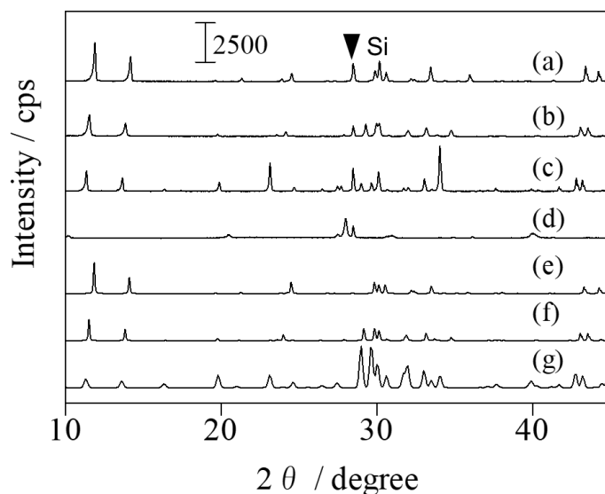
Fig. 3 XRD patterns of prepared \text{A}_2\text{Ti}_6\text{O}_{13} samples; (a) \text{Na}_2\text{Ti}_6\text{O}_{13}(\text{NaCl}) , (b) \text{K}_2\text{Ti}_6\text{O}_{13}(\text{KCl}) , (c) \text{Rb}_2\text{Ti}_6\text{O}_{13}(\text{RbCl}) and \text{Cs}_2\text{Ti}_6\text{O}_{13}(\text{SSR}) . Silicon powder mixed to calibrate the angle showed a diffraction indicated by a closed triangle. The patterns from the ICSD database are also shown, ICSD#23877 for \text{Na}_2\text{Ti}_6\text{O}_{13} (e), ICSD#25712 for \text{K}_2\text{Ti}_6\text{O}_{13} (f) and ICSD#23878 for \text{Rb}_2\text{Ti}_6\text{O}_{13} (g).
