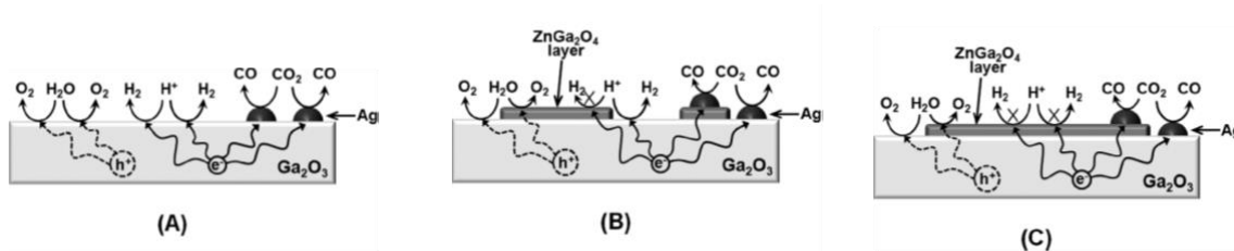
Fig. 2 A proposed mechanism for the photocatalytic conversion of CO 2 in and with H 2 O over Ag-loaded Ga 2 O 3 (A), Ag-loaded Zn modified Ga 2 O 3 with a low Zn content (B), and Ag-loaded Zn-modified Ga 2 O 3 with a high Zn content (C). 32
