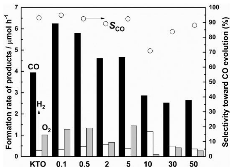
Fig. 5 Formation rates of CO (black bar), H 2 (white bar), and O 2 (gray bar) and the selectivity to CO ( S_{CO} %, open circles) in the photocatalytic reaction tests over the 1 wt% Ag/KTO modified with Ca 2+ by a flux mediate method.
