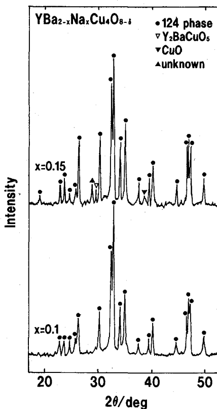
Fig. 4. The XRD patterns of \text{YBa}_{2-x}\text{Na}_x\text{Cu}_4\text{O}_{8-\delta} phases obtained by heating the gel at 780°C for 30–50 h in flowing oxygen.
