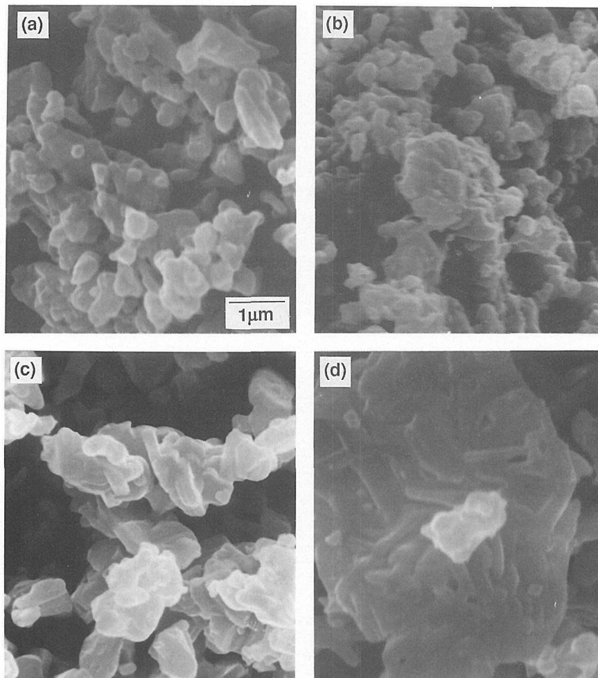
Fig. 7. The SEM photographs of the sintered pellets of \text{YBa}_{2-x}\text{R}_x\text{Cu}_4\text{O}_8 ; (a) non-substituted 124 phase, (b) \text{R}=\text{Sr} , x=0.4 , (c) \text{R}=\text{Na} , x=0.1 and (d) \text{R}=\text{K} , x=0.2 .
