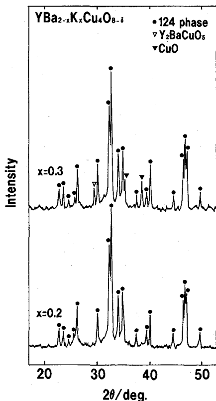
Fig. 3. The XRD patterns of \text{YBa}_{2-x}\text{K}_x\text{Cu}_4\text{O}_{8-\delta} phases obtained by heating the gel at 780°C for 30–50 h in flowing oxygen.
