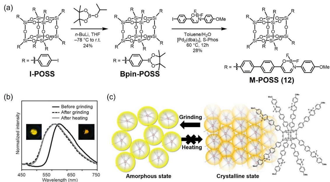
Figure 11. (a) Synthetic scheme of M-POSS (12) . (b) PL spectra of M-POSS in solid states. The ground sample was heated at 200^\circ\text{C} for 10 min. THF vapor was fumed to the ground sample. Inserted photographs are M-POSS before and after grinding under visible and UV (365 nm) light irradiation. (c) Schematic illustration of heat-resistant mechanochromism of M-POSS . Reprinted with permission from ref 30. Copyright 2017 WILEY-VCH Verlag GmbH & Co. KGaA, Weinheim.
