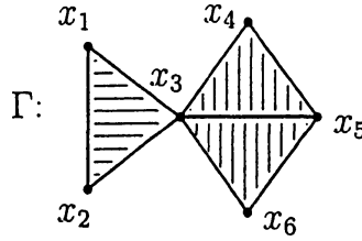
FIGURE 1. \Gamma = \langle \{x_1, x_2, x_3\}, \{x_3, x_4, x_5\}, \{x_3, x_5, x_6\} \rangle
