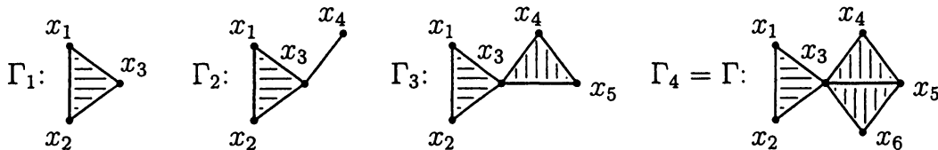
FIGURE 2. Generalized trees
