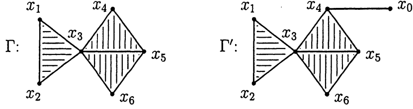
FIGURE 3. \Gamma and \Gamma'
