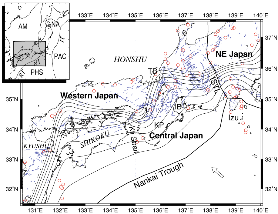
Fig. 1 Location map of central and western Japan. Thick solid lines represent plate boundaries after Bird (2003). Red open circles are epicenters of very shallow ( \leq 20 km), historical ( 1586 \leq \text{year} \leq 2013 ), and large ( M \geq 6.5 ) earthquakes from the Catalog of Damaging Earthquakes in the World (Utsu 1990, 2002, 2004, the later updates are added by the International Institute of Seismology and Earthquake Engineering) with additional depth data for historical earthquakes (Matsu'ura 2017). Thin blue lines are active faults on land (Research Group for Active Faults of Japan 1991). Contour lines of the PHS slab of the CAMP model (Hashimoto et al. 2004) are also shown every 10 km by thin solid lines. The following acronyms are used: ISTL, Itoigawa-Shizuoka tectonic line; KP, Kii Peninsula; IB, Ise Bay; TB, Tsuruga Bay; NE, northeastern; AM, Amurian Plate; PHS, Philippine Sea Plate; PAC, Pacific Plate; NA, North American Plate; JT, Japan Trench; NT, Nankai Trough; RT, Ryukyu Trench
