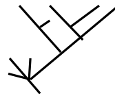
Figure 4. A dendrogram of a general development
