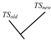
Figure 3. A dendrogram of scientific revolution
