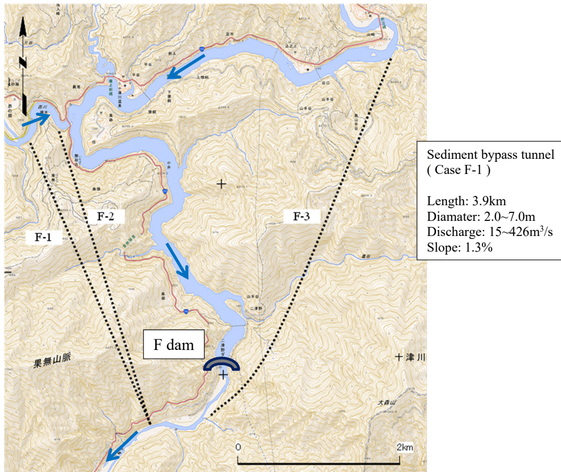
Figure 1: Three options of sediment bypass tunnels for F dam
