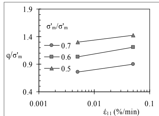
Fig. 4.16(d): q/\sigma'_m vs. \dot{\epsilon}_{11} relationship
