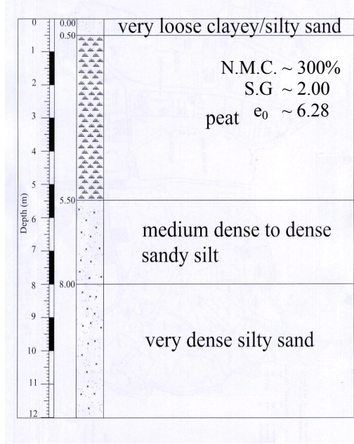
Fig. 5.4: Subsurface profile at the site
