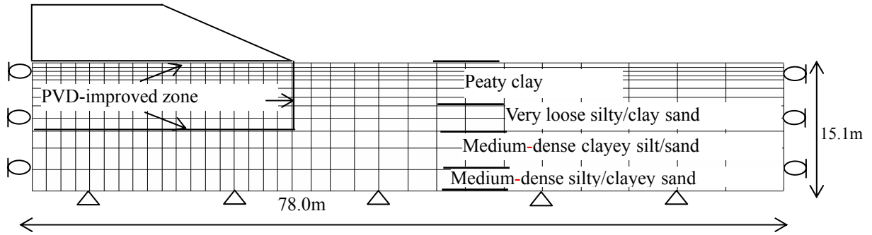
Fig. 7.6: Finite element mesh with boundary conditions
