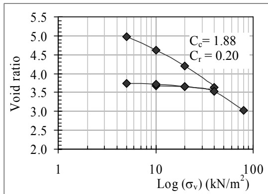
Fig. 4.1: Void ratio vs. \log(\sigma'_v) relationship
