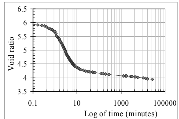
Fig. 4.2: Void ratio vs. \log(\text{time}) relationship
