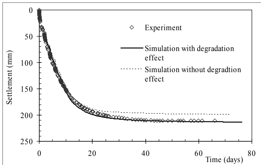
Fig. 7.3: Comparison of the settlements
