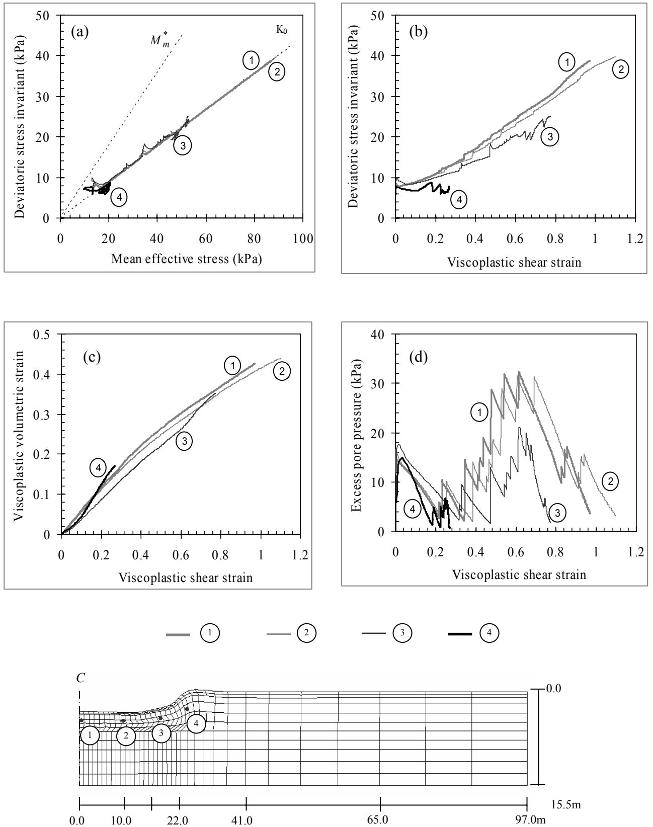
Fig. 6.12: Soil element behavior under the embankment – silty clay/peat 2.75 m depth
