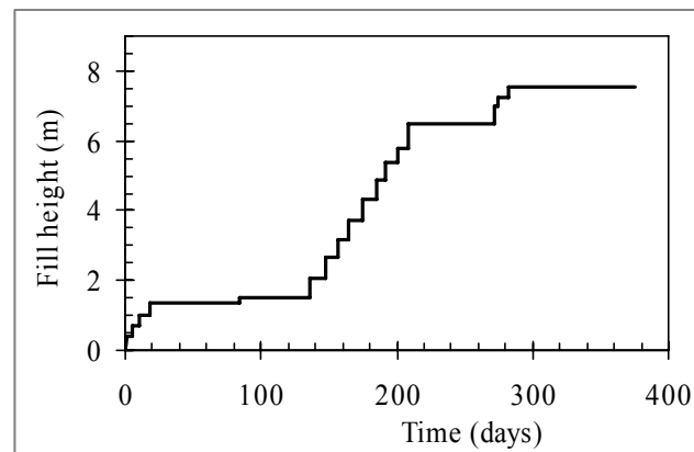
Fig. 7.16: Loading curve
