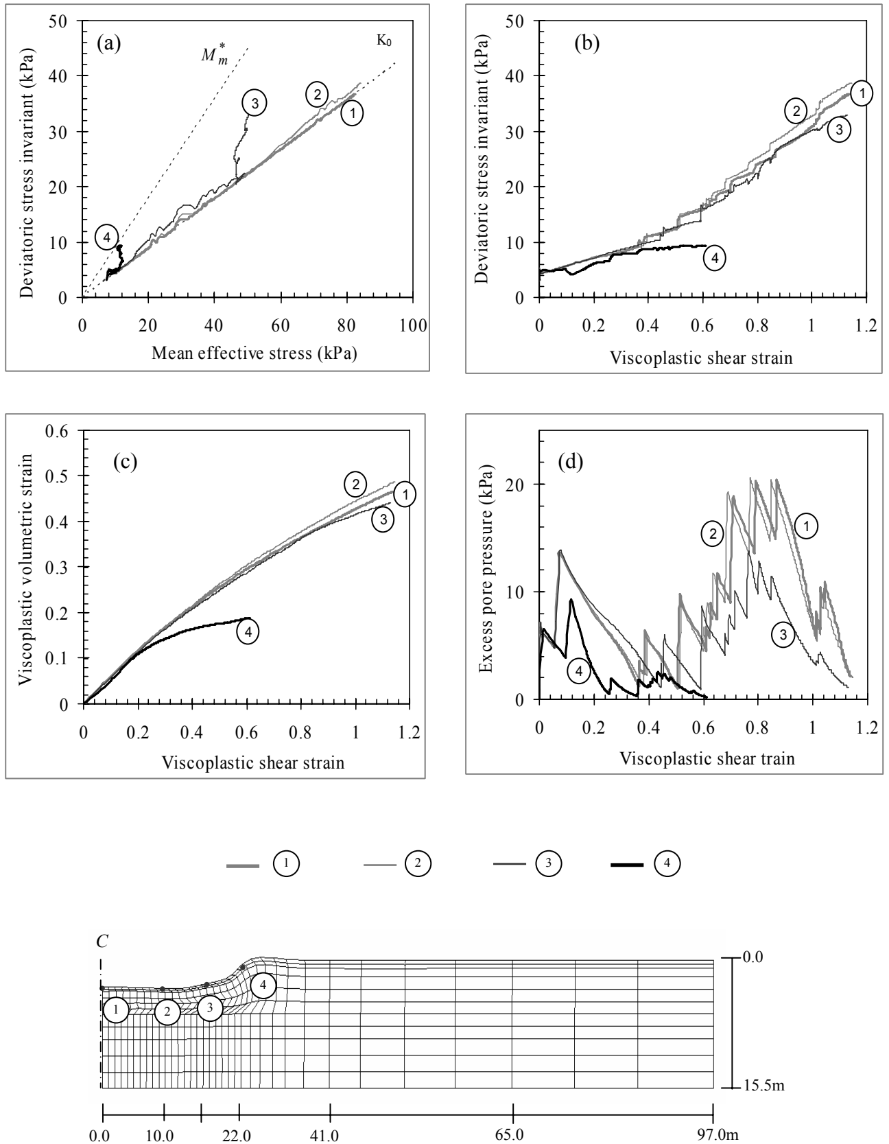
Fig. 6.14: Soil element behavior under the embankment – peat 0.75 m depth
