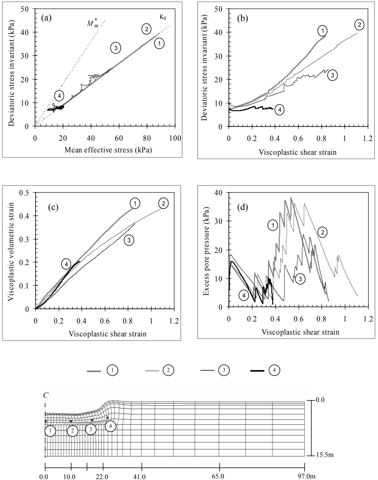
Fig. 6.11: Soil element behavior under the embankment – silty clay/peat 4.25 m depth
