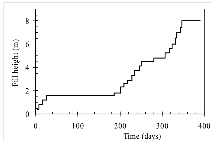
Fig. 7.5: Loading curve
