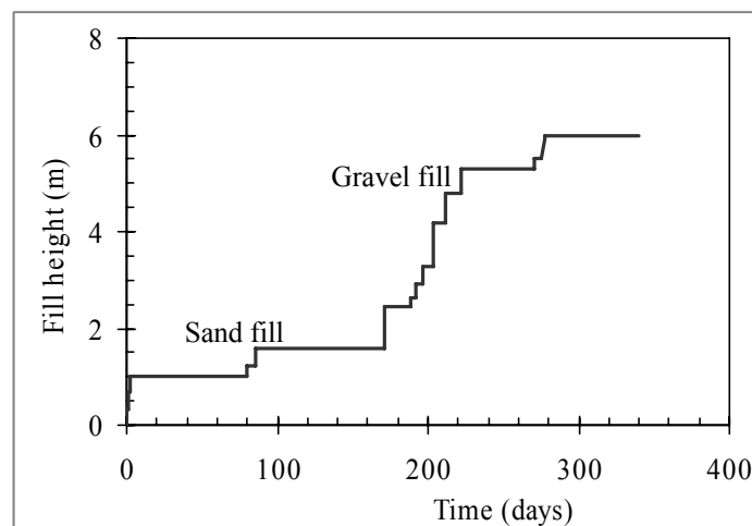
Fig. 6.2: Loading curve
