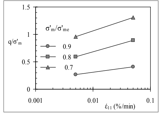
Fig. 3.9: q/\sigma'_m vs. \dot{\epsilon}_{11} relationship
