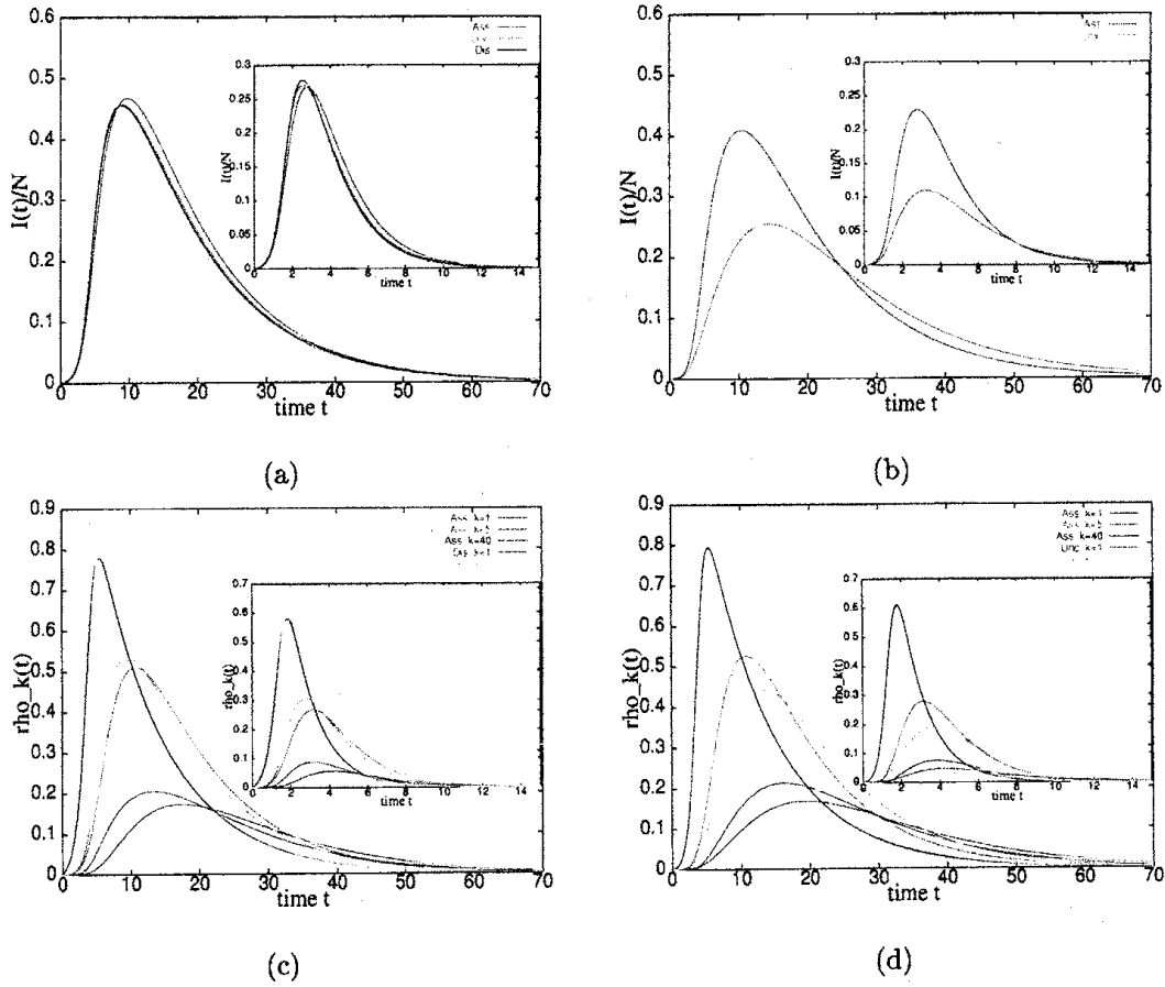
Fig. 3: Time evolutions of (a) the fraction of infected nodes I(t)/N in Dup, (b) I(t)/N in Dir, (c) each \rho_k(t) for k = 1, 5, 40 in Dup, and (d) \rho_k(t) in Dir at b = 0.1 and \delta = 0.1 . Inset figures show similar behavior at b = 0.3 and \delta = 0.5 as some other example. Note that the value of I_k(t) = N_k \times \rho_k(t) is in the reverse order to k because of N_k \propto k^{-\gamma} .
