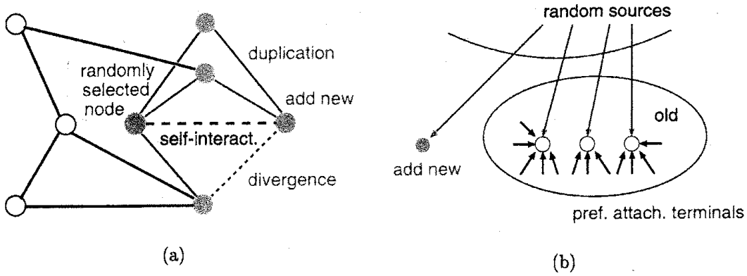
Fig. 1: Growing network models. (a) In the duplication-divergence model, duplication links (red solid lines) between a new node (red circle) and all the neighbors (green circles) of a randomly chosen node (blue circle), and self-interaction (dashed line) are generated, but some links (magenta dashed line) are removed. (b) In the directed growing model, new links from randomly chosen sources to preferentially attached terminals emerge.
