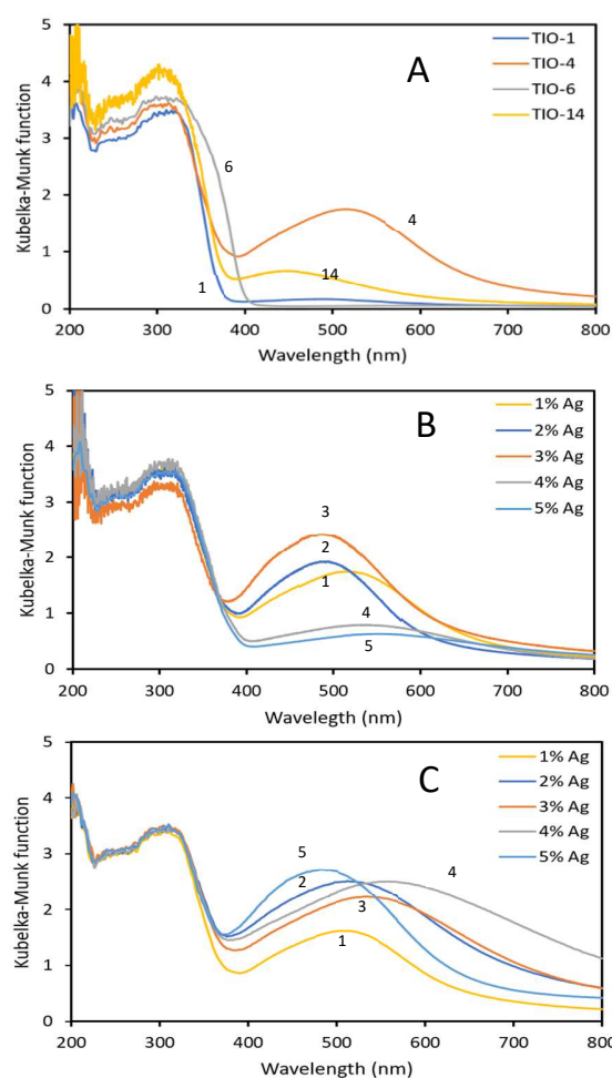
Fig. 1 DR UV-vis spectra of Ag/TiO 2 samples. (A) Ag(1)/TiO 2 (A,y), various TiO 2 samples loaded with 1% Ag photodeposited by method A, (B) Ag(x)/TiO 2 (A,4), TiO 2 samples with different silver loading photodeposited by method A, and (C) Ag(x)/TiO 2 (B,4), TiO 2 samples with different silver loading photodeposited by method B.
