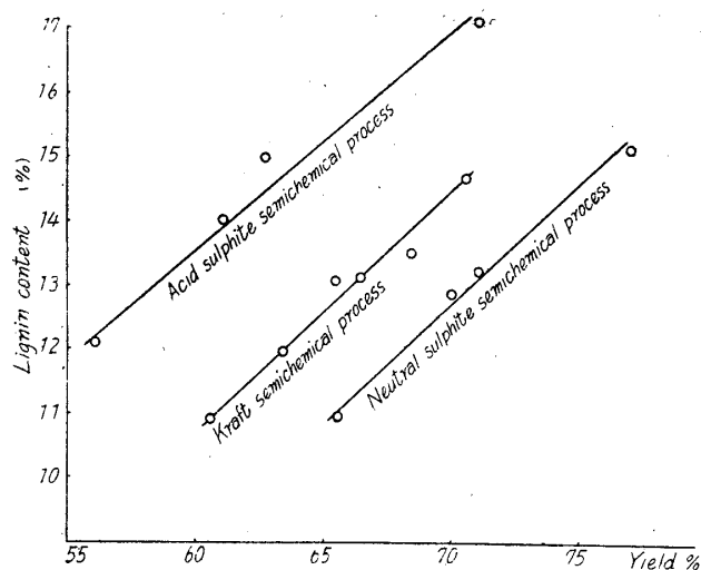
Fig. 1. Relations between Pulp yields and Lignin contents
