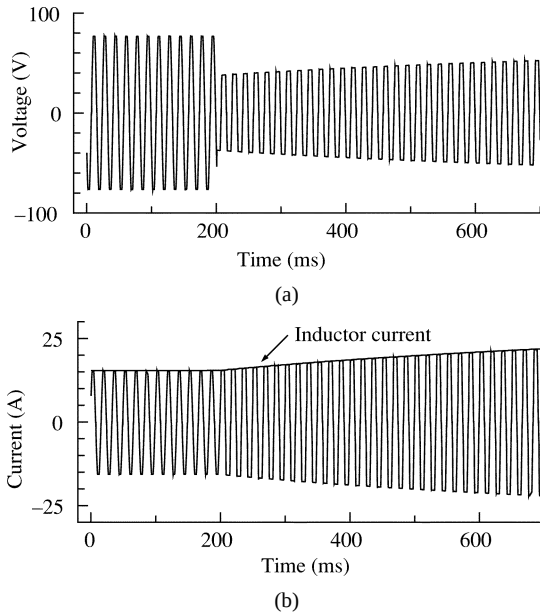
Fig. 8. Long term effect of load increasing. (a) Load voltage. (b) Load current and inductor current.
