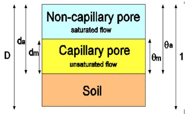
Fig. 5 Surface Soil Layer and Parameters
