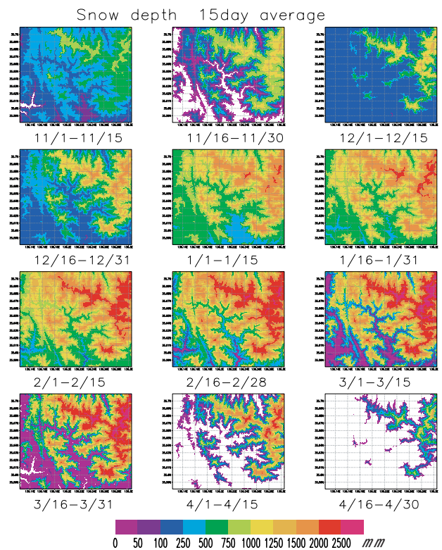
Fig. 12 Modified Snow Depth Distributed Map (15 days averaged, calculated) :2002/11/01~2003/04/30
