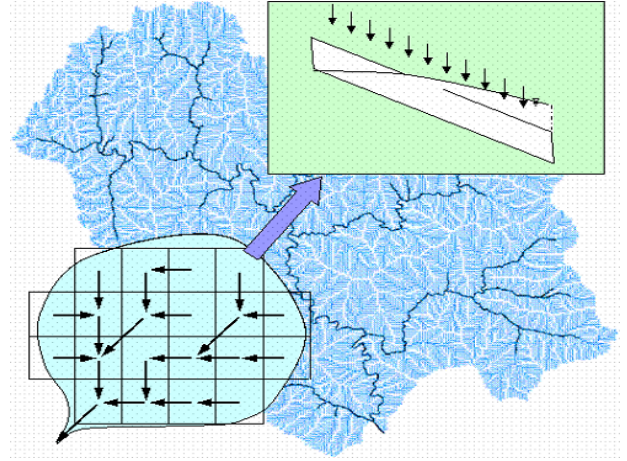
Fig. 4 Schematic image of Cell Distributed Runoff Model
