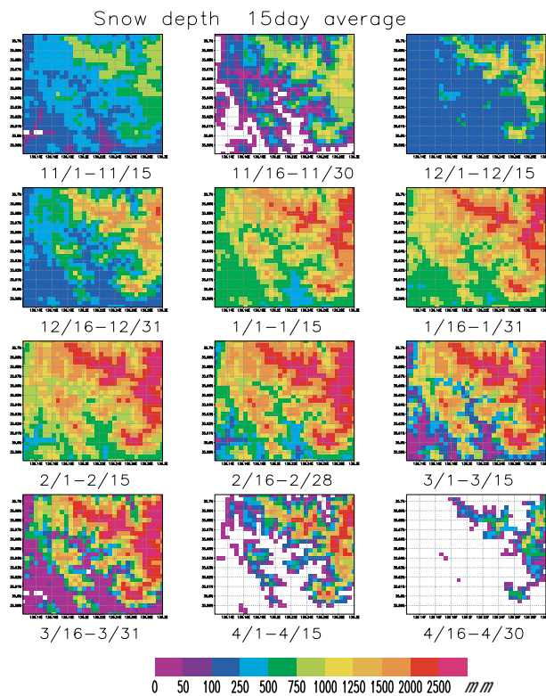
Fig. 11 Snow Depth Distributed Map (15 days averaged, calculated) :2002/11/01~2003/04/30
