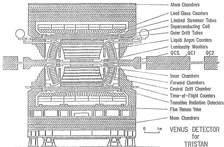
Fig. 2. Side view of the VENUS detector
