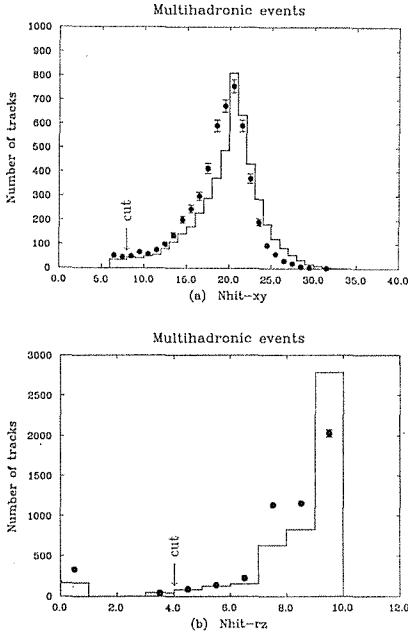
Fig. 6. Number of hits on axial wires (a) and on stereo wires (b) of the tracks for the selected multi-hadronic events (●). The solid lines show the results of the simulations.
