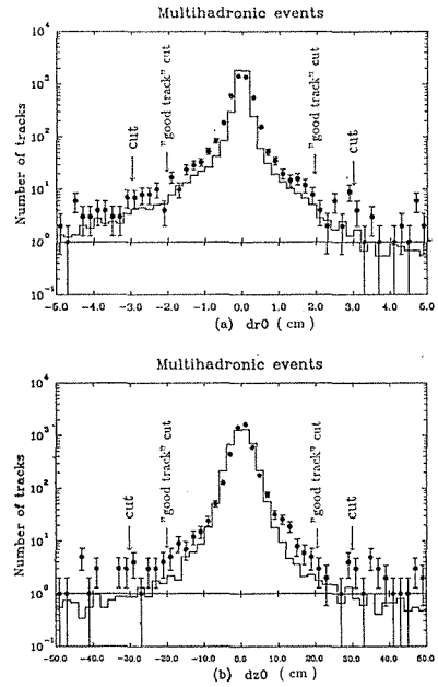
Fig. 7. d_{r0} (a) and d_{z0} (b) distributions of the tracks for the selected multi-hadronic events (●). The solid lines show the results of the simulation.
