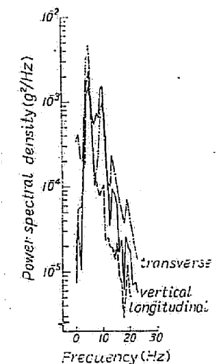
Fig. 4-16 Power Spectra of Vibration of Combine Operator's Back in case of Travelling at 3rd Velocity on the Field.
