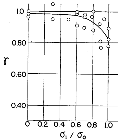
Fig. 1. Experimental Result on the Residual Strength (1) \sigma_1/\sigma_0 =uniaxial compressive stress history.
