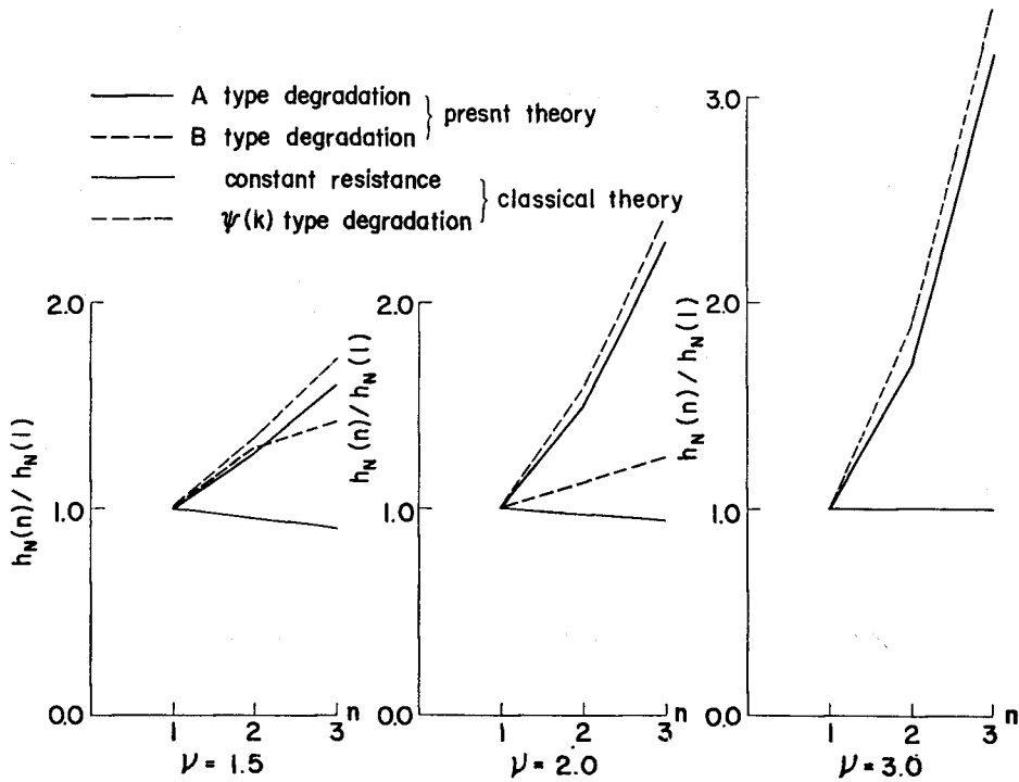
Fig. 9. The Failure Rate Ratio ( c_R=0.10 , c_S=0.4 , c_A=0.10 , c_B=0.10 , \xi=1.0 ).
