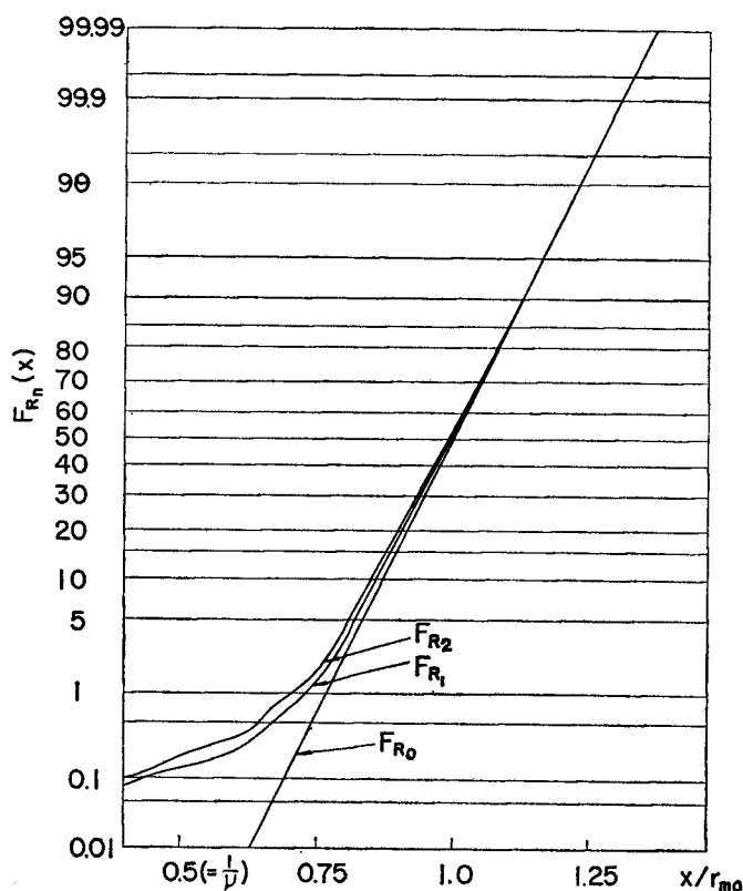
Fig. 6. Probability Distribution of the Residual Strength with the Type B Degradation ( \nu=2.0 , c_R=0.10 , c_B=0.4 , c_B=0.10 ).
