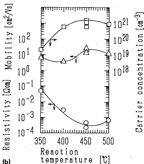
FIG. 3. Electric resistivities, carrier concentrations, and Hall mobilities for (a) \text{In}_2\text{O}_3 and (b) \text{In}_2\text{O}_3\text{:Sn} ( \text{Sn}/\text{In} = 0.01 ) films as a function of reaction temperature.
