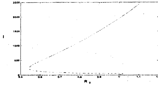
Figure 1: I^* , I_1 and I_2 versus R_0 when d = 0.1 , \lambda = 0.02 , \alpha = 0.5 , r = 0.1 , k = 0.8 , I_0 = 50 , it shows a backward bifurcation with endemic equilibria when R_0 < 1 .
