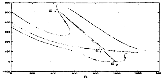
Figure 2: One region of disease persistence and one region of disease extinction when A = 100, d = 0.1, \lambda = 0.02, \alpha = 0.5, r = 0.1, k = 0.8, e = 0.01, I_0 = 50 .
