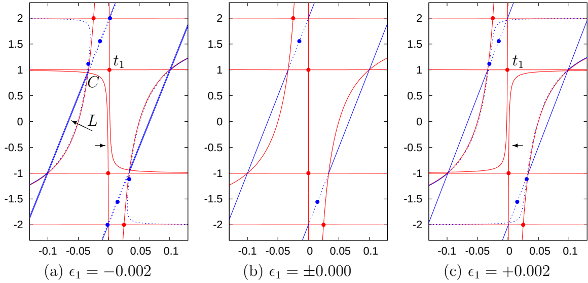
Figure 18: Appearance of a Stokes segment in Example 1. In (b), two turning points at \pm i , both of which are of type (1, 2), are connected by a Stokes curve.
