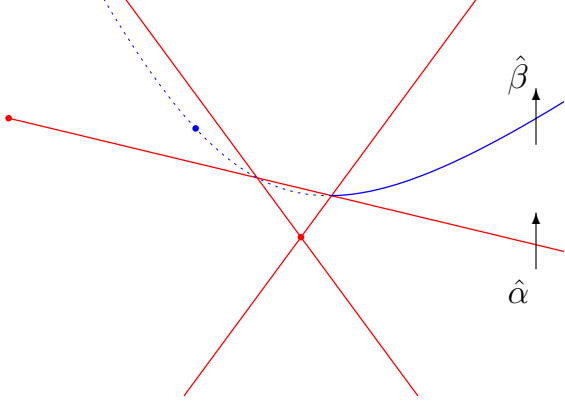
Figure 8: Stokes geometry for a = a_{-1} .
