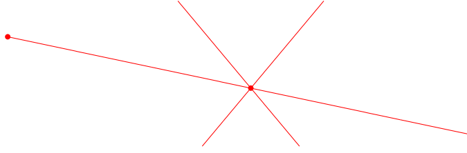
Figure 7: A Stokes curve hits a double turning point.
