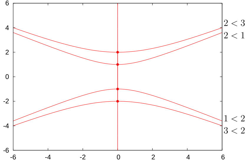
Figure 1: Turning points and ordinary Stokes curves for Example 1 with \epsilon_1 = \epsilon_2 = 0 .
