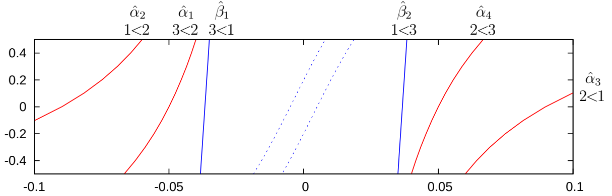
Figure 6: Stokes curves near the real axis for Example 1 with \epsilon_1 = 0.09 and \epsilon_2 = 0.1 .
