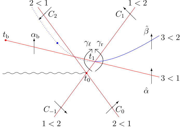
Figure 11: Stokes coefficients for a = a_{-1} .
