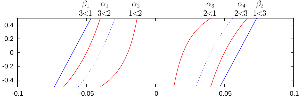
Figure 5: Stokes curves near the real axis for Example 1 with \epsilon_1 = 0.02 and \epsilon_2 = 0.1 .
