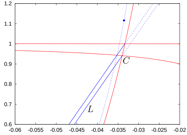
Figure 20: Enlarged figure near the point C in Figure 18 (a).
