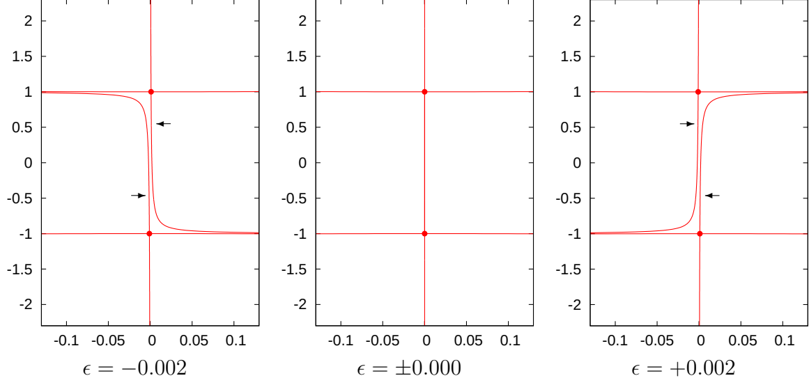
Figure 19: Appearance of a Stokes segment in the two-level system given by \rho_1 = t^2 + 1 + i\epsilon , \rho_2 = 0 .
