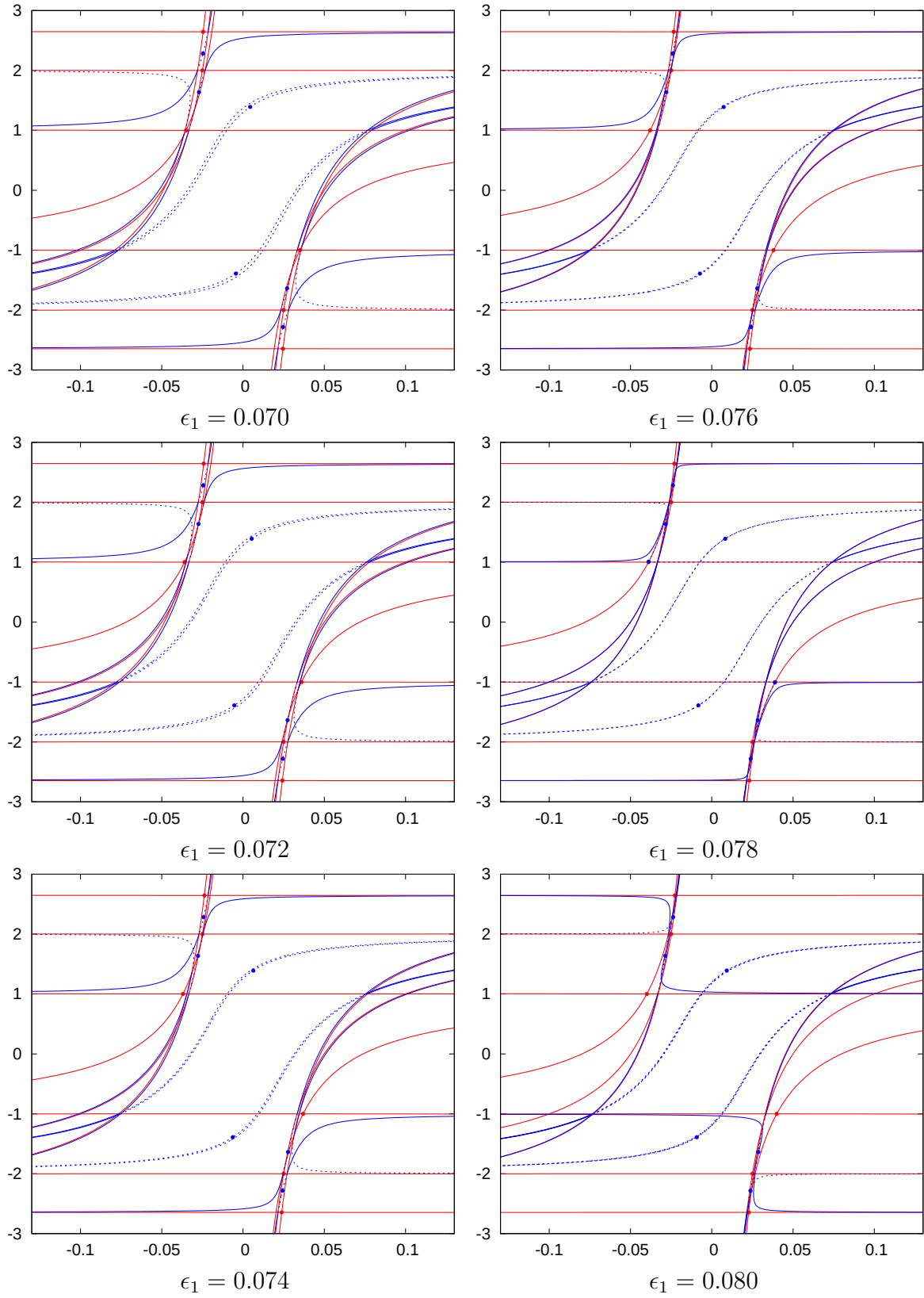
Figure 21: Change of Stokes geometry for Example 2 as \epsilon_1 = 0.07 \rightarrow 0.08 with \epsilon_2 = 0.1 . (Note that some ordinary Stokes curves overlap with new Stokes curves when \epsilon_1 = 0.078 . In such situations overlapping Stokes curves are designated by blue.)
