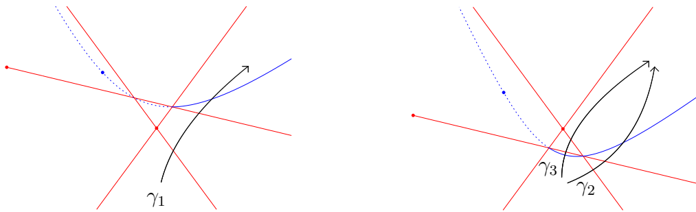
Figure 14: Stokes geometry for Theorem 1
