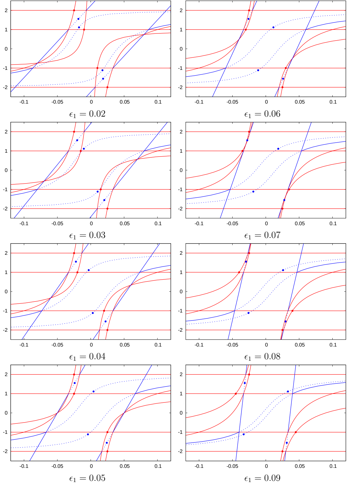
Figure 4: Change of Stokes geometry for Example 1 as \epsilon_1 = 0.02 \rightarrow 0.09 with \epsilon_2 = 0.1 .
