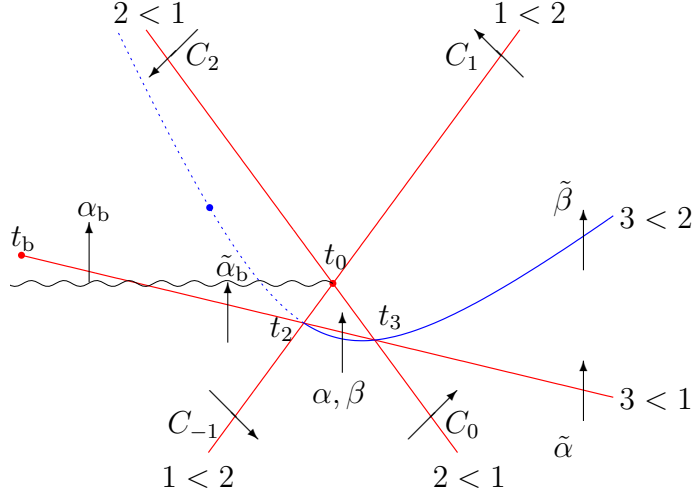
Figure 12: Stokes coefficients for a = a_1 .
