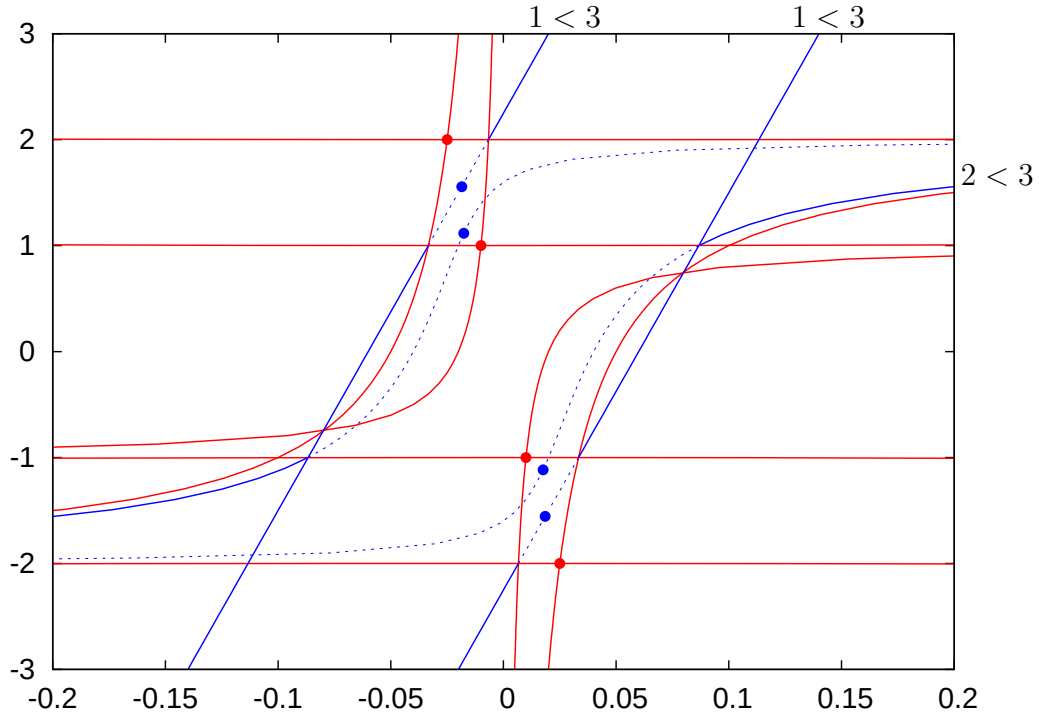
Figure 2: Stokes geometry for Example 1 with \epsilon_1 = 0.02 and \epsilon_2 = 0.1 .
