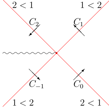
Figure 10: Stokes curves of the canonical equation and Stokes coefficients.
