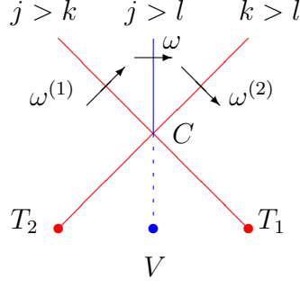
Figure 15: A new Stokes curve emanating from V passes through an ordered crossing point C of two ordinary Stokes curves emanating from T_1 and T_2 ; \omega , \omega^{(1)} and \omega^{(2)} denote the Stokes coefficients attached to them.
