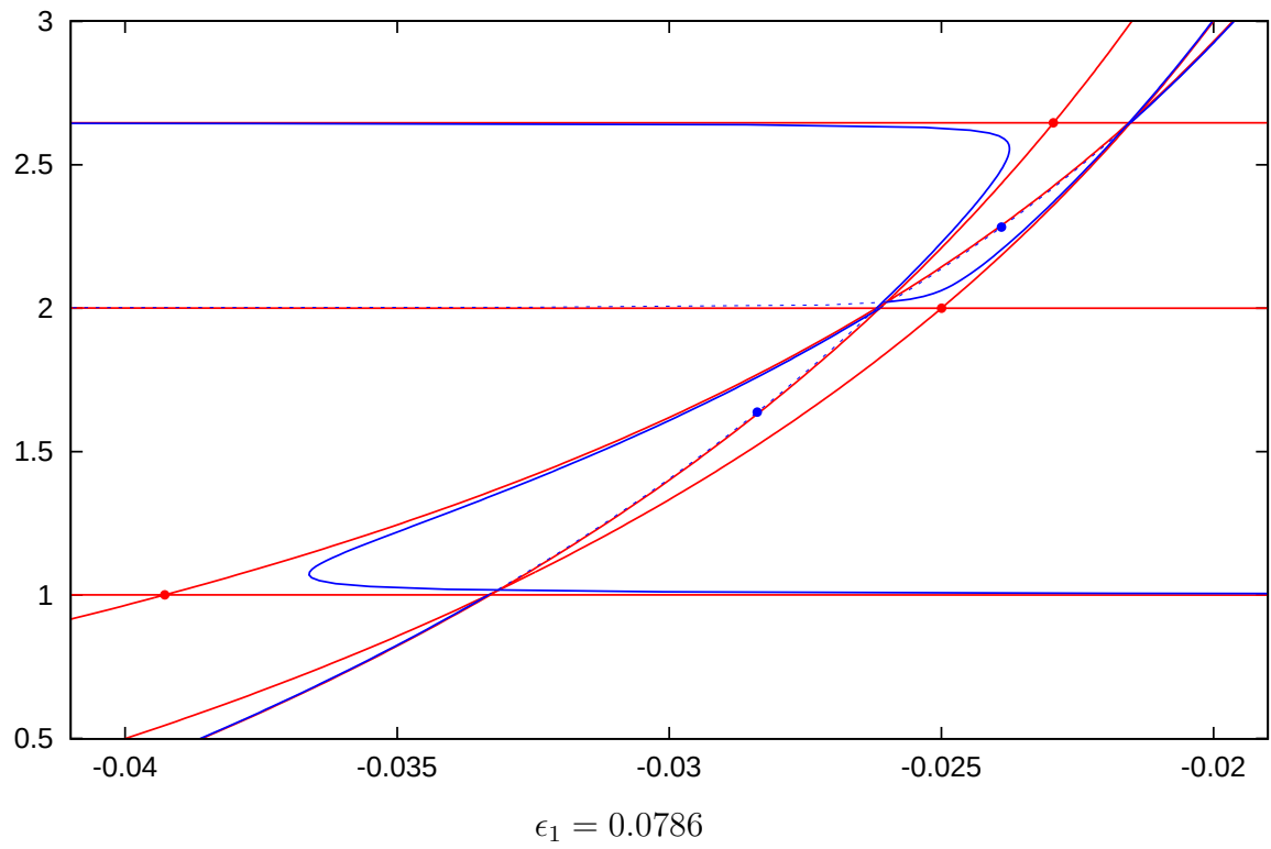
Figure 22: Change of Stokes geometry for Examples 2 as \epsilon_1 = 0.0784 \rightarrow 0.0786 with \epsilon_2 = 0.1 . A part near t = 2i is enlarged. (As in Figure 21, overlapping Stokes curves are designated by blue for \epsilon_1 = 0.078483 and \epsilon_1 = 0.078484 .)
