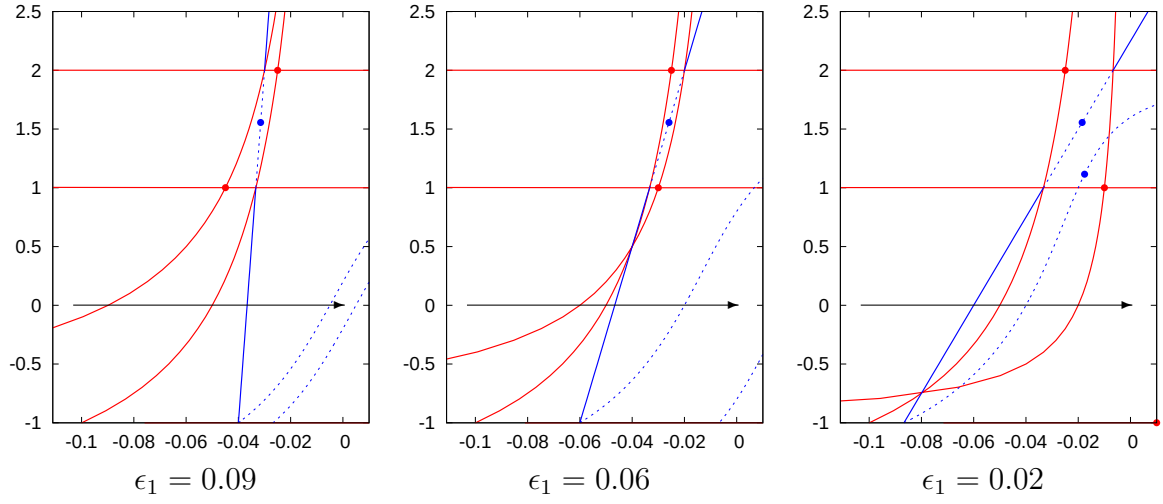
Figure 13: A part of the Stokes geometry of Example 1 with \epsilon_1 = 0.09, 0.06 and 0.02
