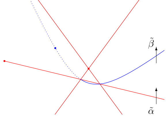
Figure 9: Stokes geometry for a = a_1 .
