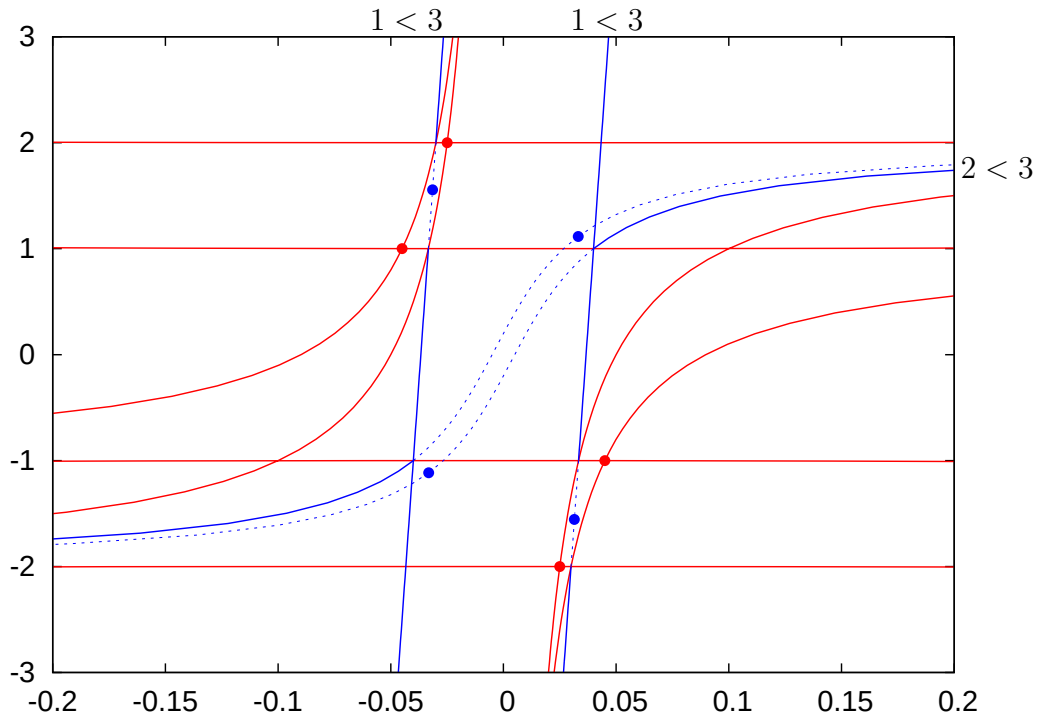
Figure 3: Stokes geometry for Example 1 with \epsilon_1 = 0.09 and \epsilon_2 = 0.1 .
