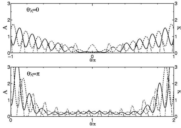
FIG. 7. Stabilizing term \mathcal{A} with M\alpha=0 (solid lines) and M\alpha=\pi (dashed lines) and the destabilizing term \mathcal{K}(>0) (dash-dotted lines) with M\alpha=0 , for (s, \theta_k) = (0.66, 0) (upper) and (s, \theta_k) = (0.52, \pi) (lower) cases for the broad pressure profile equilibrium at \beta_0 = 4.0\% .
