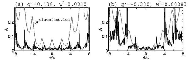
FIG. 12. Stabilizing term \mathcal{A} with the same input (s, \theta_k, M\alpha) = (0.6, 0, 0) for the broad pressure profile as in Fig. 11(b) except for q' changed artificially. (a) Taking q' = 0.138 which is the same value as in Fig. 11(a). (b) Taking q' = -0.330 which is the inverse sign of that in Fig. 11(b).
