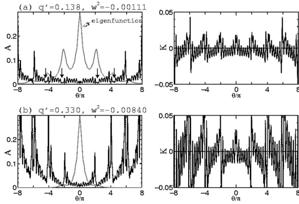
FIG. 11. Associated quantities along the field line; the stabilizing term \mathcal{A} (left) and the possibly destabilizing term \mathcal{K} (right) at \beta_0 = 1.2\% . (a) (s, \theta_k, M\alpha) = (0.5, 0, 0) for the peaked pressure profile. (b) (s, \theta_k, M\alpha) = (0.6, 0, 0) for the broad pressure profile. The q' values shown are proportional to global shear, s_* \propto -q' . The reductions of the integrated local shear in the field line tension \mathcal{A} , pointed by arrows are realized more clearly in (a) with small global shear and the eigenfunction uprise there. In the case of (b) with larger shear, the mode structure is more localized.
