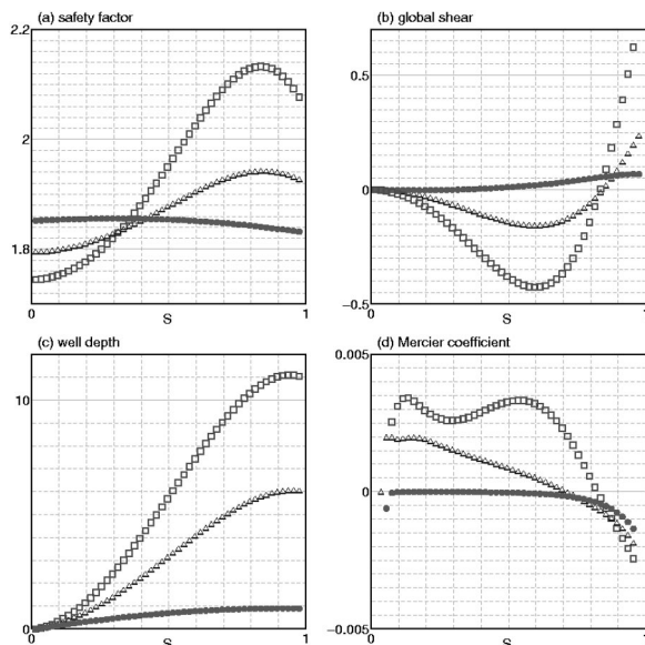
FIG. 3. Radial dependence of the equilibrium quantities for the broad pressure profile, (a) safety factor, (b) global shear, (c) well depth, (d) Mercier coefficient with central beta value \beta_0 = 0.0\% (circles), \beta_0 = 1.0\% (triangles), \beta_0 = 2.0\% (squares), as a function of s .
