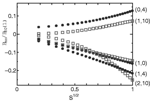
FIG. 2. Radial dependence of B_{mn} normalized by B_{00} at plasma edge, as a function of s^{1/2} . Not only Heliotron-J (circles) but also LHD (squares) case at \beta_0 = 0.0\% are shown for comparison.
