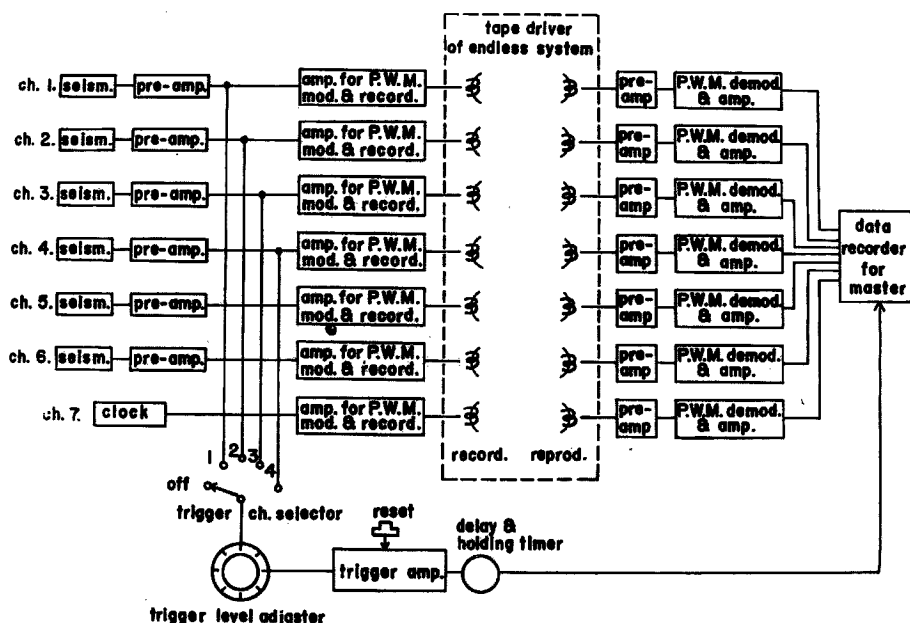
Fig. 1 Block diagram of the automatic data-recorder.
