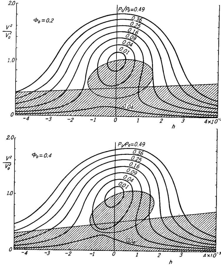
Fig. 7. h-V^2 diagrams for the cases \phi_0=0.2 and 0.4 . As a parameter P_1/P_0 is used instead of E . The hatched regions correspond to unstable states. These diagrams are drawn for the assumed values: Q_a=Q_{\text{ext}}=500 , X=1.84 (when \phi_0=0 ), M^2=0.5 , n=2 , V_b=300 and \nu=0.1058 .
