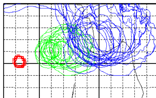
Fig. 5 Spaghetti diagram of sea level pressure of NHM. Each contour shows 1000 hPa in each ensemble member. Red: initial time. Green: t=24 h. Blue: t=48 h.
