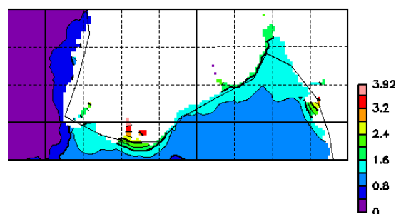
Fig. 3 Maximum sea surface height simulated by POM and computed using all the ensemble members and all the time steps.
