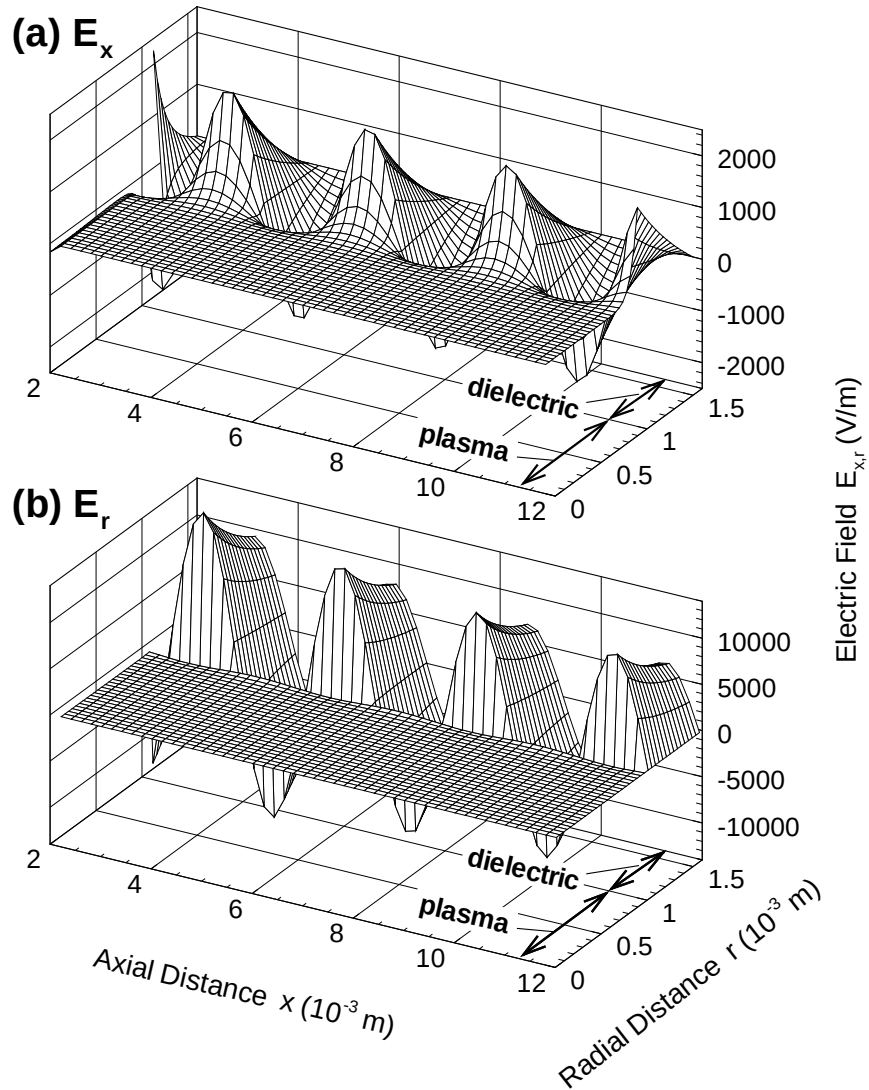
Figure 2.8: Typical snapshots of the two-dimensional distribution of the (a) axial and (b) radial electric field components of E_x and E_r in the plasma chamber, taken at the time when the electric fields reach the peak values in a microwave period. Here the calculation conditions are the same as those of Fig. 2.7(c).
