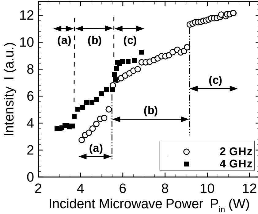
Figure 4.6: Emission intensity (Ar I 763.5 nm) as a function of incident microwave power P_{\text{in}} = P_t - P_{\text{rf}} for different microwave frequencies f = 2 and 4 GHz, otherwise measured under the same conditions as in Fig. 4.5.
