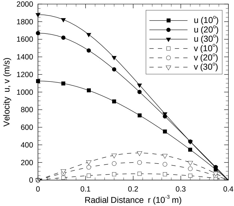
Figure 2.20: Radial distribution of the axial velocity u and radial velocity v at the nozzle exit, for different half-cone angles of (a) 10^\circ , (b) 20^\circ , and (c) 30^\circ in Fig. 2.17.
