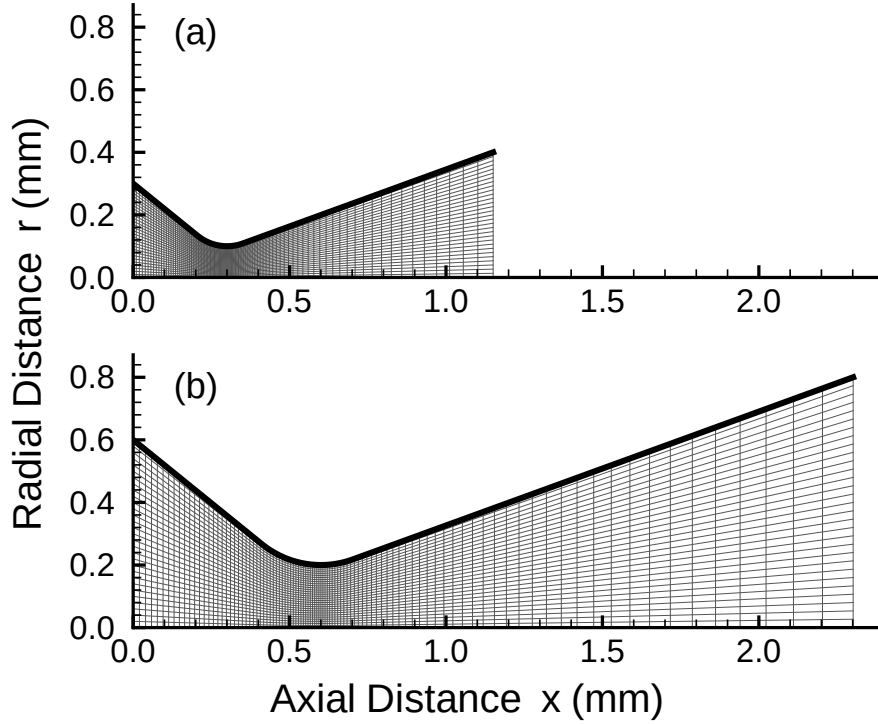
Figure 4.13: Cross-sectional view and computational grid for micronozzles with a 20^\circ -half-cone-angle isothermal wall ( T_{\text{wall}} = 300 \text{ K} ). The radii of the nozzle inlet, throat, and exit are set at 0.3, 0.1, and 0.4 mm, respectively, in (a), while the twice of them with the same aspect ratio in (b). The computational domain of both nozzles is divided into 100 cells in the axial direction and 30 cells in the radial direction.
