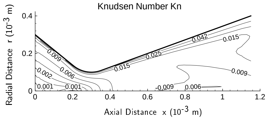
Figure 2.21: Distribution of the Knudsen number Kn in the micronozzle under isothermal wall conditions of the 20^\circ -half-cone-angle micronozzle, calculated at an absorbed power P_{\text{abs}} = 5.0 W and a pressure p = 1.0 \times 10^5 Pa in the microplasma source. Here, the inlet conditions are the same as those in Fig. 2.11.
