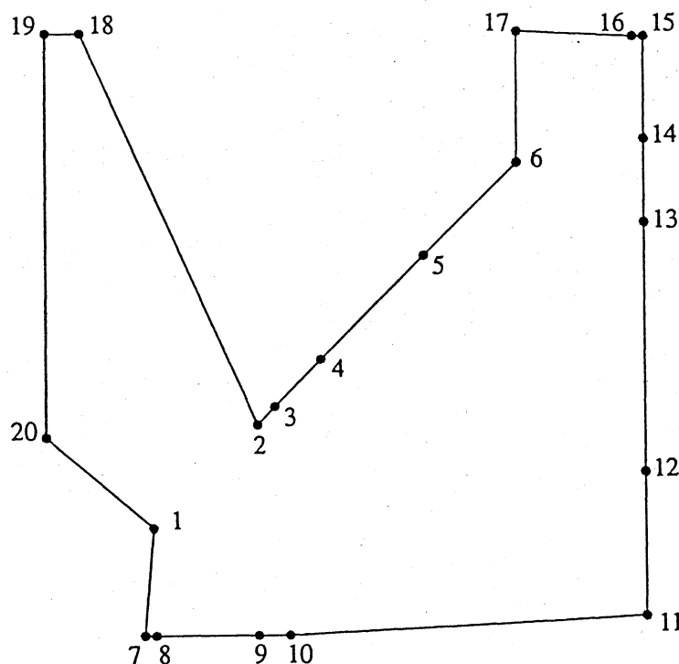
Figure 2: An instance of the convex-hull-and-line TSP and its solution.
