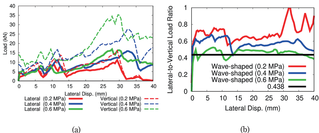
Fig. 9 Test results for the wave-shaped block wall: (a) load-displacement relationship; (b) relationship between the lateral-to-vertical load ratio and lateral displacement.
