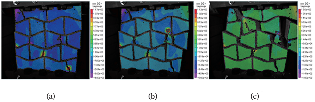
Fig. 11 Failure process and strain contour in the lateral direction of the wave-shaped block wall with an initial vertical stress of 0.4 \text{ N/mm}^2 : (a) lateral displacement of 18 mm; (b) lateral displacement of 33 mm; (c) lateral displacement of 36 mm.
