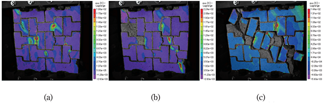
Fig. 8 Failure process and strain contour in the lateral direction of the I-shaped block wall with an initial vertical stress of 0.6 \text{ N/mm}^2 : (a) lateral displacement of 8 mm; (b) lateral displacement of 12 mm; (c) lateral displacement of 36 mm.
