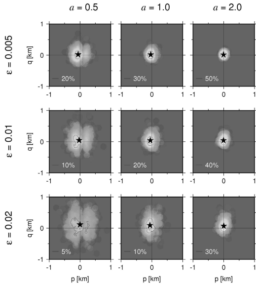
Fig. 3 Cross-sections of the stochastic tubes for each structure. The background structure, the source point and the receiver station are the same as in Fig.2. Anomalies are calculated for perturbations of a = 0.5, 1.0 and 2.0 km and \varepsilon = 0.005, 0.01 and 0.02 . The cross-section planes are perpendicular to the reference ray path at the turning point. p - and q -axes include transverse and vertical components from the receiver point of view, respectively. In these cases, unit vectors p/|p| and q/|q| are (0, 1, 0) and (0, 0, -1) , respectively. The origin is identical with the reference ray path. The probability for an arbitrary point is estimated by the ratio of the number of stochastic paths included in the arbitrary point centered circle of 0.1 km radius, to the total number of samples ( d = 1,000 ). Stars show the expectation values in each cross-section. The grayscale of probability is identical with that in Fig.2.
