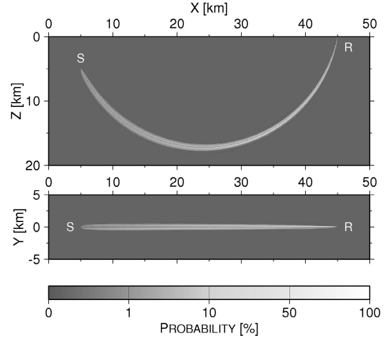
Fig. 2 Stochastic tube for a reference ray of the first arrival P-wave projected onto the XZ -plane and the XY -plane. X and Y are horizontal coordinates and Z is the vertical, which form a left-hand system. The probability indicates the ratio of stochastic paths through each 0.05 \times 0.05 \text{ km}^2 square in the projected planes, to the total number of samples ( d = 1,000 ). The light region indicates high probability and the gray low probability. S and R are the source point (5, 0, 5) and receiver station (45, 0, 0), respectively. The background velocity is 0.25Z + 1 \text{ km/s} and its perturbation is characterized by the exponential ACF with a = 0.5 \text{ km} and \varepsilon = 0.01 . The solid line in the stochastic tube is the reference ray path.
