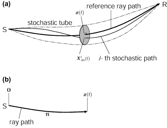
Fig. 1 (a) Geometry of a stochastic tube. A seismic source and a receiver station are represented as S and R, respectively. The reference ray path connects S and R. X_{stc}^i(t) is the intersection of the i -th stochastic path in a cross-section perpendicular to x(t) in the reference ray path for time t . A stochastic tube is constructed by the bundle of d stochastic paths. (b) Position vector x(t) in the ray path. S is both the source point and the origin of the vector. n is the tangent vector along the ray path.
