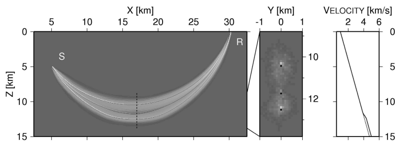
Fig. 5 Stochastic tube for the reference ray in the case of a triplication. The left figure is the tube projected onto the XZ-plane, where solid curves are multiple ray paths of the triplication. The middle figure is the magnified tube crossing the YZ-plane, which is also illustrated with a vertical broken line in the left figure. Small filled circles indicate the cross sections of the multiple reference ray paths. In the right portion, the background velocity structure is shown with a solid line, indicating that the velocity suddenly but smoothly increases beneath a certain depth. The perturbation is characterized by the exponential ACF with a = 1.0 km and \varepsilon = 0.01 . The total number of samples is d = 3,000 . The grayscale of probability is identical with that in Fig.2.
