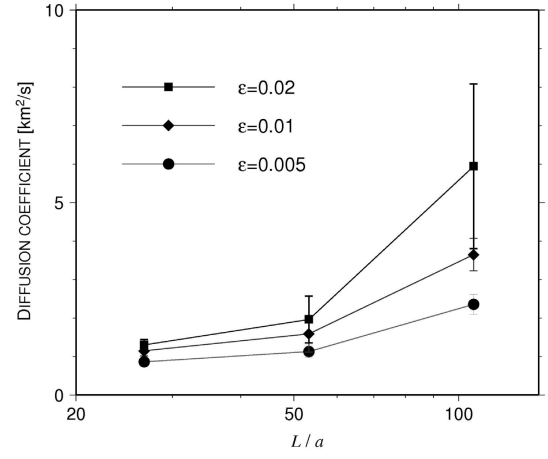
Fig. 4 Diffusion coefficients of stochastic tubes for each media of a and \varepsilon indicated in Fig.3. L is the travel distance of the reference ray. The diffusion along the vertical component (or q -axis) is always larger than lateral component (or p -axis). The bars show differences of the diffusion between the major axis and the minor axis of the elliptical shape in the cross-section.
