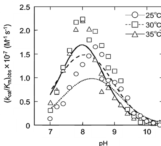
Fig. 11. Effect of pH on human RNase H2 activity. (A) Reaction scheme with two ionizable groups responsible for activity. (B) (k_{cat}/K_m)_{obs} vs. pH. The reaction was carried out at 25 (open circle), 30 (open square), and 35°C (open triangle), each with the initial enzyme and R1/D18 concentrations of 300 pM and 5.6 nM, respectively. Solid line represents a curve expressed by Eq. 1 with the (k_{cat}/K_m)_0 value and the pK_{e1} and pK_{e2} values of (1.2 \pm 0.3) \times 10^7 M^{-1} s^{-1} , 7.4 \pm 0.3 , and 9.2 \pm 0.3 , respectively, for 25°C, (1.9 \pm 0.5) \times 10^7 M^{-1} s^{-1} , 7.2 \pm 0.4 , and 8.9 \pm 0.3 , respectively, for 30°C, and (2.9 \pm 0.7) \times 10^7 M^{-1} s^{-1} , 7.5 \pm 0.2 , and 8.5 \pm 0.2 , respectively, for 35°C, which was drawn to fit the experimental data.
