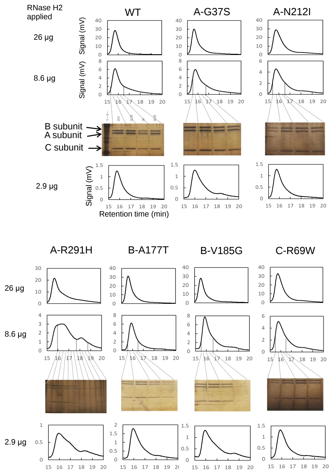
Fig. 7. Elution patterns of gel filtration column chromatography of human RNase H2 variants. WT and variants (26, 8.6, or 2.9 µg) were applied onto the column. Silver-stained 12.5% SDS-polyacrylamide gel is also shown.
