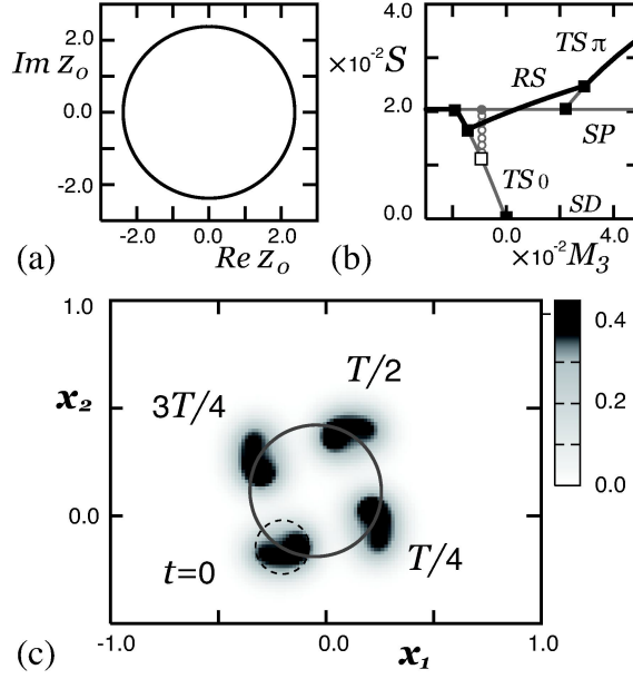
Figure 1: (a) 1:2 mode interaction in a rotational spot (RS) motion for ODE of (9). (b) Bifurcation diagram of spot solutions for the ODEs of (10), where N_3 is fixed to 0.1. Stable RS motion appears via pitchfork bifurcations and connects between the TS_0 and TS_\pi branches. (c) Rotational spot (RS) motion in the PDE system: A spot moves in a counterclockwise direction as observed in four superimposed snapshots. The trajectory of the the centroid of v -component distribution is depicted by the solid line.
