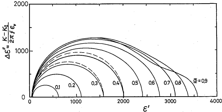
Fig. 2. Complex plane plots of complex relative permittivity for suspensions of shell-spheres calculated from Eq. (2) (solid curves). The dashed curves are semicircles. Phase parameters used: \epsilon_a=80 , \kappa_a=\kappa_i=2.5 mS cm -1 , \epsilon_i=50 , \epsilon_s=6.5 , \kappa_s=0 mS cm -1 , d=50 Å, D=3.8 μm.
