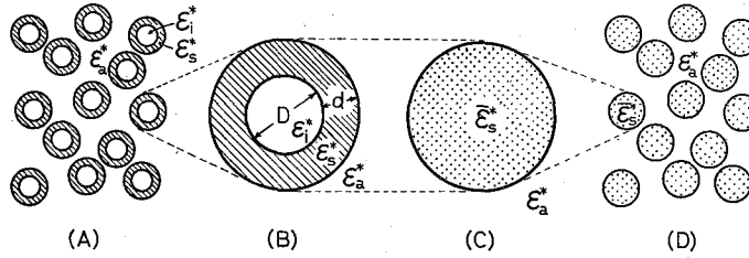
Fig. 1. Schematic diagram for a theoretical model of a concentrated suspension of shell-spheres. (A) Concentrated suspension of spheres ( \epsilon_i^* ) covered with a shell phase ( \epsilon_s^* ) dispersed in a continuous medium ( \epsilon_a^* ). (B) Shell structure of a suspending particle. (C) A homogeneous sphere ( \bar{\epsilon}_s^* ) as an equivalent of the shell sphere shown in (B). (D) Concentrated suspension of particles ( \bar{\epsilon}_s^* ) dispersed in a continuous medium ( \epsilon_a^* ) as an equivalent of the suspension shown in (A).
