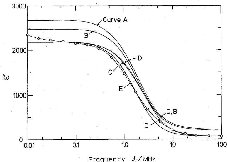
Fig. 3. Frequency dependence of relative permittivity and conductivity for a bovine erythrocyte suspension and the procedure of curve-fitting. The hollow circles (—○—) are the measured values. The curves A, B, C, D, and E correspond to Steps 1, 2, 3, 4, and 5 in Table II, respectively. The observed values for the outer medium are: \epsilon_a=77.1 , \kappa_a=4.346 \text{ mS cm}^{-1} .
