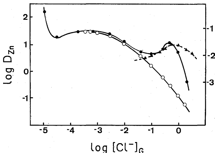
Fig. 1. Distribution of zinc as a function of chloride concentration. \text{Zn}^{2+} ; 10^{-6}\text{M} , TOPO; 0.1M in decaline, temp.; 25°C ●; HCl in diethylene glycol, ○; LiCl ( [\text{H}^+] = 4 \times 10^{-4}\text{M} ), ▲; distribution of HCl.
