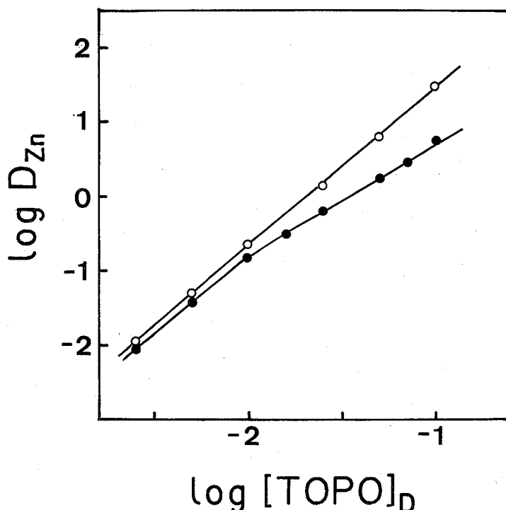
Fig. 3. Distribution of zinc as a function of TOPO concentration. [H^+] ; ○ 3.0 \times 10^{-4} M, ● 0.18M, initial chloride concentration; 9.7 \times 10^{-4} M.
