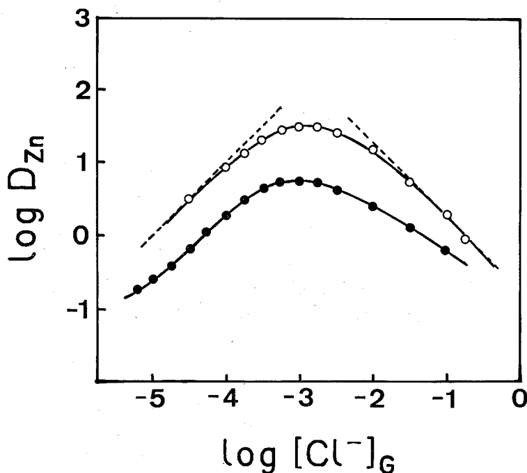
Fig. 2. Log D_{Zn} vs. log [Cl^-]_G plots at a constant hydrogen ion concentration. [H^+] ; ○ 3.0 \times 10^{-4} M , ● 0.18M, ionic strength; 0.18, H_2O ; 0.7 V% in diethylene glycol. Others are the same to those in the Fig. 1.
