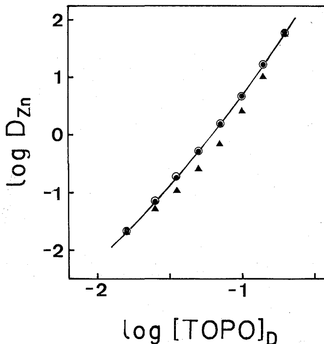
Fig. 5. \log D_{Zn} vs. \log [\text{TOPO}]_D plots. ○; observed, ●; calculated from Eq. 5 as y=4 , ▲; calculated as y=5 .
