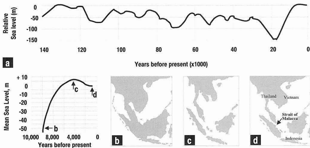
Fig. 3. a) Sea level fluctuation over the past 140,000 years ago (Potts 1983). b), c) and d) Sea levels and topographies of SPouth East Asia during 8000, 4000 years ago and at present, respectively (modified from Lekagul and McNeely 1977; Geyh et al. 1979).
