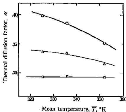
Fig. 7. Thermal diffusion factor as a function of mean temperature of x_2 = .561 at various pressures:
