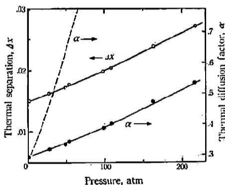
Fig. 8. Thermal separation and thermal diffusion factor as a function of pressure:
