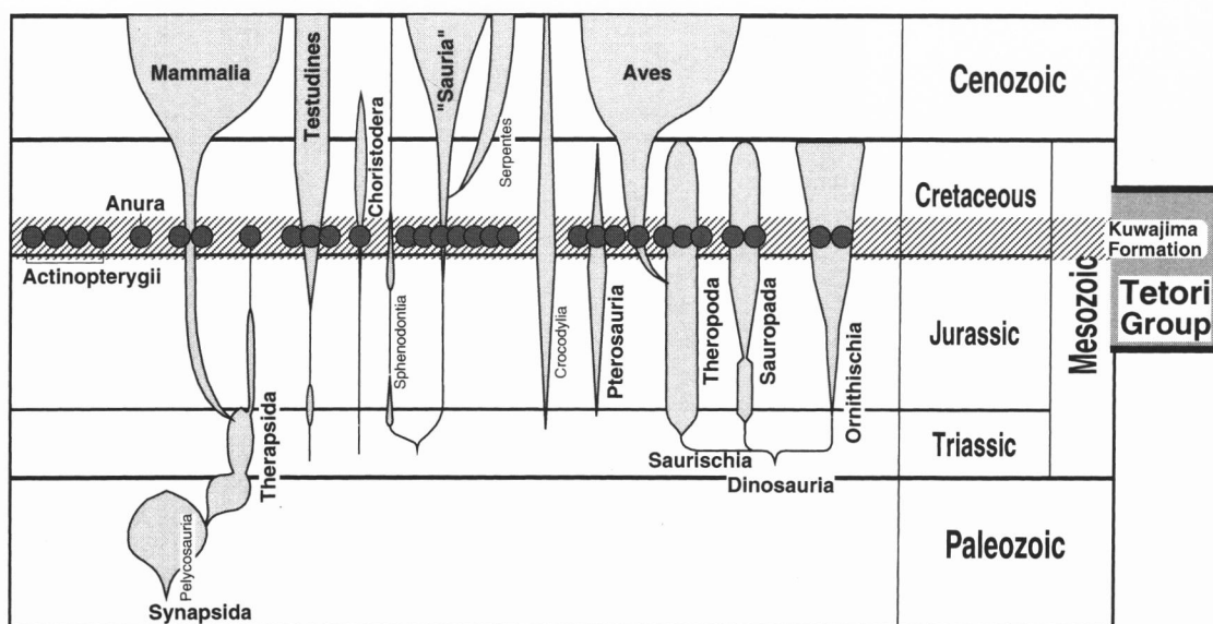
Fig. 3. Taxonomic composition of the vertebrate assemblage of the Kuwajima "Kaseki-kabe". Circles showing the collected taxa.
