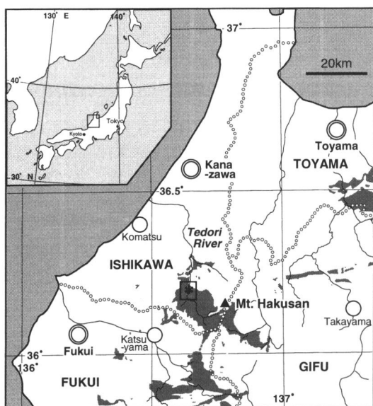
Fig. 1. Main distribution of the Tetsu Group (modified after Maeda, 1961e). Asterisk showing the position of Shiramine Village, Ishikawa Prefecture.
