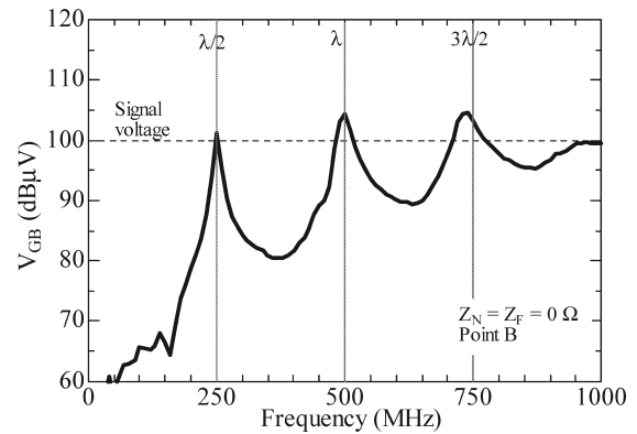
(b) Measured guard-trace voltage at point B.
