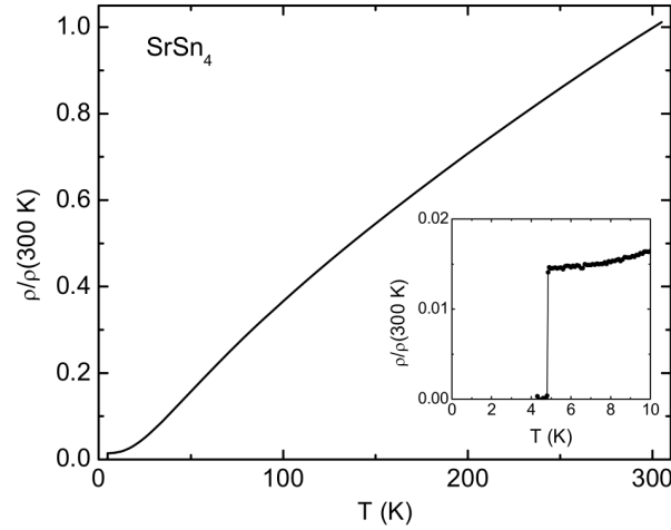
Figure 2.4: The temperature-dependent, normalized resistivity of \text{SrSn}_4 [63]. Inset: low temperature data showing the superconducting transition.
