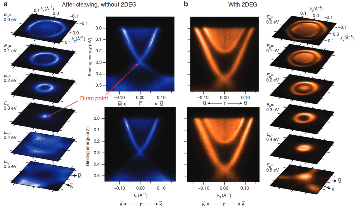
Figure 1.4: Development of a surface 2DEG in \text{Bi}_2\text{Se}_3 [41]. (a) Electronic structure of \text{Bi}_2\text{Se}_3 approximately 30 minutes after cleaving the sample. The Dirac-like dispersion of the topological surface state is clearly shown. (b) After three hours in vacuum, the chemical potential shifted, probably due to defect formation. The sharp rim around the conduction band is the spectral signature of the 2DEG near the surface in real space.
