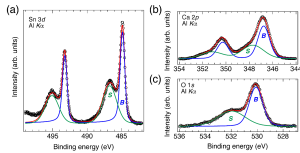
Figure 2.17: (Color online) XPS spectra from the \text{Ca}_3\text{SnO} film for (a) \text{Sn-}3d , (b) \text{Ca-}2p , and (c) \text{O-}1s core levels. The fitting results are overlaid by green, blue, and red curves, which correspond to the surface component (S), bulk component (B), and their summation, respectively [75]
