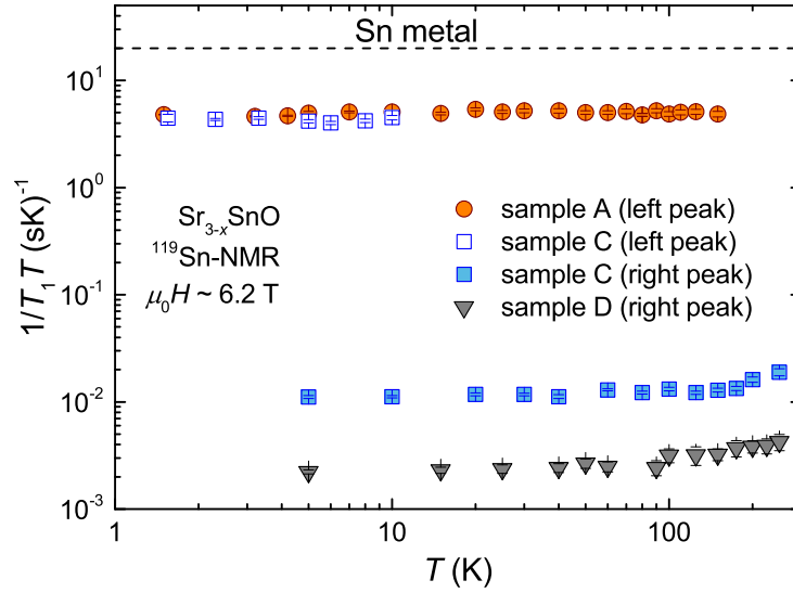
Figure 7.5: Temperature dependence of 1/T_1T at different positions and samples, which is plotted on a logarithmic scale. 1/T_1T was measured around 6.2 T. The broken line represent the value of 1/T_1T on Sn metal. [Figures by S. Kitagawa]
