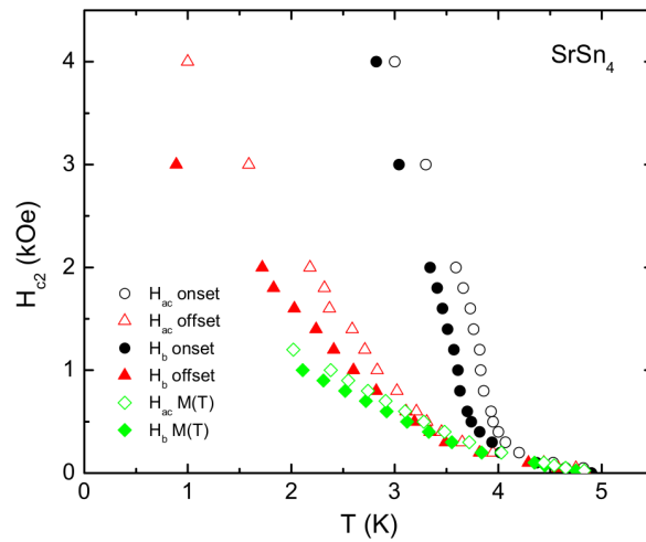
Figure 2.5: Anisotropic upper critical field of \text{SrSn}_4 from magnetization and magnetotransport measurements [63].
