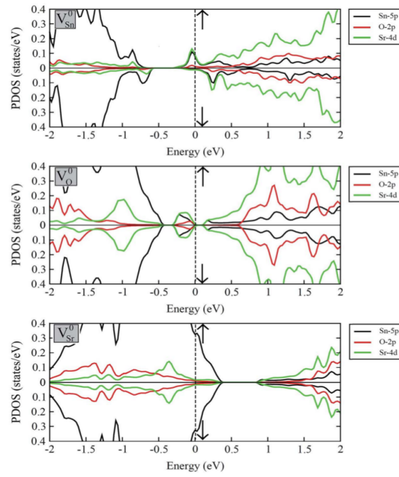
Figure 2.10: The spin-polarized partial DOS plots of V_{\text{Sn}}^0 , V_{\text{O}}^0 and V_{\text{Sr}}^0 containing 2 \times 2 \times 2 superlattice of \text{Sr}_3\text{SnO} calculated with the inclusion of SOC. The majority and minority spin channels are represented by up and down arrows, respectively. [65]
