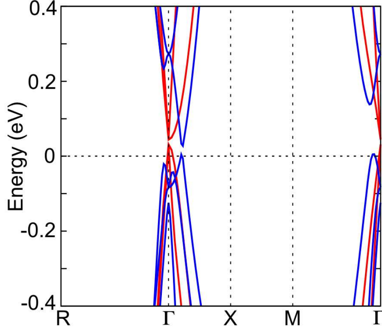
Figure 5.11: Band structures of \text{Sr}_3\text{SnO} in the first principles calculation carried out with the WIEN2k package [78] (blue line) and the Vienna ab-initio simulation package (VASP) [109, 110, 111] (red line) [1]. Spin-orbit coupling is included in both calculations. For calculations with the WIEN2k package, the Perdew-Burke-Erzerhof generalized-gradient approximation [82] is used for the exchange-correlation function. The parameter (RK_{\text{max}}, G_{\text{max}}) = (9.0, 14.0) [112] are chosen, and 20 \times 20 \times 20 momentum points in the irreducible Brillouin zone are used in the self-consistent cycle. The crystal parameters are taken from the experimental results [14]. The radii of the spherical atomic regions for Sr, Sn, O are chosen to be 2.33, 2.50, and 2.33 (a.u.), respectively. In the band structure obtained with the VASP, the Heyd-Scuseria-Ernzerhof (HSE) screened Coulomb hybrid density functionals [113] are employed to improve the underestimation of band gap. Besides, the projector augmented-wave potential [114, 115] and the 5 \times 5 \times 5 Monkhorst-Pack grid are used. The energy cutoff of the plane wave basis is 400 eV, and we performed structural relaxations with forces converged to less than 0.001 \text{ eV/\AA} . We note that for \text{Sr}_3\text{SnO} the band spectrum generated using the WIEN2k package is very different from that in ref. 5, where the HSE screened Coulomb hybrid density functionals were employed in the first principles calculation. First, details of the band structure near the \Gamma point are substantially different. Second, there is no hole FS around the R-point, whereas it is present in the result of ref.5. In contrast, the band spectrum generated using the VASP with the HSE method almost reproduces the band spectrum in ref. 5 near the \Gamma point, despite that there is no hole FS around the R-point again. Such method-dependence was discussed before by Vidal et al. [116], which concludes that the HSE method is more reliable. Thus we adopt the HSE result to parameterize our tight-binding band structure near the \Gamma point to obtain the orbital texture (Fig. 5.3 and Fig. 5.12).
