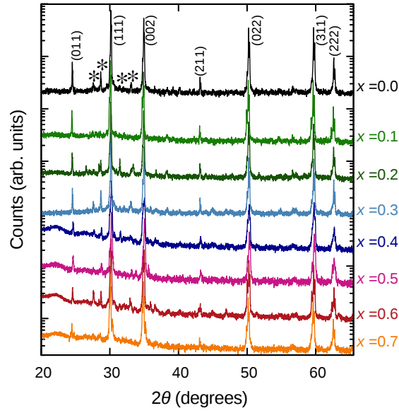
Figure 6.1: Powder XRD pattern of \text{Sr}_{3-x}\text{SnO} with various nominal values of x plotted on a log scale. Minor impurity peaks from SrO phase are seen on the left of (111) and (002) peaks of the main phase. Additional weak impurities can be seen between the (011), (111), and (002) peaks.
