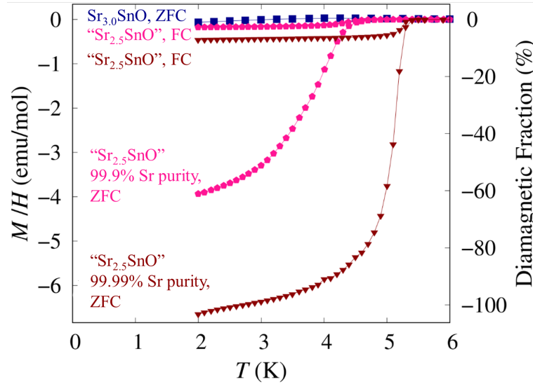
Figure 4.7: Magnetization under zero field cooling (ZFC) with an applied field of 2 mT of \text{Sr}_3\text{SnO} of Sample B-1 (blue square), and under ZFC as well as field cooling (FC) of \text{Sr}_{2.5}\text{SnO} of Sample B-2 (pink pentagon) and Sample B-3 (brown triangles) [2]. The vertical scale on the right indicates the estimated diamagnetic volume fraction without demagnetization correction. Stoichiometric \text{Sr}_3\text{SnO} is not superconducting. The superconducting volume fraction of \text{Sr}_{2.5}\text{SnO} increases significantly with increased purity of the strontium raw material.
