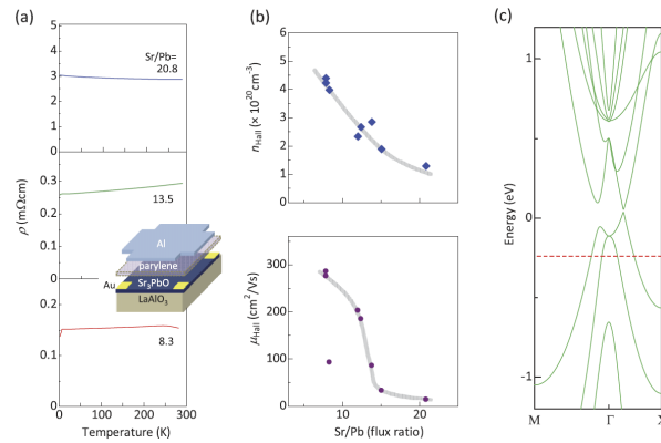
Figure 2.16: (a) Temperature dependence of resistivity for \text{Sr}_3\text{PbO} films grown with different Sr/Pb flux ratio. The inset in the middle panel shows schematic structure of \text{Sr}_3\text{PbO} film with contacts and capping layers. (b) At 10 K, n_{\text{Hall}} (top panel) and \mu_{\text{Hall}} (bottom panel) versus Sr/Pb flux ratio. Gray solid lines are guide to the eye. (c) Band diagram based on first-principles calculation (green solid line) and estimated position of E_F using an input from n Hall (red dashed line) [74].
