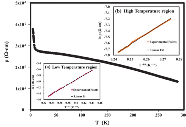
Figure 2.15: Resistivity as a function of temperature (5 K-285 K). Bottom left inset (a): \ln \rho vs. T^{-1/2} at low temperature (5-10 K). Top right inset (b): \ln \rho vs. T^{-1/4} at high temperature (170-285 K) along with best fit results obtained by least-square fitting [66].
