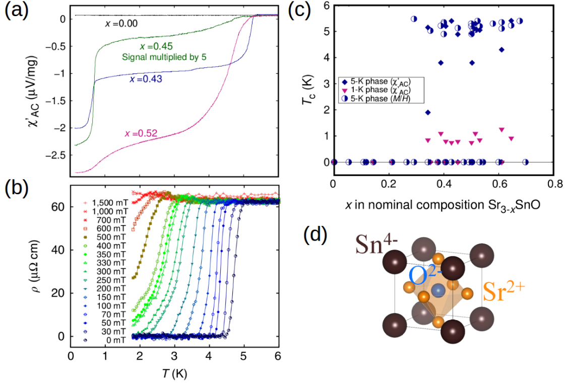
Figure 8.1: (a) \chi_{AC} of \text{Sr}_{3-x}\text{SnO} with various x , showing transitions at 5 and 1 K. (b) Resistivity of \text{Sr}_{3-x}\text{SnO} at low temperature under different magnetic fields. (c) T_c of 5 and 1 K phases as a function of x in “ \text{Sr}_{3-x}\text{SnO} ”. (d) Crystal structure of \text{Sr}_3\text{SnO} with oxidation state of ions. Figure produced with VESTA [16].
