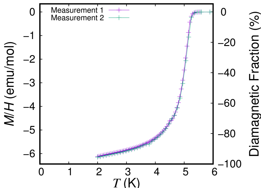
Figure 6.2: DC magnetization measured at 10 Oe as a function of temperature of a \text{Sr}_{2.5}\text{SnO} sample (Batch No. AP164). Degaussing was performed between the two measurements, both reproducibly showing strong superconducting 5-K phase, close to 100% volume fraction. Demagnetization correction was not done. After these measurements, the remnant field was checked using a reference superconductor (Pb, 99.9999% purity) and found to be below 1 Oe.
