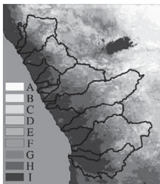
Fig. 1. Nine classes resulted from the ISODATA classification.
