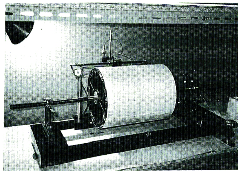
Photo. 2. Pen-drum recorder.
