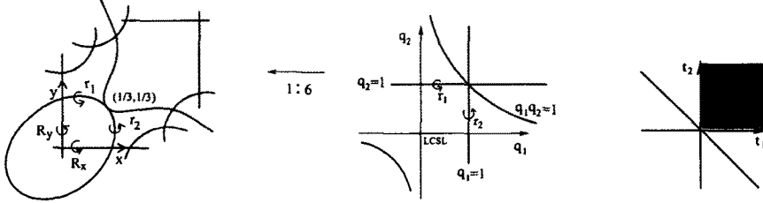
Fig.2. The discriminant dis(x,y) = 0 in \hat{\mathcal{M}}_{Sec(\Sigma)} (left), the mirror map to q_1q_2 -plane (3.5)(middle), and the complexified Kähler moduli t_1, t_2 with the complexified Kähler cone (right). The discriminant is an elliptic curve with a node at (x,y) = (\frac{1}{3}, \frac{1}{3}) , which is mapped to (q_1, q_2) = (1, 1) . The mirror map is 1 : 6 at generic (x,y) . Over the discriminant, it is 1 : 3 and represented by the three lines q_1 = 1, q_2 = 1, q_1q_2 = 1 in the q -plane.
