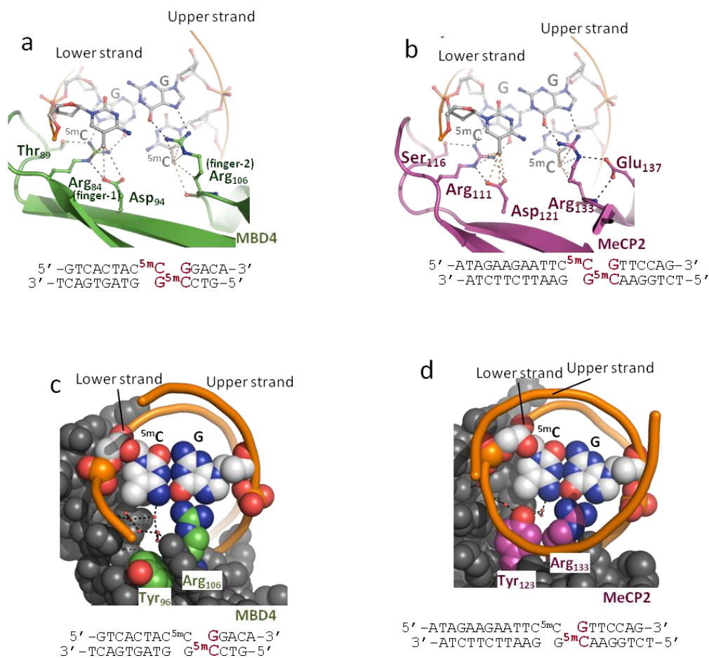
Figure 2. (a, b) The close up views of the DNA binding interface of the \text{MBD}_{\text{MBD4}}\text{-}^{5\text{m}}\text{CG}/^{5\text{m}}\text{CG} complex (a) or \text{MBD}_{\text{MeCP2}}\text{-}^{5\text{m}}\text{CG}/^{5\text{m}}\text{CG} complex (b). The CpG bases (shown in red in the DNA sequence, below) and amino acid residues involved in the base recognition are shown in the stick models. The dotted line in black and orange indicate the hydrogen bond ( \sim 3.2 Å) and the van der Waals interaction ( \sim 4.2 Å), respectively. The arginine finger-1 or finger-2 contact with lower or upper strand ^{5\text{m}}\text{CpG} step, respectively. (c, d) Space filling representation of the protein-DNA interface of the \text{MBD}_{\text{MBD4}}\text{-}^{5\text{m}}\text{CG}/^{5\text{m}}\text{CG} complex (c) or \text{MBD}_{\text{MeCP2}}\text{-}^{5\text{m}}\text{CG}/^{5\text{m}}\text{CG} complex (d). The ordered water molecules are shown as red balls and hydrogen bonds between water molecules are shown as black dotted lines. There is a cavity on the \text{MBD}_{\text{MBD4}}\text{-DNA} interface because of the difference in the side chain conformation of Tyr96.
