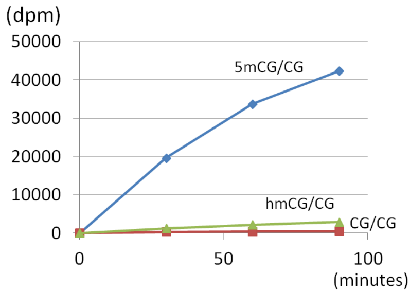
Figure 6. The DNA substrate specificity of maintenance DNA methyltransferase, Dnmt1. Radio-activities incorporated into the substrate DNA fragments after incubation for 30, 60 and 90 minutes were analyzed. The ratio of reaction rate for the 5mCG/CG and hmCG/CG substrates was estimated to be about 10:1 from the slopes of the linear fitting curves.
