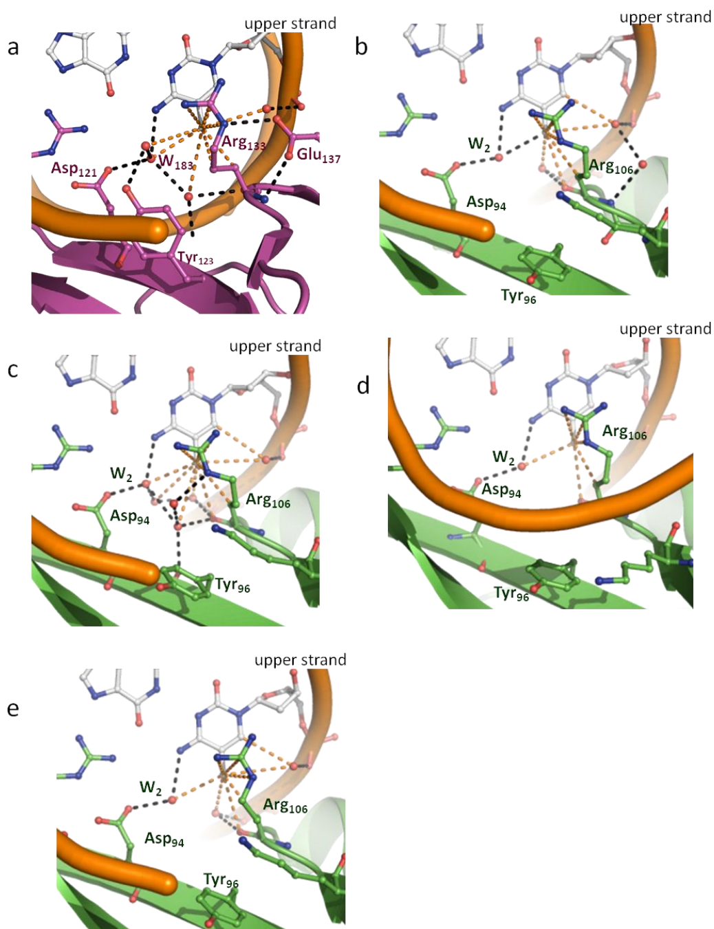
Figure S7. The close up view of the upper strand {}^5\text{mC} base recognition in the \text{MBD}_{\text{MeCP2}}\text{-}{}^5\text{mC}/{}^5\text{mC} complex (a) or \text{MBD}_{\text{MBD4}} in complex with {}^5\text{mC}/{}^5\text{mC} (b), 14bp- {}^5\text{mC}/\text{TG} (c), 11bp- {}^5\text{mC}/\text{TG} (d) or {}^5\text{mC}/{}^{\text{hm}}\text{C} (e). Hydrogen bonds ( \sim 3.2 Å) and van der Waals contacts or CH-O type hydrogen bonds ( \sim 4.2 Å) are represented in the black and orange dotted lines, respectively.
