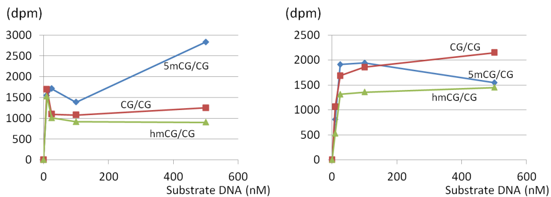
Figure 9. DNA-substrate dose dependency in the reaction of de novo DNA methyltransferases. The concentration of substrate DNA fragments were 0, 10, 25, 100 or 500 nM.
