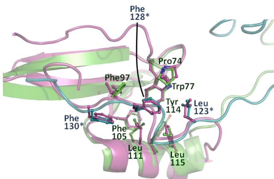
Figure S2. The structural alignment of the amino acid residues in the hydrophobic core of the MBD MBD4 and MBD MeCP2 . MBD MBD4 in the complex with 14-bp 5m CG/TG fragment is shown in green and the C-terminal part of the domain which comes from the symmetry related molecule is shown in cyan. MBD MeCP2 is represented in magenta. The hydrophobic core side chains of MBD MBD4 , Pro74, Trp77, Phe97, Phe105, Leu111, Tyr114, Leu115, Leu123, Phe128 and Phe130 and the corresponding amino acid residues of MBD MeCP2 are shown as a stick model.
