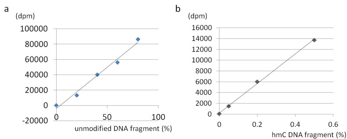
Figure 1. The representative linear calibration curves for the 5mC and hmC quantification assays. (a) The scintillation counts after SssI reaction for 200 ng of standard DNA samples, which are the mixtures of C and 5mC fragments at ratios of 0:1, 1:4, 2:3, 3:2, and 4:1. (b) The radio-activities of the filter papers after \beta GT assay for 200 ng of the C standard DNA spiked with 0, 0.1, 0.4 and 1 ng of the hmC standard fragment.
