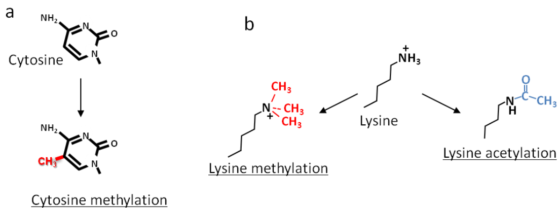
Figure 2. Examples of chemical modification of chromatin. (a) DNA methylation occurs at the C5 position of the cytosine ring. (b) The terminal amino group of the lysine side chain can be methylated and acetylated. Lysine methylation modifies protein-protein interactions and lysine acetylation alters surface property of the protein cancelling the positive charge of the lysine residue.
