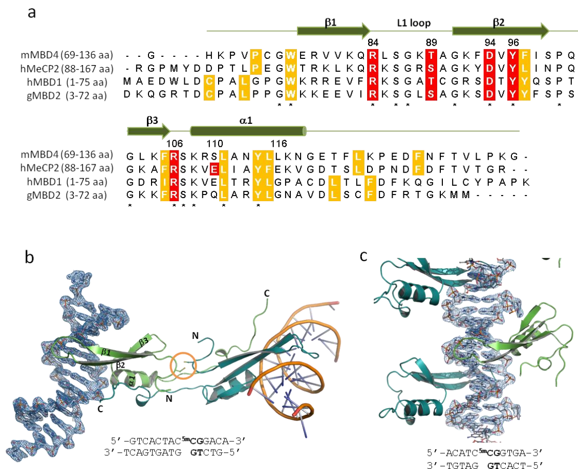
Figure 1. (a) The amino acid sequence alignment of structurally known MBD domains of mouse MBD4, human MeCP2, human MBD1 and chicken MBD2. The asterisks indicate that the residues are conserved among these MBD domains. The amino acid residues, highlighted in yellow, form hydrophobic core of the domain and the residues in red are involved in the recognition of the methylated CpG base pair.
