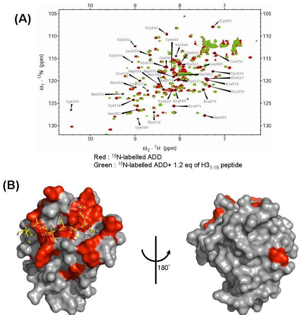
Fig. S5 | ^1\text{H} - ^{15}\text{N} chemical shift perturbation upon H3 peptide binding. (A) ^1\text{H} - ^{15}\text{N} HSQC spectra of free (red) and H3-bound ADD 3A (green). Residues that undergo chemical shift changes larger than 0.1 ppm in ^1\text{H} or 0.5 ppm in ^{15}\text{N} upon H3 binding are indicated with labels. (B) Surface representation of ADD 3A . Surface residues that exhibited large chemical shifts upon binding, labeled in A, are highlighted in red. The H3 peptide bound to ADD 3A in the fusion crystal is shown as stick model.
