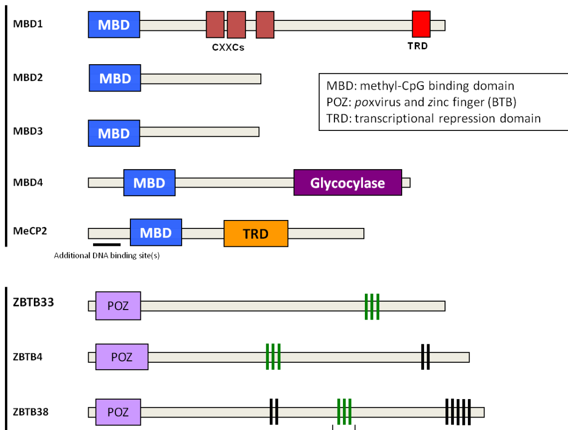
Figure 4. The domain structures of Methyl CpG binding proteins. MBD family proteins contain a conserved MBD domain. MBD1 has extra DNA binding motifs which can bind to unmodified CpG sequence. MBD1 and MeCP2 have a TRD where the amino acid sequence is not conserved. ZBTB33, ZBTB4 and ZBTB38 contain a conserved POZ domain involved in protein-protein interactions and three C2H2 zinc finger motifs, two of which are essential for binding to methylated DNA.
