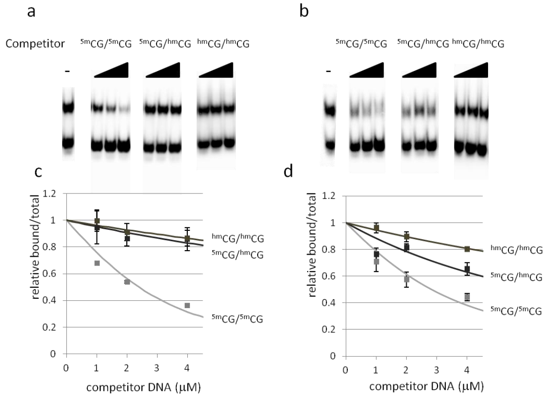
Figure S11. Competitive electrophoretic mobility shift assay using 5mCG/5mCG , 5mCG/hmCG or hmCG/hmCG sequence as a competitor DNA as shown in figure 4. (a, b) The representative autoradiographic images of the competition assay of MBD MBD1 (a) and MBD MBD4 (b). Each of the competitor DNA sequence is indicated above. (c, d) The bound to total ratios are quantified from gel band density and the values relative to the control lanes are plotted against the amount of competitor DNA. Each dots represent the average of three independent experiments using MBD MBD1 (c) or MBD MBD4 (d) with standard deviation. The solid lines represent the fitting curves using the Morrison's equation.
