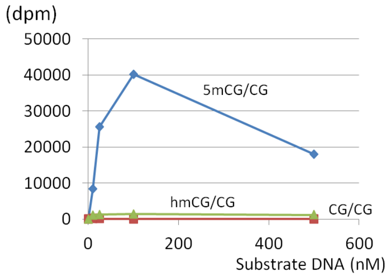
Figure 7. The substrate concentration dependence for Dnmt1 methyltransferase reactions with increasing amount of substrate DNA fragments at the concentration of 0, 10, 25, 100 or 500 nM.
