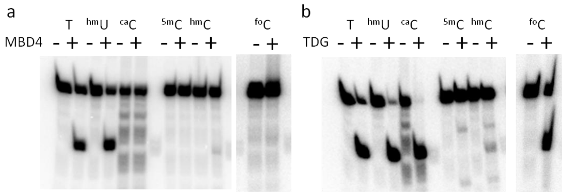
Figure 6. (a, b) The glycosylase assays toward a series of pyrimidine bases, T, hm U, ca C, 5m C, hm C and fo C, in the context of 5m CG/XpG sequence DNA using full-length MBD4 (a) or TDG (b) as an enzyme. The nucleotide sequences of the substrates for the assay are listed in Table S1.
