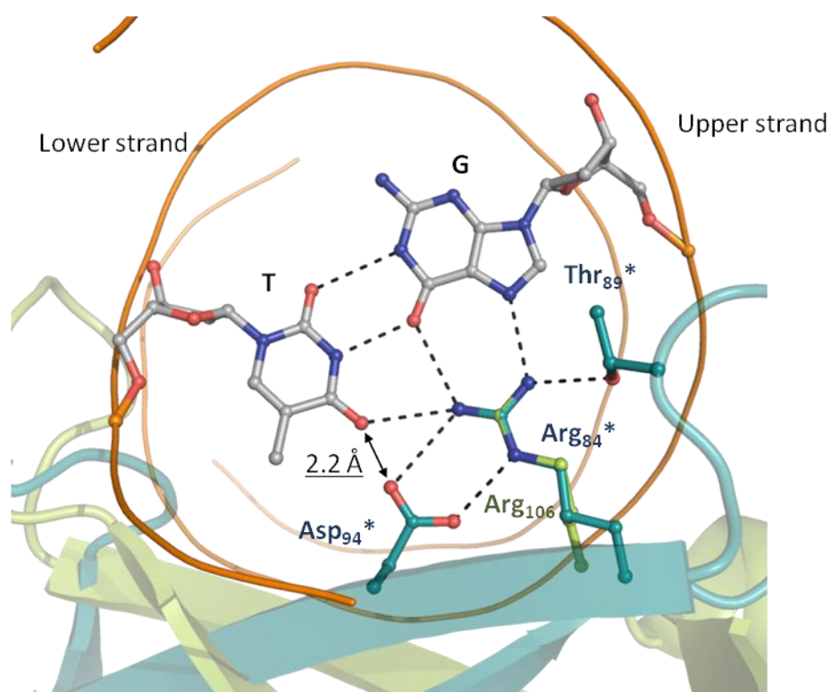
Figure S14. The structural model of the MBD domain of MBD4 bound to the 5m CG/TG sequence in the direction opposite to that observed in the crystal. The guanidino group group of Arg84 of the model molecule (colored in blue) is overlaid onto that of Arg106 in the MBD MBD4 - 5m CG/TG complex structure (colored in green). The steric clash between the carboxyl groups of the thymine base and the Asp94 is expected.
