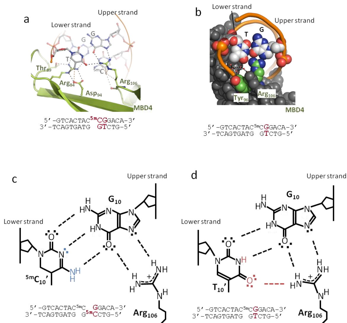
Figure 3. (a) The close up view of the DNA binding interface of the MBD MBD4 -5 m CG/TG complex similar to the figures 2a and 2b. The overall recognition mode of 5 m CG/TG sequence by MBD MBD4 is similar to that of 5 m CG/5 m CG sequence. (b) Space filling representation of the MBD MBD4 -5 m CG/TG interface similar to the figures 2c and 2d. The ordered water molecules are shown as red balls and hydrogen bonds between these water molecules are shown as black dotted lines. (c, d) Schematic diagrams of hydrogen bonding pattern of 5 m C/G (c) and T/G mismatch base pair (d). The structural elements specific to the 5 m C or thymine base is highlighted in blue or red, respectively.
