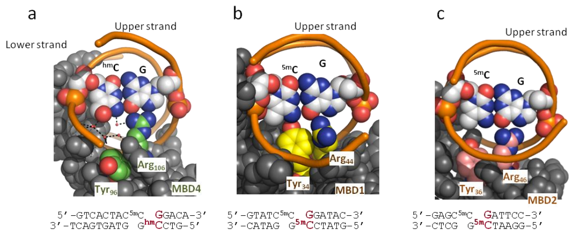
Figure S5. The space filling model representation of the MBD MBD4 - 5mC CG/ hmC CG (a), MBD MBD1 - 5mC CG/ 5mC CG (b) or MBD MBD2 - 5mC CG/ 5mC CG complex structure (c) as shown in figure 3.
