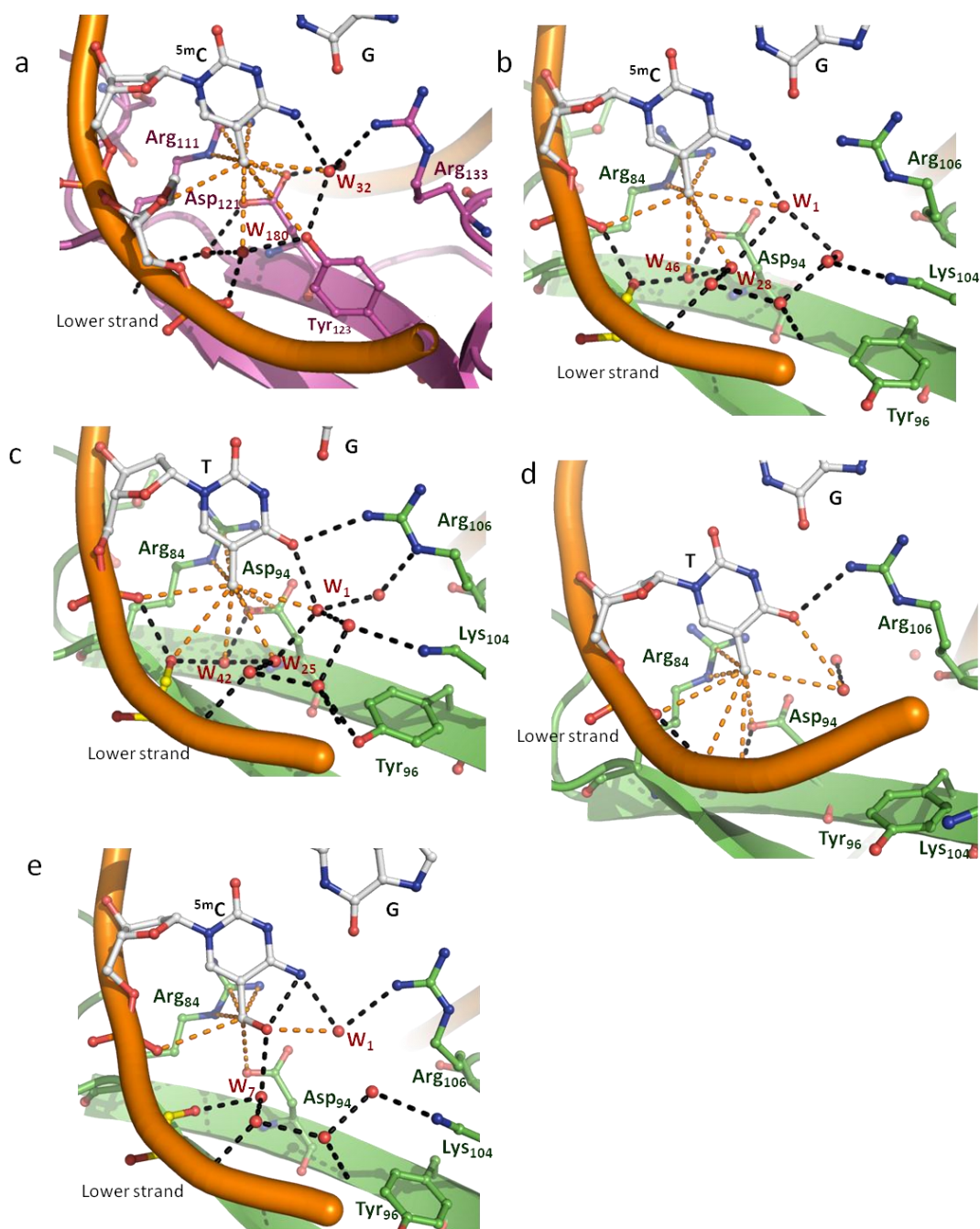
Figure S6. The close up views of the lower strand pyrimidine base recognition in the \text{MBD}_{\text{MeCP2}}\text{-}^{5\text{m}}\text{CG}/^{5\text{m}}\text{CG} complex (a) or \text{MBD}_{\text{MBD4}} in complex with ^{5\text{m}}\text{CG}/^{5\text{m}}\text{CG} (b), 14\text{bp-}^{5\text{m}}\text{CG}/\text{TG} (c), 11\text{bp-}^{5\text{m}}\text{CG}/\text{TG} (d) or ^{5\text{m}}\text{CG}/^{\text{hm}}\text{CG} (e). Hydrogen bonds ( \sim 3.2 Å) and van der Waals contacts or CH-O type hydrogen bonds ( \sim 4.2 Å) are represented in the black and orange dotted lines, respectively.
