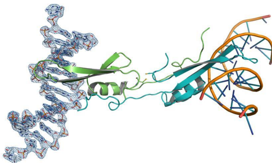
Figure S4. The overall structure of MBD MBD4 complexed with the 14-bp DNA fragment carrying 5m CG/ 5m CG sequence. The blue mesh is the 2mF_O-DF_C electron density map contoured at 1.5 \sigma around the DNA molecule. The C-terminal swapping and a disulphide bond are conserved with the orthorhombic crystal structure of MBD MBD4 - 5m CG/TG complex.
