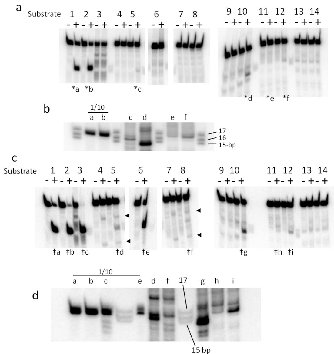
Figure S15. (a) The glycosylase assays toward various DNA sequences (listed in Table S1) using MBD4 as an enzyme. The DNA substrate 1 and 2 yielded significant digestion bands (*a and *b) and 5, 10, 11 and 12 yielded slight digestion bands (*c-*f). (b) Samples *c-*f and 1/10 amounts of samples *a and *b were re-run on the same gel to compare the size of product bands. The 15-, 16- and 17-bp oligo nucleotide fragments were used as DNA size marker. The result implies that MBD4 has significant activity to excise thymine (*a) and hm U (*b) paired with guanine and weak activity toward the
