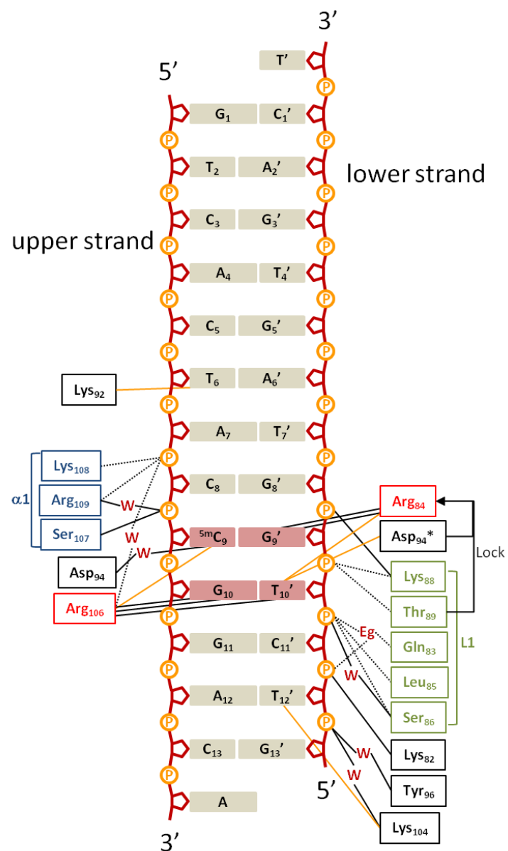
Figure S17. The summary of the interaction between MBD MBD4 and the 14-bp 5m CG/TG fragment.
