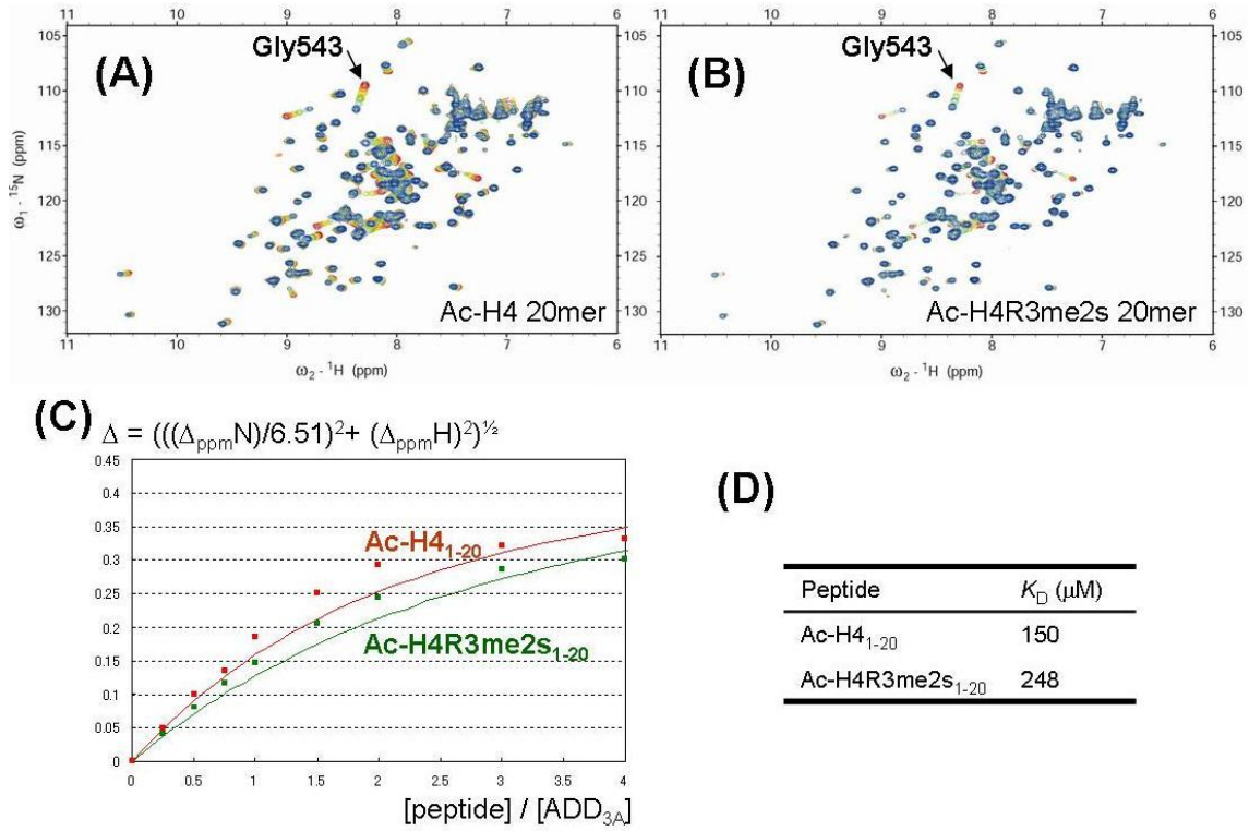
Fig. S2 | Binding experiment with N-terminus acetylated H4 tail without and with symmetrical dimethylation on Arg3 (Ac-H4 and Ac-H4R3me2s) using ^1\text{H} - ^{15}\text{N} correlation spectra. ^{15}\text{N} -labeled ADD 3A at the concentration of 100 \mu\text{M} was titrated by unlabeled Ac-H4 (A) or Ac-H4R3me2s peptide (B) from the peptide stock solutions at the concentration of 1.0 \mu\text{M} . The ^1\text{H} - ^{15}\text{N} correlation spectra were recorded at the peptide to protein ratio of 0, 0.25, 0.5, 0.75, 1.0, 1.5, 2.0, 3.0 and 4.0 (red to blue). Almost identical peak shifts were observed regardless of the methylation status of H4R3. Nonlinear least-square fitting of the gradual peak shift of the backbone amide of Gly543 to the equation,
