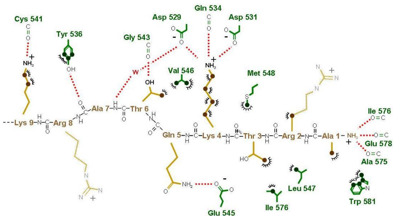
Fig. S4 | Schematic diagram of the ADD 3A :H3-tail interaction. Amino acid residues of ADD 3A involved in the H3-tail interaction are indicated. The main chain hydrogen bonds forming the inter-molecular \beta -sheet are not shown. Hydrogen bonds ( <3.3 Å) between ADD 3A and the H3-tail are shown in red dotted lines, van der Waals contacts ( <4.0 Å) are represented by semicircular arcs. 'W' represents a water molecule.
