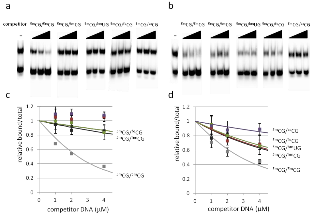
Figure 4. Competitive electrophoretic mobility shift assay. (a, b) The representative autoradiographic images of the competition assay of MBD MBD1 (a) and MBD MBD4 (b). Each of the competitor DNA sequence is indicated above. (c, d) The bound to total ratios are quantified from gel band density and the values relative to the control lanes are plotted against the amount of competitor DNA. Each dots represent the average of three independent experiments using MBD MBD1 (c) or MBD MBD4 (d) with standard deviation. The solid lines represent the fitting curves using the Morrison's equation. The values for the experiment using competitor fragment 5mCG/caCG or 5mCG/hmUG for the MBD MBD1 -5mCG/5mCG complex could not fit to the equation because no competitive effect was observed for these competitor sequences.
