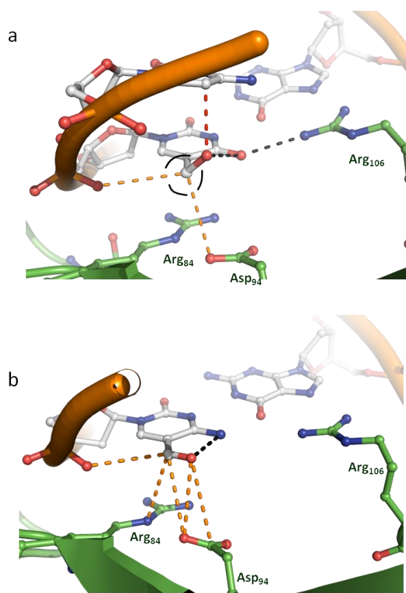
Figure S12. The structural models of the \text{MBD}_{\text{MBD4}}\text{-}^{5\text{m}}\text{CG}/^{\text{hm}}\text{UG} and \text{MBD}_{\text{MBD4}}\text{-}^{5\text{m}}\text{CG}/^{\text{f0}}\text{CG} complexes. (a) The ^{\text{hm}}\text{C} base from the \text{MBD}_{\text{MBD4}}\text{-}^{5\text{m}}\text{CG}/^{\text{hm}}\text{CG} complex is overlaid onto the thymine base of the \text{MBD}_{\text{MBD4}}\text{-}^{5\text{m}}\text{CG}/\text{TG} complex structure. The tetrahedral coordination of the 5-methyl moiety is expected to be conserved. The CH-O type hydrogen bonds donated by the methyl moiety (orange dotted lines), hydrogen bonds (black dotted lines) and a close contact with the 5' neighboring base (red dotted line) are expected. (b) The ^{\text{f0}}\text{C} base from the small molecular crystal is overlaid onto the lower strand ^{5\text{m}}\text{C} base of the \text{MBD}_{\text{MBD4}}\text{-}^{5\text{m}}\text{CG}/^{5\text{m}}\text{CG} complex structure. The intra-base hydrogen bond (black dotted line) of the ^{\text{f0}}\text{C} base is reported in reference 41. The CH-O type hydrogen bonds or van der Waals contacts (orange dotted lines) between the ^{\text{f0}}\text{C} base and Arg84 or Asp94 are expected.
