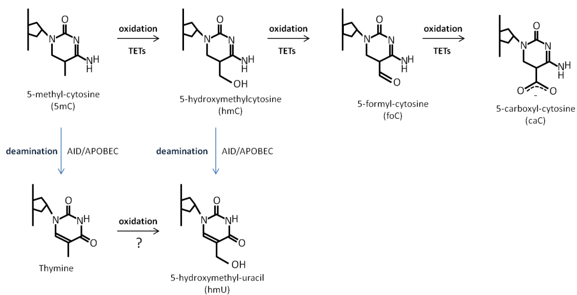
Figure 5. Oxidative modifications of cytosine and thymine.
