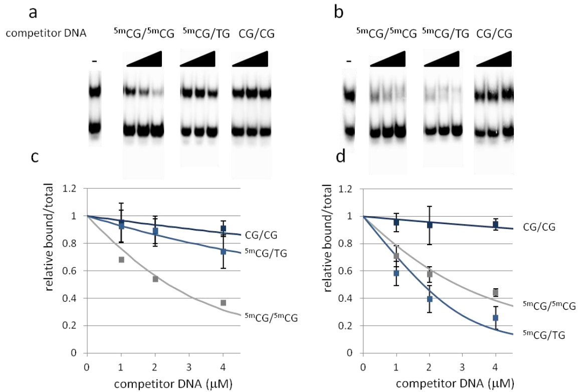
Figure S1. Competitive electrophoretic mobility shift assay. (a, b) The representative autoradiographic images of the competition assay of MBD MBD1 (a) and MBD MBD4 (b). Each of the competitor DNA sequence is indicated above. (c, d) The bound to total ratios are quantified from gel band density and the values relative to the control lanes are plotted against the amount of competitor DNA. Each dots represent the average of three independent experiments using MBD MBD1 (c) or MBD MBD4 (d). The solid lines represent the fitting curves using the Morrison's equation.
