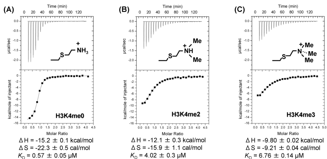
Fig. 2 | Calorimetric study of the binding of ADD 3A to H3 1-19 peptides containing (A) non-, (B) di- or (C) tri-H3K4 methylated analogues. \Delta S , \Delta H and K_D values are means of two experiments using different peptide and protein concentrations.
