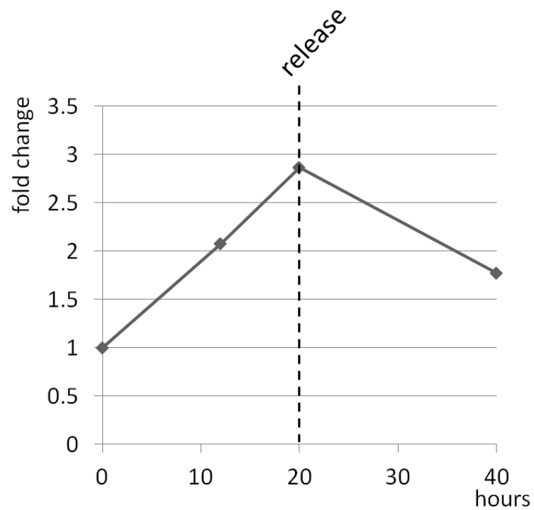
Figure 5. Time course dependent accumulation of hmC bases in the presence of aphidicolin. Fold changes from the control cells (0-hour sample) were plotted as in figure 4. After aphidicolin treatment for 20 hours, the cells were washed and incubated in the normal ES medium for another 20 hours.
