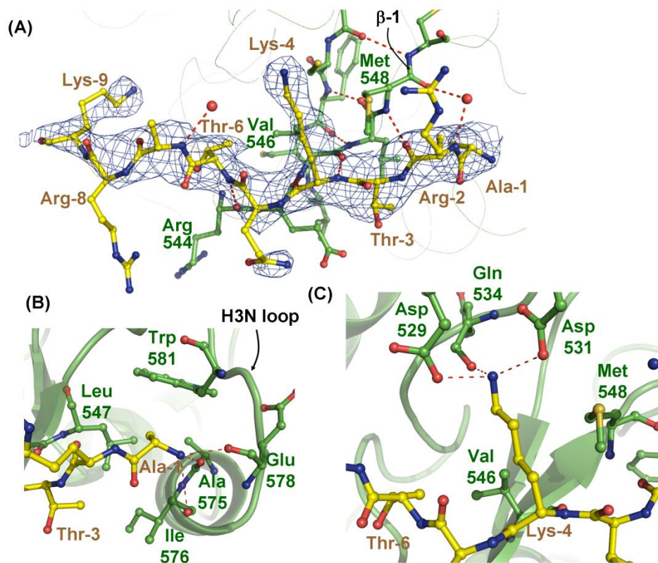
Fig. 3 | Recognition of non-methylated H3K4 by ADD 3A . Red dotted lines indicate hydrogen bonds (<3.3 Å) between H3 and ADD 3A residues. ADD 3A and H3 residues are represented as ball-and-stick models in green and yellow, respectively. (A) H3 peptide is shown with a F_o - F_c omit map contoured at 2.0 \sigma . (B) Close-up view of the recognition of the N-terminus of the H3-tail by ADD 3A . (C) Close-up view of the Lys4 binding pocket of ADD 3A .
