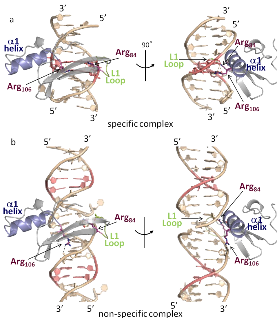
Figure S9. The triclinic crystal structure of MBD MBD4 in complex with 11-bp 5 m CG/TG in the space group of P1. (a) The specific complex binding to the 5 m CG/TG site (colored in red) essentially in the same manner as in the orthorombic crystal. (b) The non-specific complex at the junction of the two symmetry-related DNA fragments. The \alpha 1 helix and the L1 loop are colored in blue and green, respectively. The two arginine side chains are shown as a stick model in purple. The hydrogen bonds and van der Waals interactions which involve Arg 84 or Arg 106 are depicted as black and orange dotted lines, respectively.
