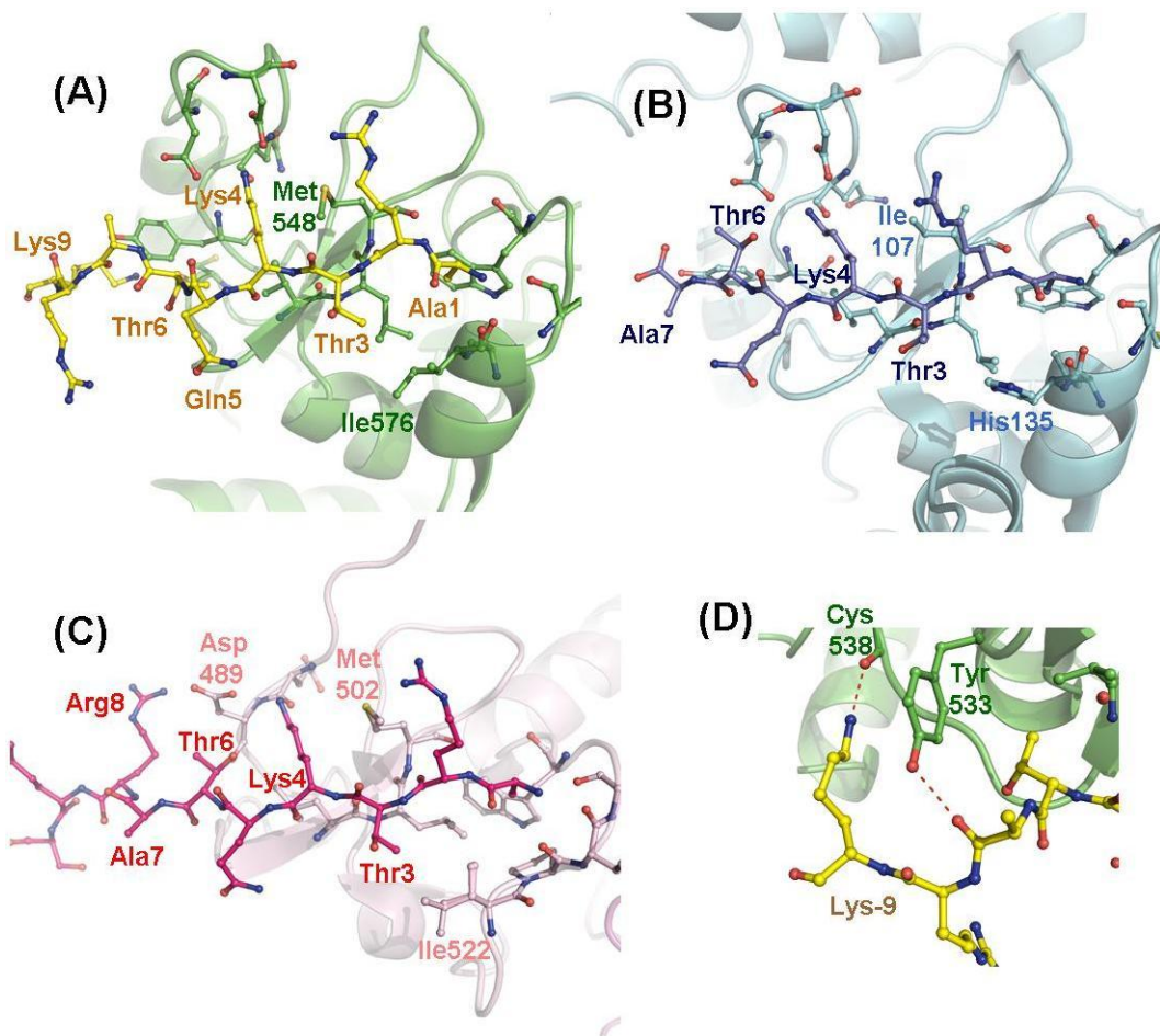
Fig. S3 | Structural comparison between the histone H3 tail bound to ADD 3A (A) , ADD 3L (B) and the PHD of BHC80 (PHD BHC80 ) (C) (PDB code: 3A1B, 2PVC and 2PUY, respectively). The ribbon and stick representation of protein models of ADD 3A , ADD 3L and PHD BHC80 are shown in green, cyan and pink, respectively. The H3 tail peptide bound to these proteins are shown as stick models in yellow, blue and red, respectively. The regions from H3A1 to H3Q5 of the H3 peptide bound to ADD 3A adopts the similar conformation to those bound to ADD 3L and, PHD BHC80 which recognize non-methylated H3K4 (Lan et al , 2007; Ooi et al , 2007), while the conformation of H3 peptide from H3T6 to H3K9 observed in the ADD 3A -H3 complex is slightly deviated from that in the PHD BHC80 -H3 complex. (D) Close-up view of the Lys9 contact site in the ADD 3A -H3 complex structure.
