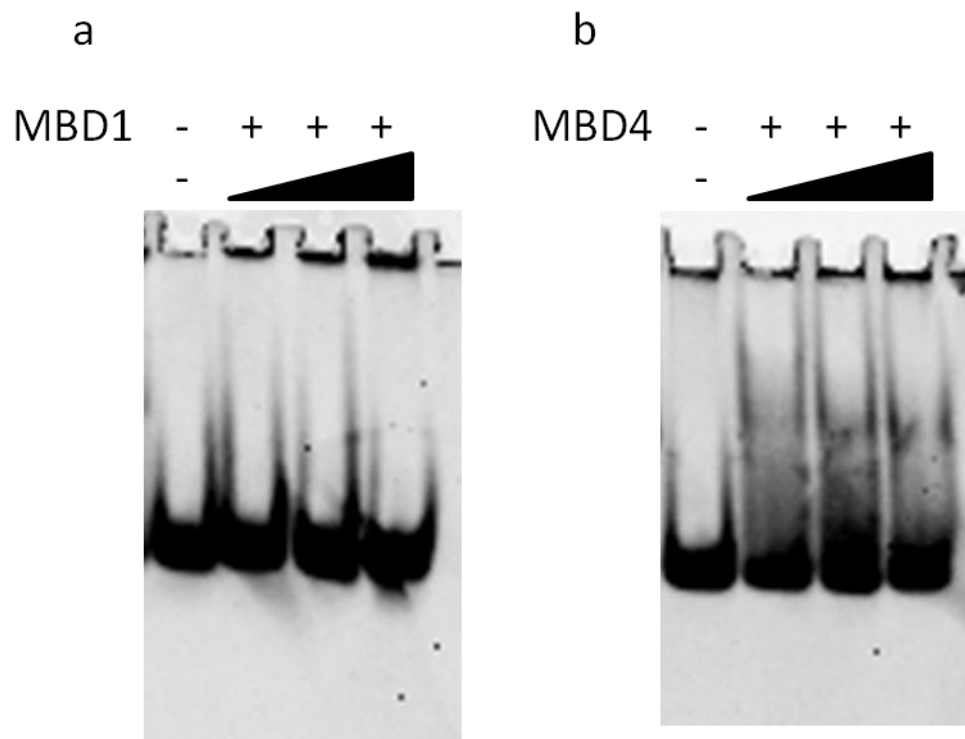
Figure S10. (a, b) Electrophoretic mobility shift assay of MBD1 (a) and MBD4 (b). 1 mM of each MBD domain protein, 3 mM of 14-bp non-modified CpG DNA and 100, 200 or 400 ng of non-specific competitor, poly dI-dC are mixed, incubated for 15 minutes at 4 °C and separated by the 7.5% acrylamide gel electrophoresis followed by GelGreen staining (Cosmo Bio Co. Ltd.).
