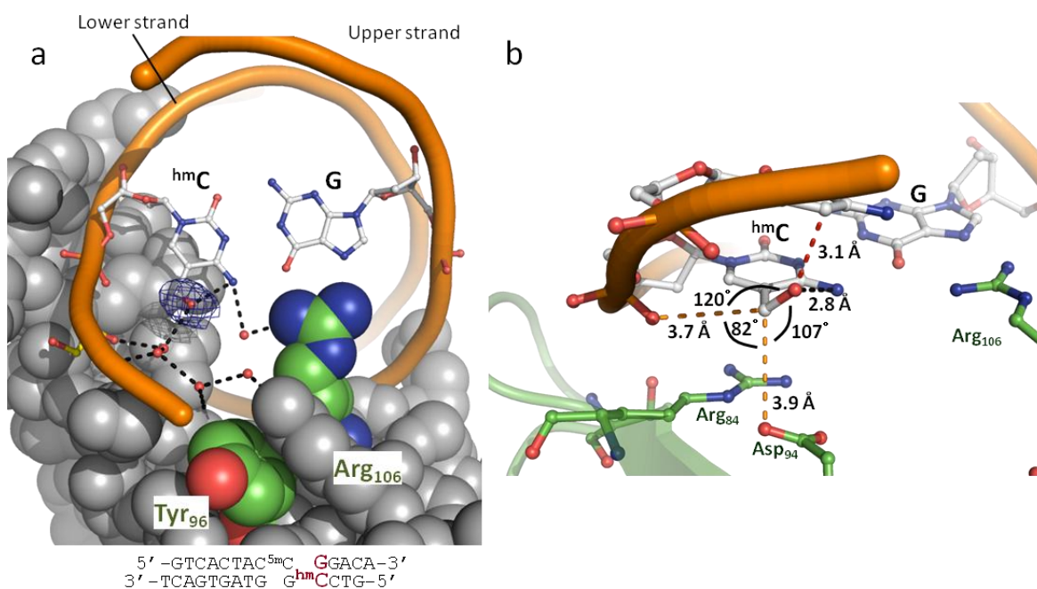
Figure 5. (a) The structure of the MBD MBD4 - 5m CG/ hm CG complex. MBD MBD4 is represented as space filling model. The DNA molecule is shown as ribbon model and the hm C/G base pair is represented as stick model. The blue mesh is the mF O -DF C simulated annealed omit map of the hydroxyl group of the hm C base contoured at 3.0 s. The ethylene glycol molecule is shown in yellow stick model. Water molecules are represented in red small balls. Black dotted lines indicate the hydrogen bonds (~3.2 Å) (b) The tetrahedral configuration around the carbon atom at 5 th position of the cytosine ring. The black, orange or red dotted line represents a hydrogen bond, a CHO type hydrogen bond or an unfavorable close contact.
