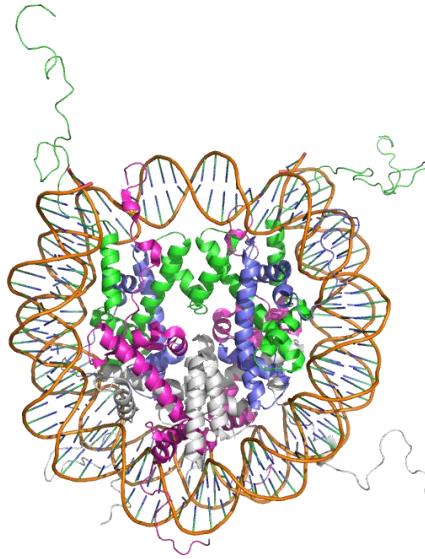
Figure 1. Crystal structure of the nucleosome core particle (PDB code: 1KX5). Two copies of histones H3, H4, H2A and H2B, colored in green, blue, red and white, form octamer wrapped by the 147bp DNA fragment.
