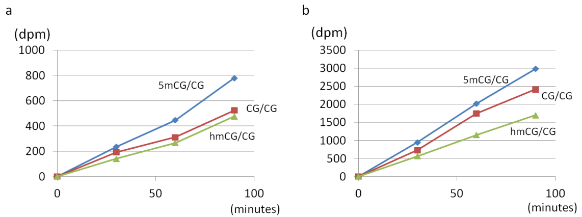
Figure 8. The DNA substrate specificity of de novo DNA methyltransferases, Dnmt3a (a) and Dnmt3b (b). Radio-activities incorporated into the substrate DNA fragments after incubation for 30, 60 and 90 minutes were plotted.
