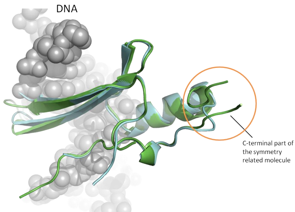
Figure S3. The structural comparison of MBD MBD4 structures with or without C-terminal swapping. The MBD MBD4 molecule in the P1 crystal (without swapping), shown in blue ribbon model, is overlaid onto the green ribbon model of the MBD MBD4 molecule in the C222 1 crystal (with swapping). The exchange of peptide chain occurs at the loop between Asn118 and Leu124. The structural perturbation because of the swapping artifact can be seen at the limited region on the other side of the DNA binding interface (orange circle).
