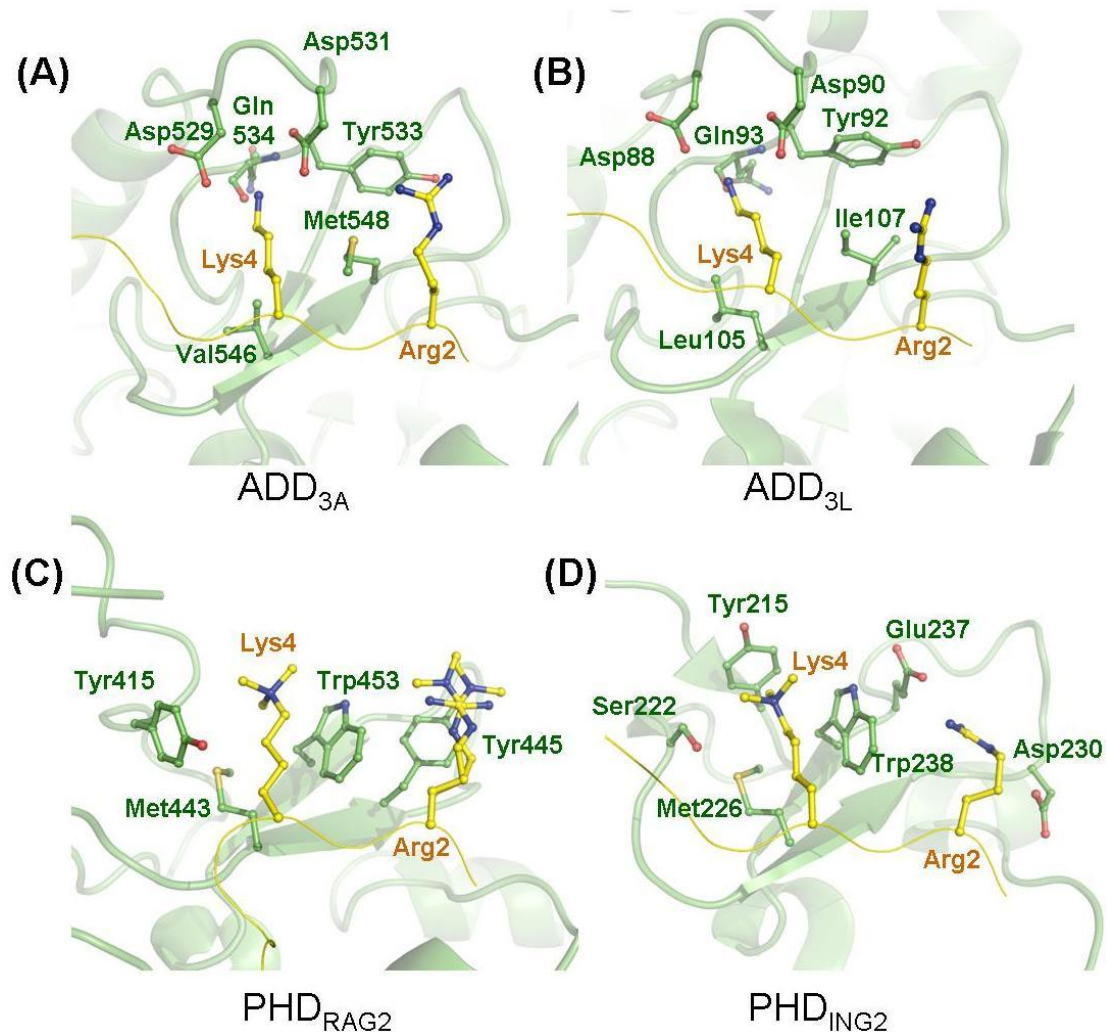
Fig. S8 | H3R2 binding pockets of PHD fingers. In the structure of ADD 3A -H3 complex (A) , the side chain of H3R2 is fully exposed to the solvent as is observed in the structure of DNMT3L-H3 complex (B) , PDB code: 2PVC) and the methylation on this residue seems not to affect the interaction between ADD 3A and H3 tail. The PHD finger of RAG2 was reported to bind to the H3 tail carrying both methylated H3R2 and H3K4 with slightly higher affinity than to the tail carrying only methylated H3K4 (Ramón-Maiques et al , 2007). In the structure of PHD RAG2 complexed with methylated H3R2 (C) , PDB code: 2V86), methylated side chain of H3R2 stacks with aromatic side chain of Tyr445. In contrast, it was proposed that the methylation of H3R2 generally
