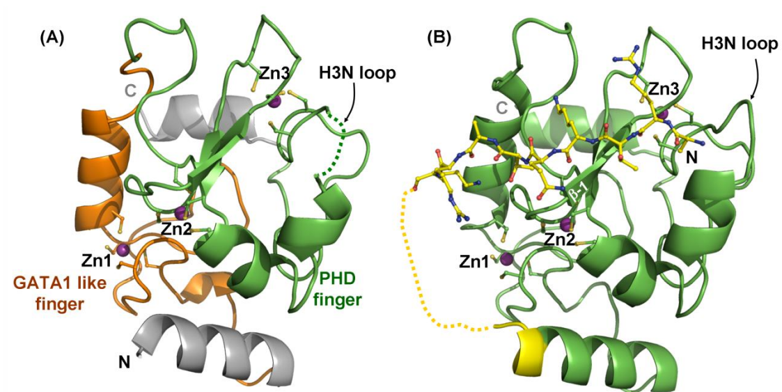
Fig. 1 | Overall structures of ADD 3A in the unliganded and H3-bound forms. (A) Ribbon representation of the unliganded ADD 3A . Three zinc ions and cysteine residues forming CxxC motifs are shown as magenta spheres and stick models, respectively. GATA-1-like and PHD fingers are shown in orange and green, respectively. The green dotted line represents the disordered H3N loop. (B) Crystal structure of ADD 3A (green) bound to the H3-tail (yellow). H3-peptide (residues 1-9) is shown as a ball-and-stick model. The disordered linker peptide that connects the C-terminus of the peptide and the N-terminus of ADD 3A is represented by a yellow dotted line. The H3N loop is shown in red.
