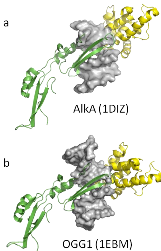
Figure S13. The ternary complex model based on the crystal structures of AlkA complexed with product DNA (a, PDB ID; 1DIZ) and OGG1 complexed with the substrate DNA (b, PDB ID; 1EBM). There are apparent steric clashes between the bent DNA molecules and MBD domain.
