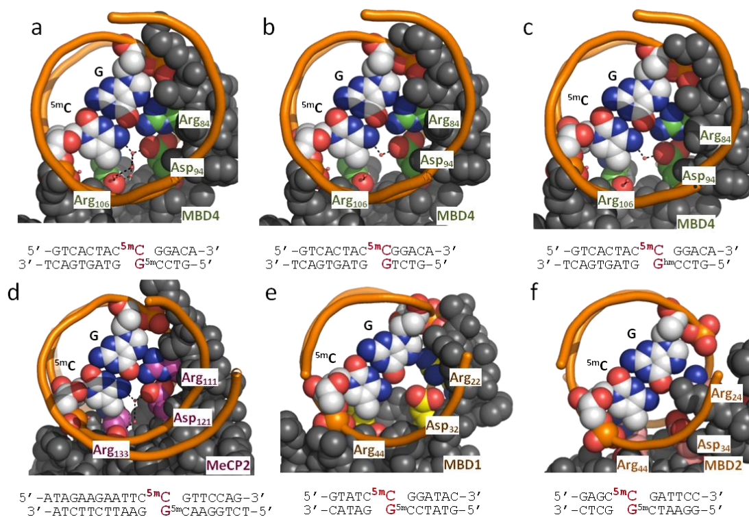
Figure S8. The space filling model representation of the MBD MBD4 - 5mC CG/ 5mC CG (a), MBD MBD4 - 5mC CG/TG (b), MBD MBD4 - 5mC CG/ hmC CG (c), MBD MeCP2 - 5mC CG/ 5mC CG (d), MBD MBD1 - 5mC CG/ 5mC CG (e) or MBD MBD2 - 5mC CG/ 5mC CG complex structure (f) viewed from the opposed angle of that of figure 3 and supplementary figure S4. The upper strand 5mC C recognition mode is conserved among all structurally known MBD domain proteins.
