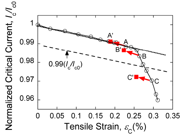
Fig.6. Change in I_c/I_{c0} with strain \varepsilon_c in loading-unloading process in a specimen without copper. A, B and C refer to the start of unloading, and A', B' and C' refer to the end of unloading around by 0.04% from A, B and C, respectively.
