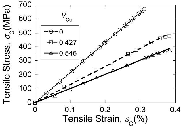
Fig. 3. Measured tensile stress \sigma_C - strain \varepsilon_C relation at 77 K of the specimens with V_{Cu}=0, 0.427 and 0.546 .
