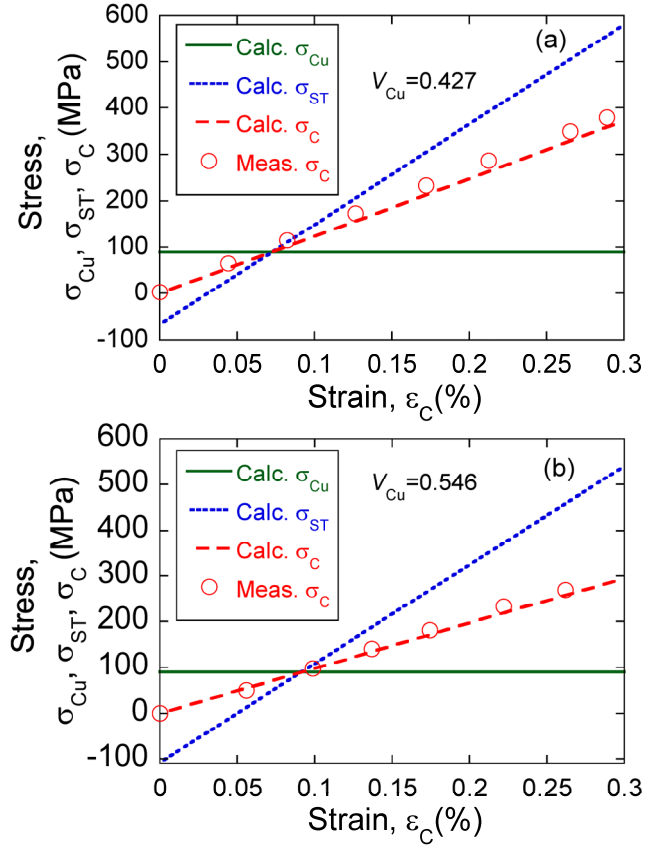
Fig. 5. Calculated stress ( \sigma_{ST} ) of the substrate tape and stress ( \sigma_{Cu} ) of copper, stress ( \sigma_C ) of the composite tape as a function of strain ( \varepsilon_C ) of the composite, together with the measured \sigma_C - \varepsilon_C relation for comparison with calculated one. (a) V_{Cu}=0.427 . (b) V_{Cu}=0.546 .
