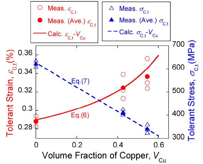
Fig. 9. Measured tolerant strain \varepsilon_{C,t} and tolerant stress \sigma_{C,t} plotted against volume fraction of copper ( V_{Cu} ). The solid curve and broken line refer to the analyzed \varepsilon_{C,t} - V_{Cu} and \sigma_{C,t} - V_{Cu} relation, respectively.
