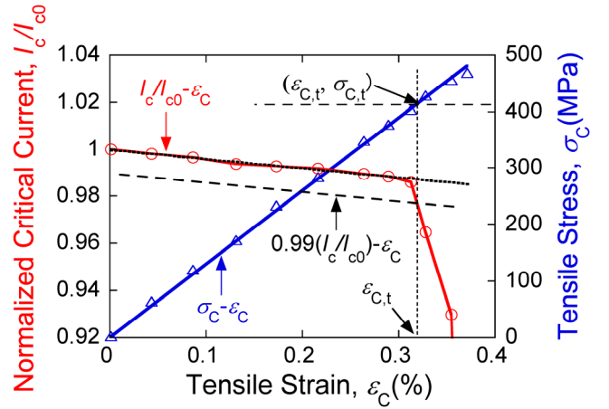
Fig. 8. An example of determination of \varepsilon_{C,t} and \sigma_{C,t} from the measured I_c/I_{c0} - \varepsilon_C and \sigma_C - \varepsilon_C relations.
