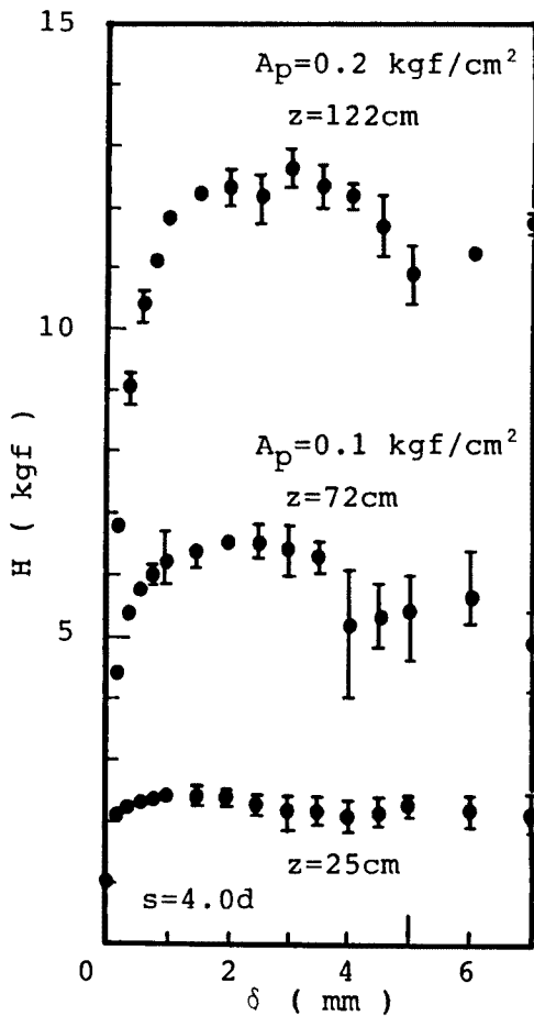
Fig. 16. H \sim \delta curves and data scattering condition. ( s = 4.0 \text{ d} ).
