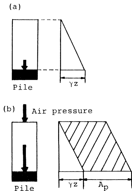
Fig. 14. Load acting on pile by using loading apparatus controlled by air pressure.
