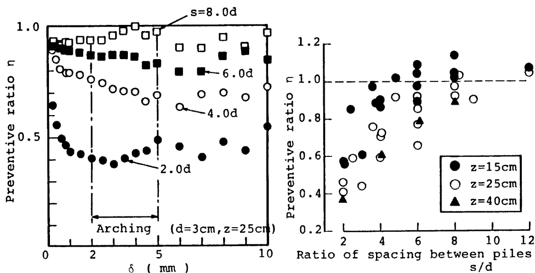
Fig. 8. Preventive ratio \eta ( d=3\text{ cm} , z=25\text{ cm} ). Fig. 9. Relationship between preventive ratio ( \eta ) and ratio of spacing between piles ( s/d ).
