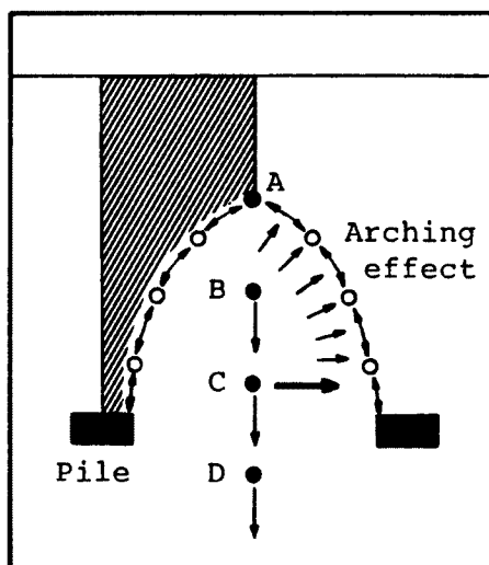
Fig. 4. Arching effect in front of piles.
