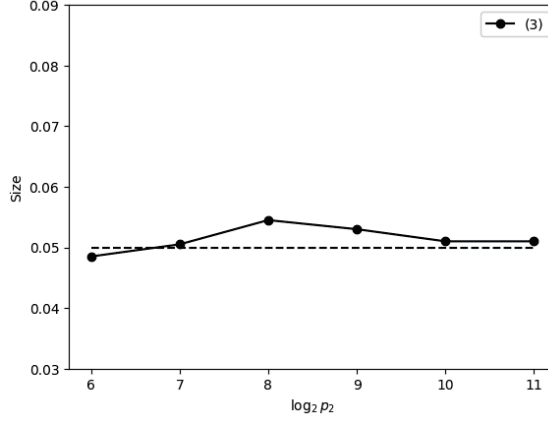
図 1 (I) \mathbf{x}_j \sim N_p(\mathbf{0}, \Sigma)
