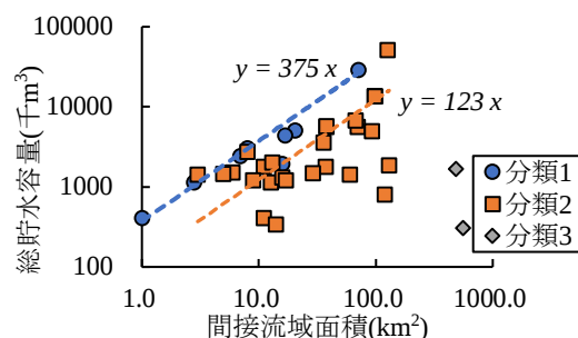
Fig. 2 Relation between indirect catchment area and capacity
