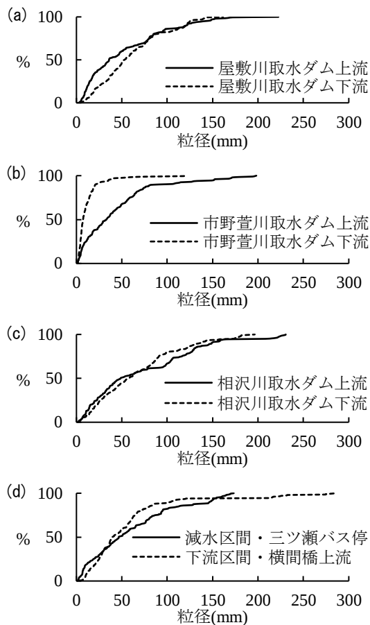
Fig. 6 Grain size accumulation curve, (a) Yashikigawa, (b) Ichinokayagawa, (c) Aizawagawa, (d) main channel
