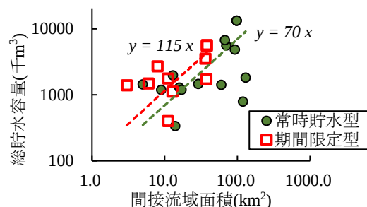
Fig. 3 Relation between indirect catchment area and capacity in class 2
