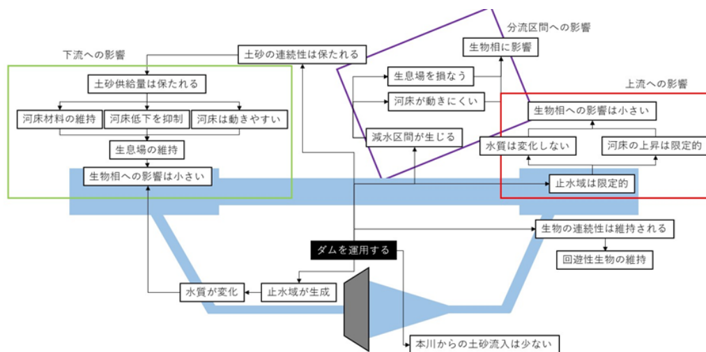
Fig. 4 Impact response flow of off-stream dam
